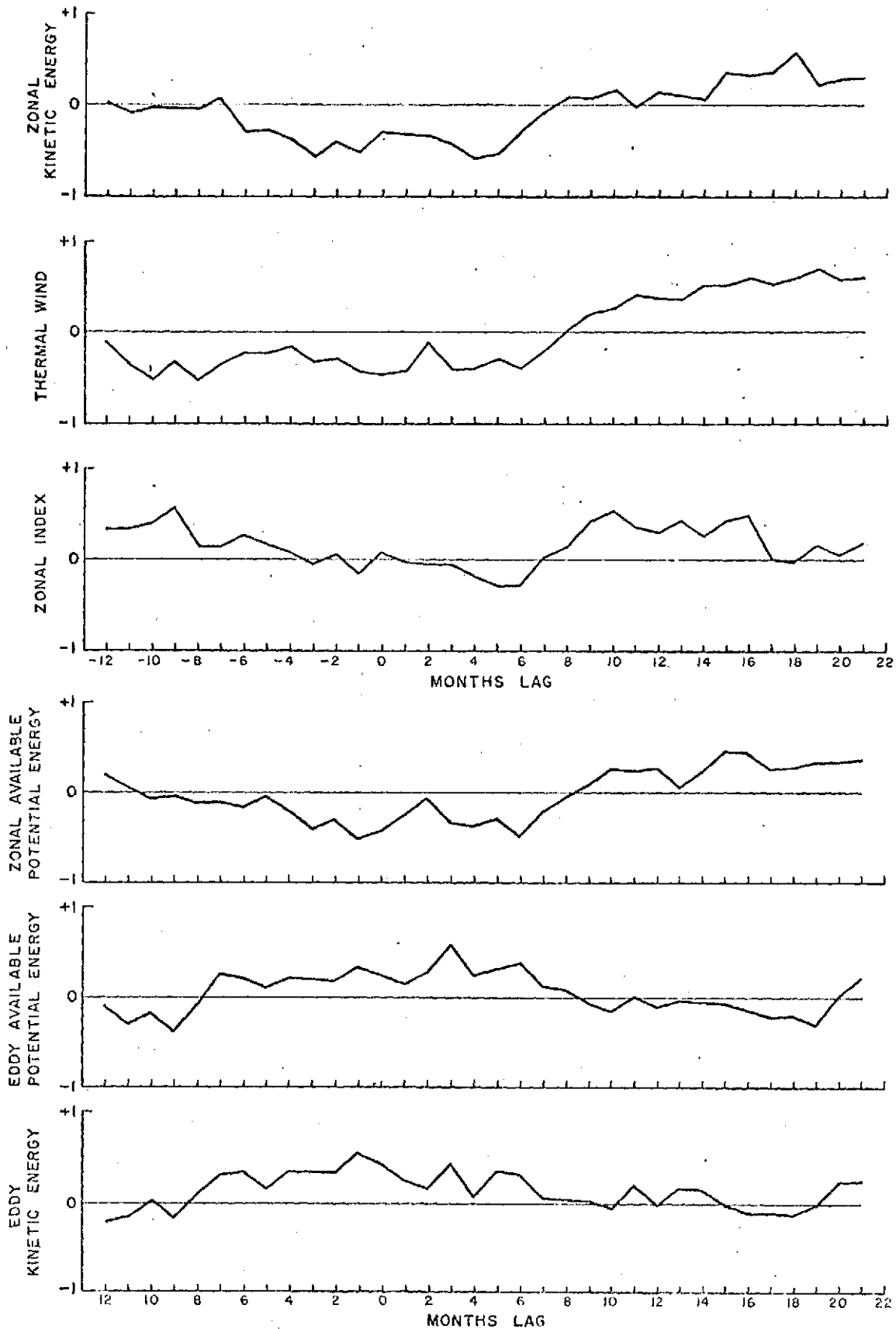
Figure 3. Lag correlation coefficients between interannual variations in general circulation parameters ( GP' ) and north-south gradient of infrared radiant exitance ( \Delta RL' ); - months (+ months) for GP' leading (lagging) \Delta RL' .
