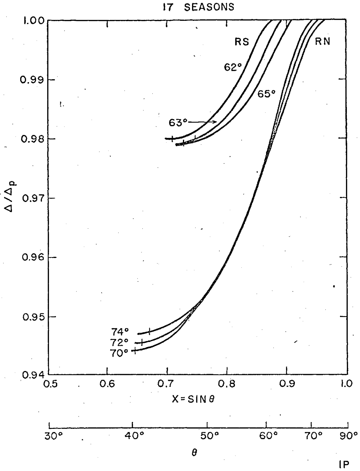
Figure 2. Budyko-Leith climate model generated ice-snow boundary latitudes for various reductions in the solar constant ( \Delta/\Delta p ) using 17 seasons satellite data. Vertical hacks indicate latitude for model instability RN: northern hemisphere, RS: southern hemisphere.
