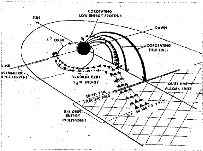
Figure 1. General flow patterns of protons.
