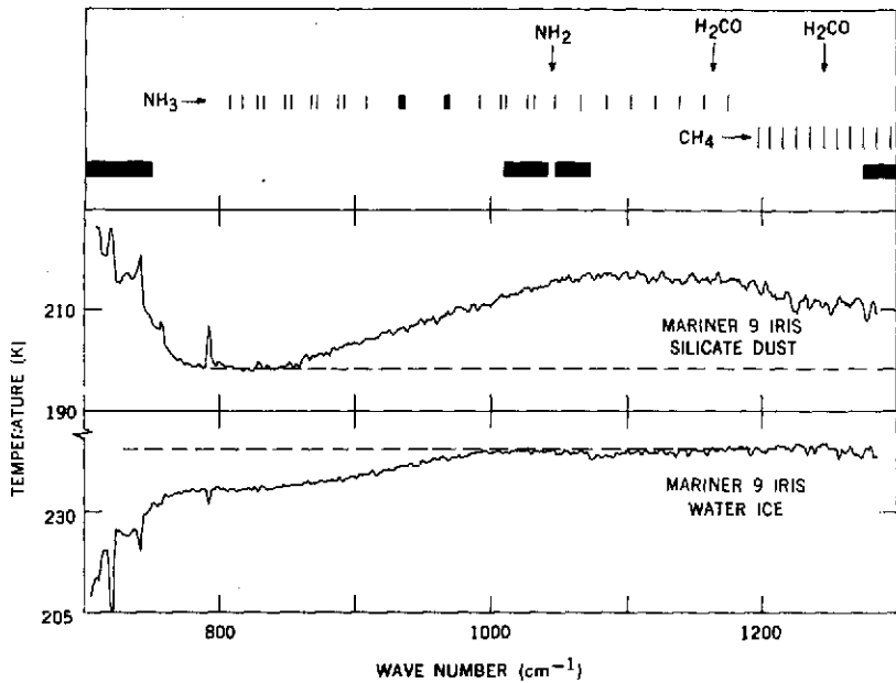
Figure 1. Cometary composition schematic, 10- \mu\text{m} region.
