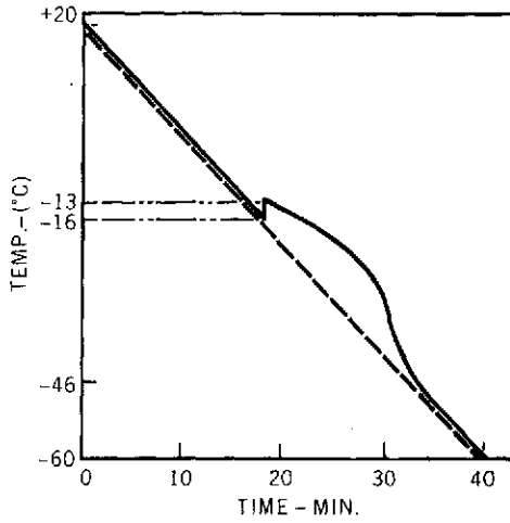
Figure 1. Temperature of the blood as a function of time during the freezing process.
