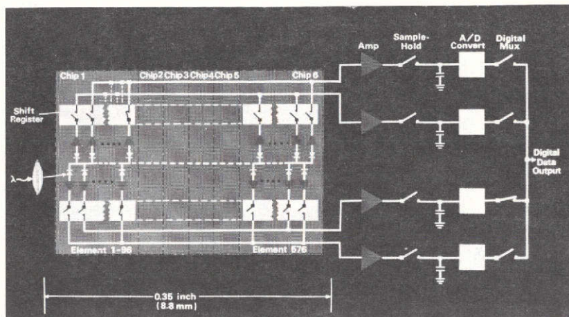
Figure 2. Solid-state linear array imager.
