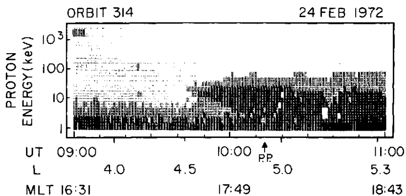
Figure 2. Energy spectrogram taken at the beginning of a magnetic storm main phase.
