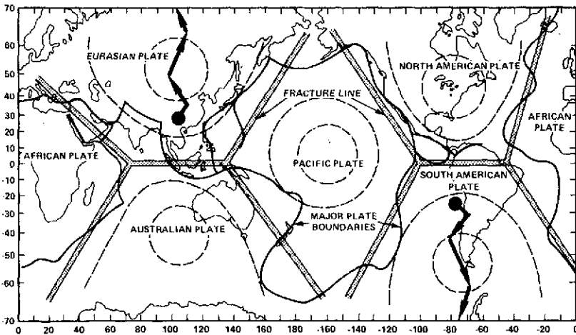
Figure 4. Fracture lines for a shift of the poles over 70^\circ along the meridian of 75^\circ\text{W} .
