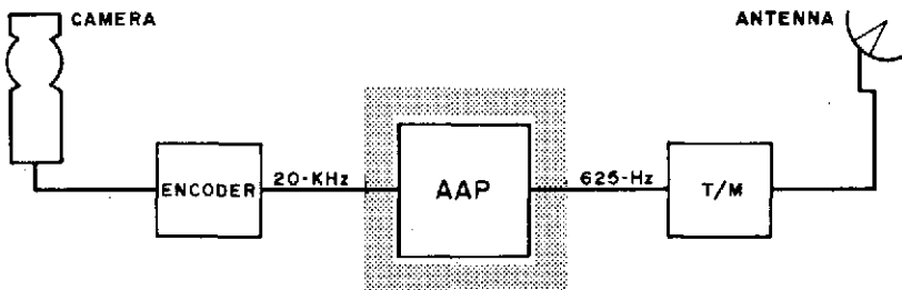
Figure 1. Antenna aspect subsystem for the RAE-B spacecraft.
