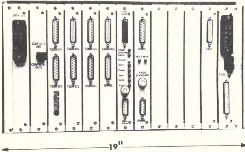
Figure 5. Equipment needed at each end of the demand assigned voice communications system.
