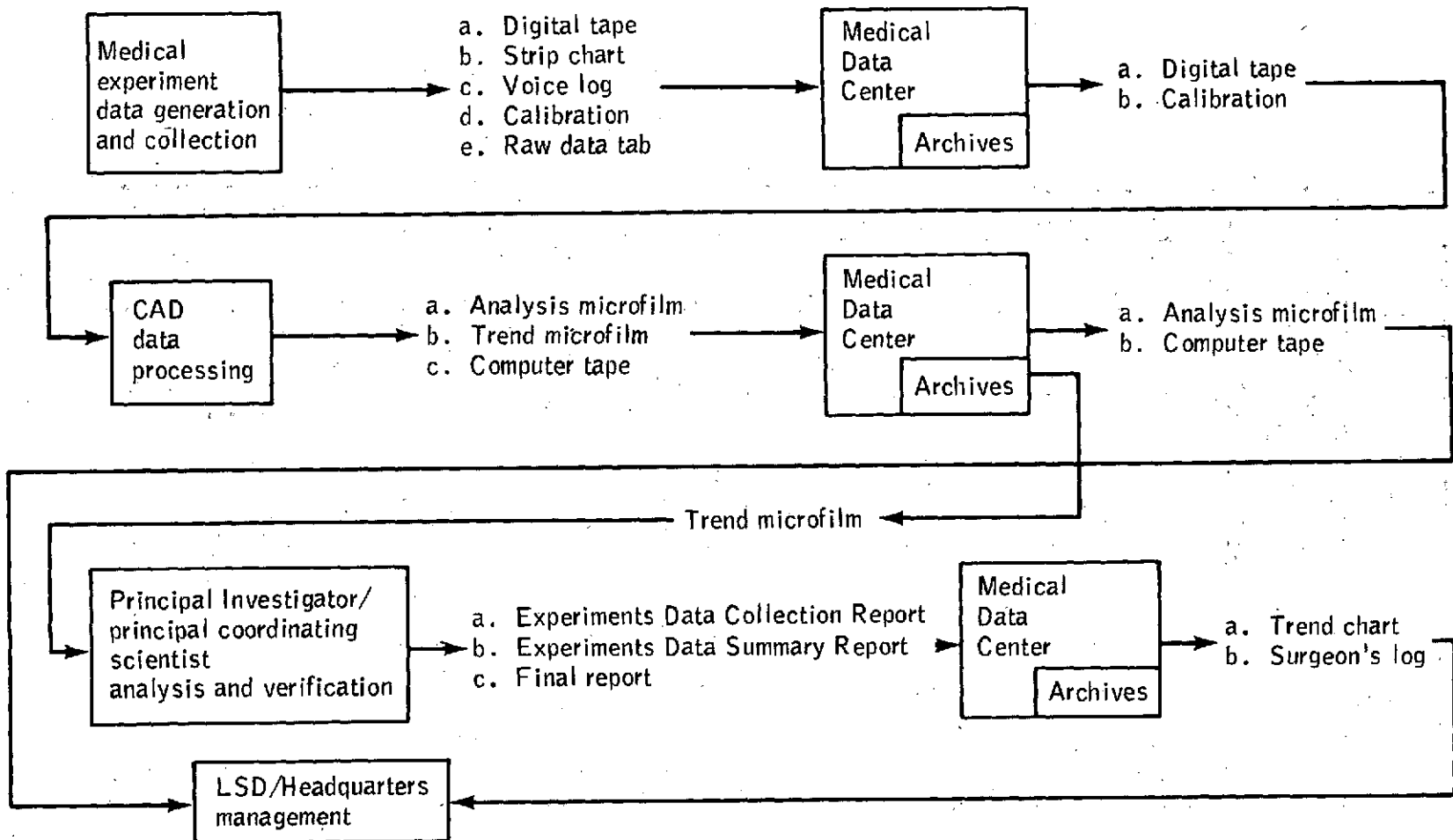
Figure 3.- Typical data flow during each Skylab mission.
