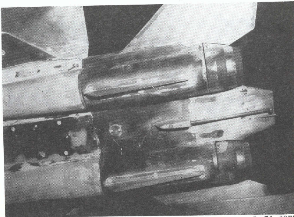
(b) Bottom rear view of nozzle type A, maximum afterburning power setting, with basic interfairing.
