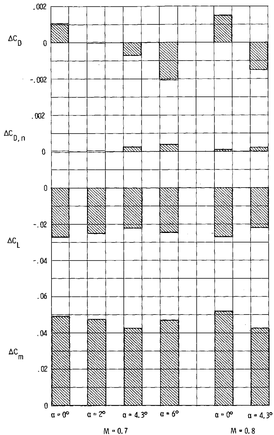
Figure 39.- Increments in afterbody-nozzle aerodynamic characteristics due to deflecting horizontal tails from 0° to -2° with type A cruise nozzles and interfering 2.
