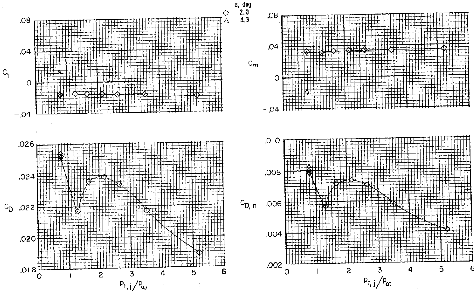
Figure 16.- Effect of jet total-pressure ratio on afterbody-nozzle aerodynamic forces and moments for type A maximum afterburning nozzles and interfering 6 at M = 1.20 .
