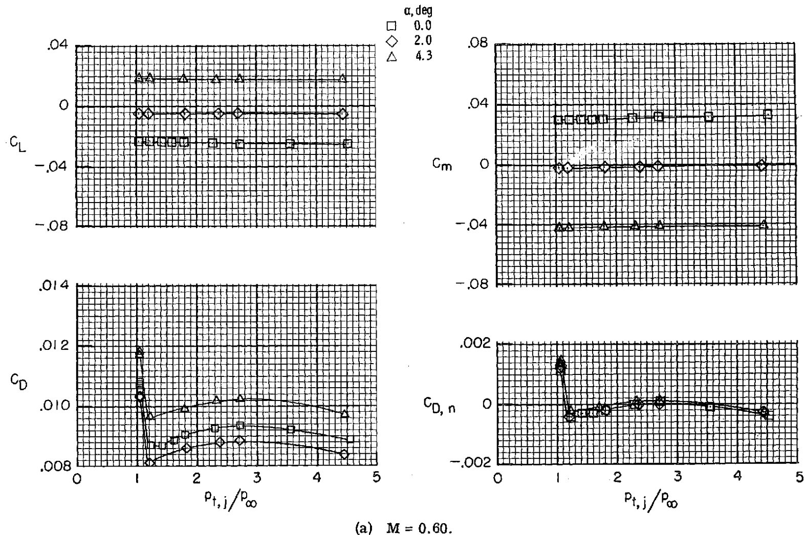
Figure 20.- Effect of jet total-pressure ratio on afterbody-nozzle aerodynamic forces and moments for type B cruise nozzles and interfairing 4.
