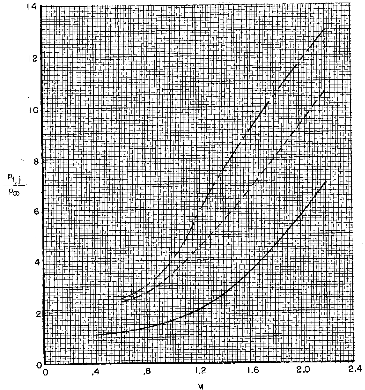
Figure 29.- Typical schedules of aerodynamic model flow-through and engine total-pressure ratios.
