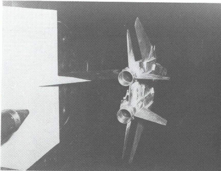
(t) Rear view of nozzle type B, supersonic maximum afterburning power setting, with interfairing 2 in 4-foot tunnel; model mounted on side wall.
