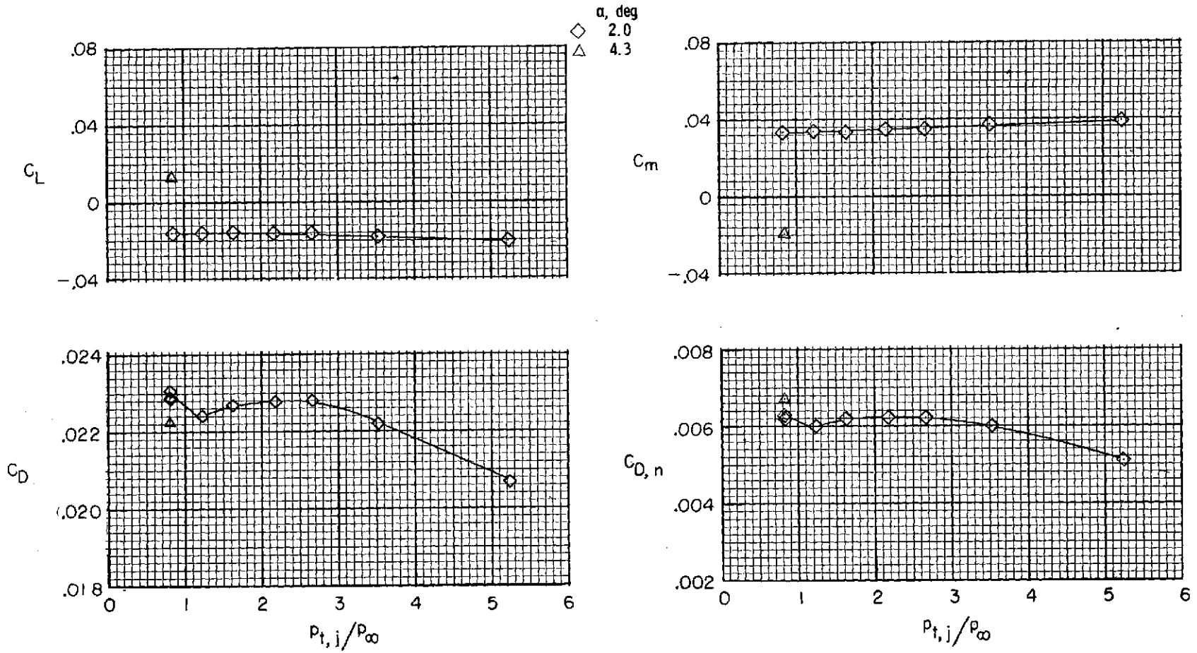
Figure 27.- Effect of jet total-pressure ratio on afterbody-nozzle aerodynamic forces and moments for type B transonic maximum afterburning nozzles and interfering 6 at M = 1.20 .
