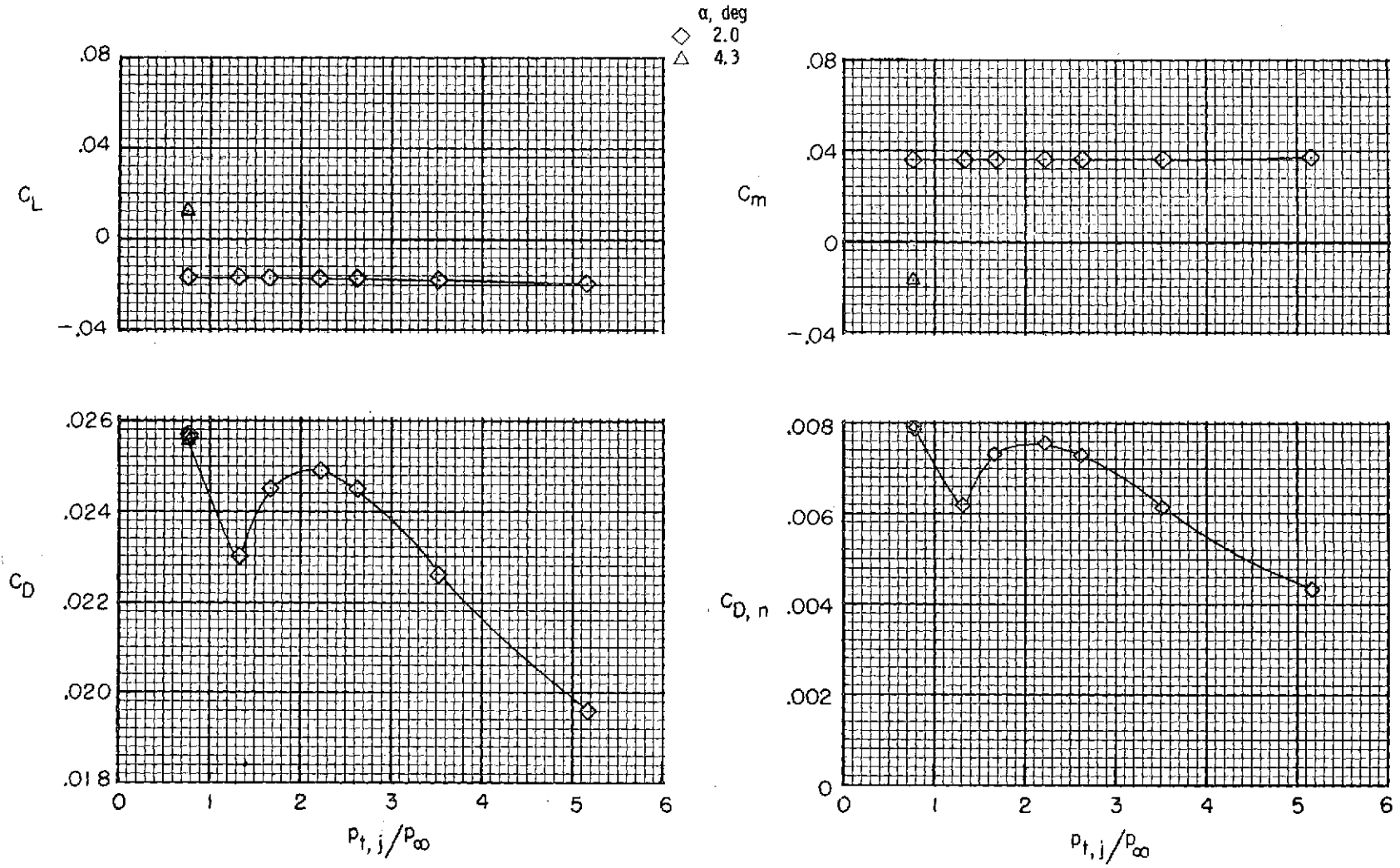
Figure 15.- Effect of jet total-pressure ratio on afterbody-nozzle aerodynamic forces and moments for type A maximum afterburning nozzles and interfairing 4 at M = 1.20 .
