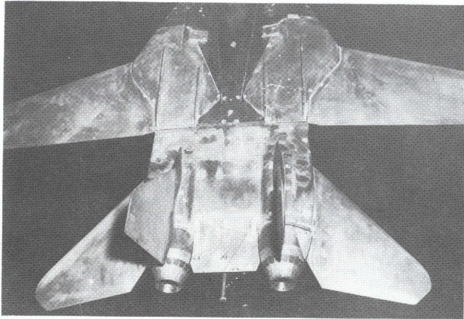
(c) Top rear view of nozzle type A, cruise power setting, with typical short wedge interfairing.
