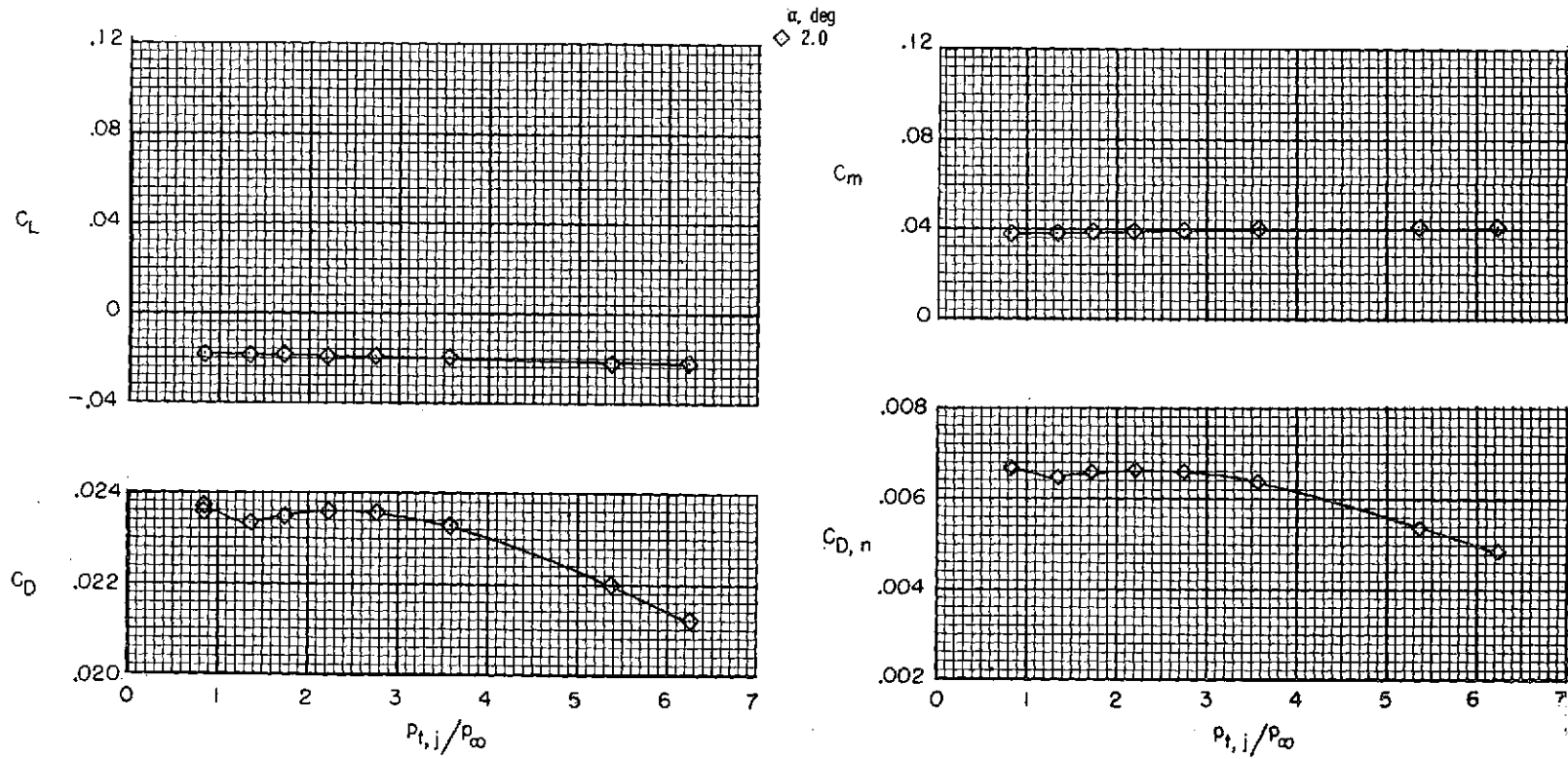
Figure 26.- Effect of jet total-pressure ratio on afterbody-nozzle aerodynamic forces and moments for type B transonic maximum afterburning nozzles and interfering 4 at M = 1.20 .
