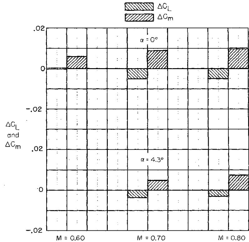
(b) Afterbody-nozzle lift and pitching moment.
