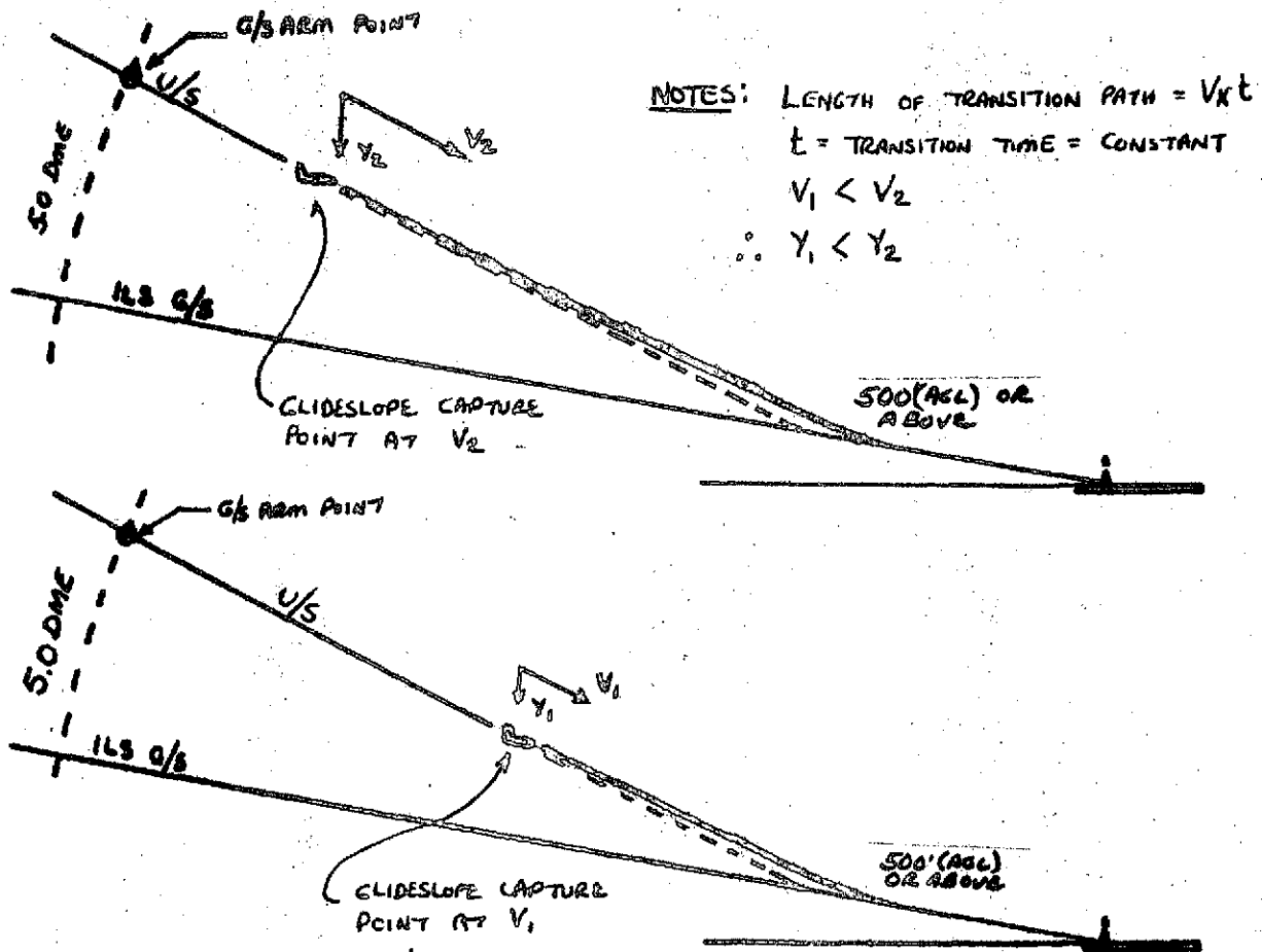
FIGURE 1 - GLIDESLOPE CAPTURE POINT - AS FUNCTION OF APPROACH SPEED.
