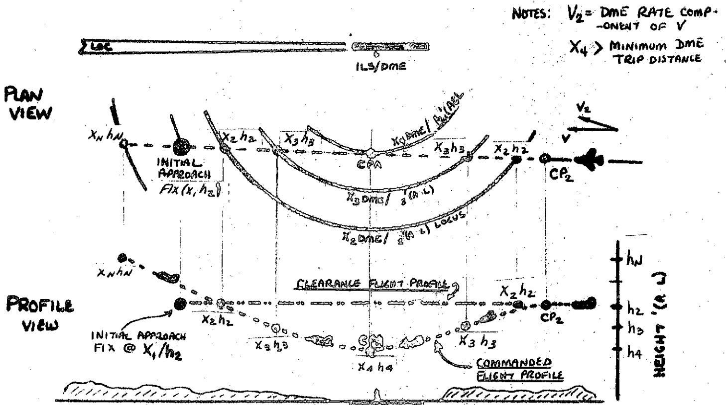
FIGURE 2 - UPPER SEGMENT PROFILE - AREA TRANSIT CASE (Two-segment system armed and valid - F/D and A/P in auto modes)
