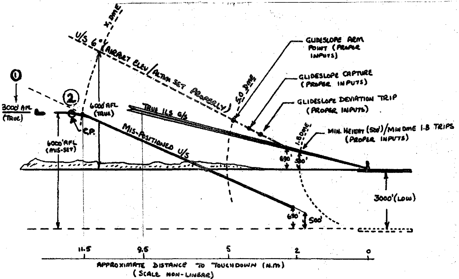
FIGURE 6 - EFFECT UPON FAIL GLIDESLOPE CAPTURE PROTECTORS OF AIRPORT ELEVATION MIS-SET LOW (ALTIMETER BARO-CORRECTION MIS-SET HIGH)
