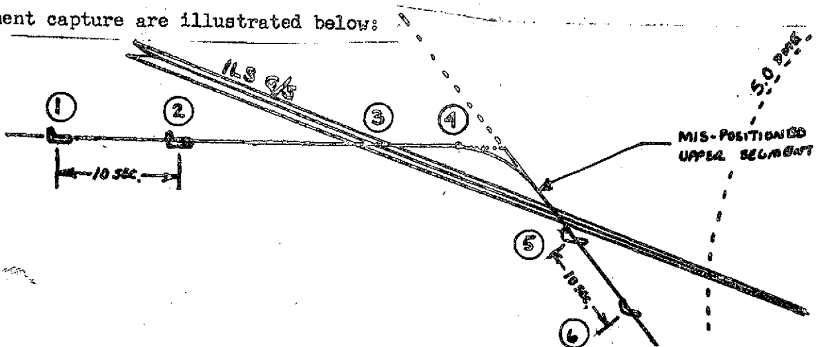
FIGURE 7 - BELOW-TO-ABOVE GLIDESLOPE PRIOR TO UPPER SEGMENT CAPTURE CASES
