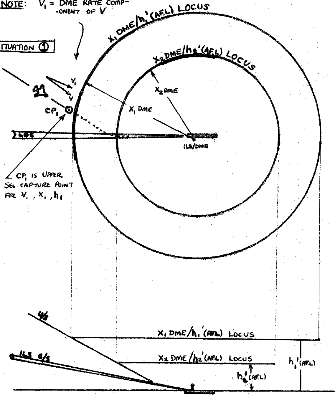
FIGURE 1 - UPPER SEGMENT CAPTURE AS FUNCTION OF HEIGHT ABOVE FIELD ('AFL) AND DME
