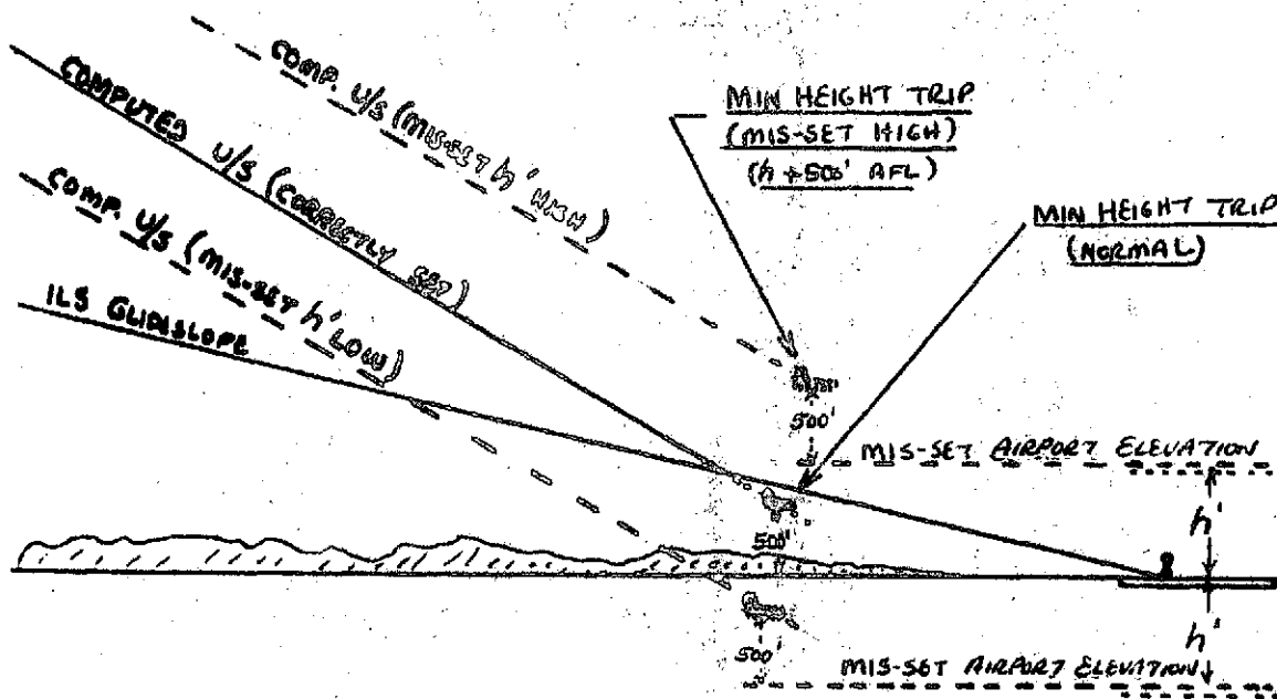
FIGURE 4 - HEIGHT ABOVE FIELD TRIP (INCLUDING AIRPORT ELEVATION MIS-SET HIGH AND LOW)
