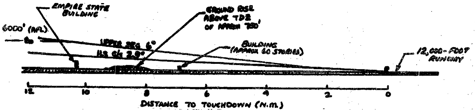
2-SEGMENT PROFILE (APPROXIMATELY TO SCALE)
