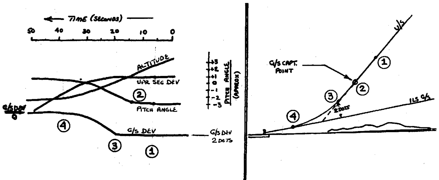
FIGURE 3 - GLIDESLOPE TRANSITION OSCILLOGRAPH DATA RELATED TO AIRCRAFT POSITION IN PROFILE
