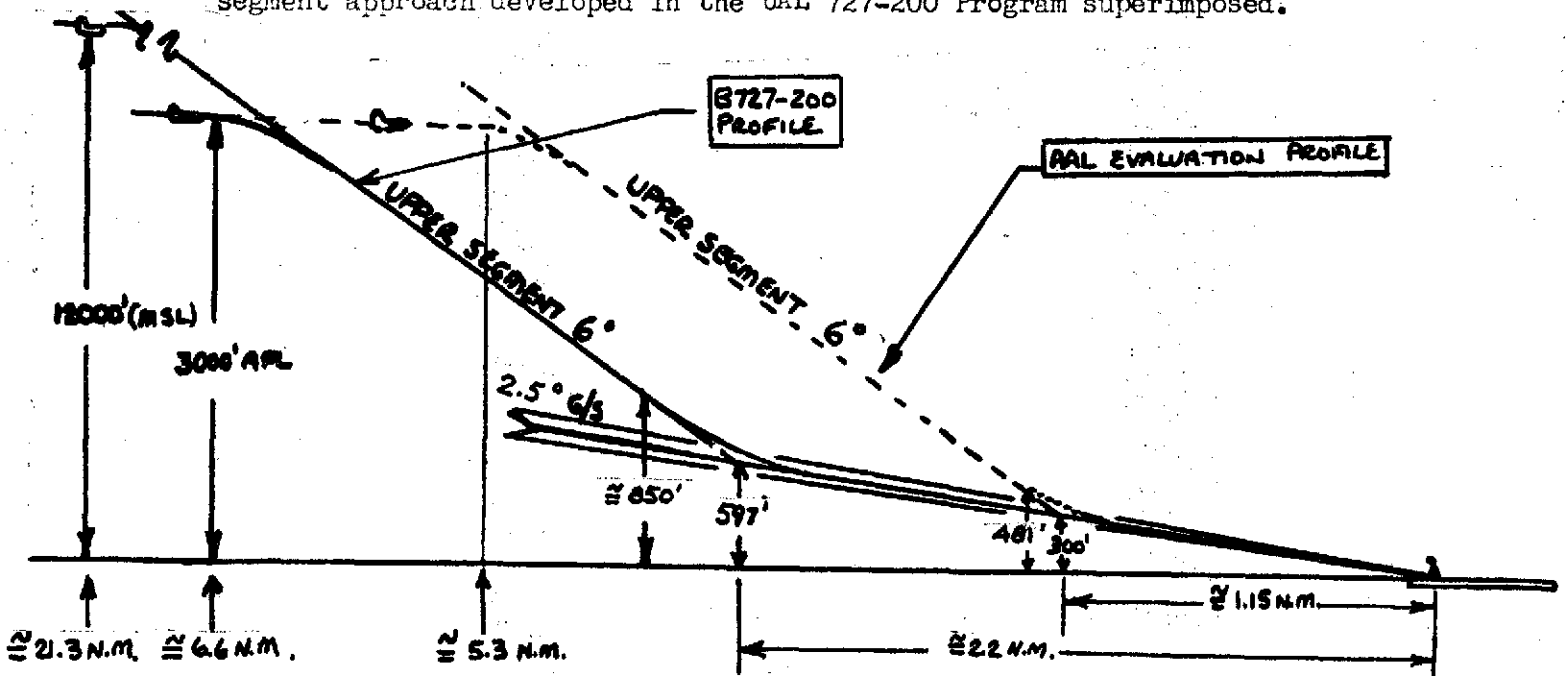
FIGURE 3 - COMPARISON BETWEEN AA 720-023B AND UAL 727-222 FLIGHT SIMULATOR 2-SEGMENT PROFILES.
