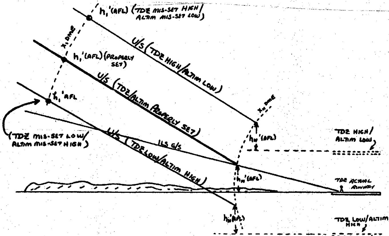
FIGURE 2 - EFFECT OF ERRONEOUS TDZ ELEVATION OR ERRONEOUS ALTIMETER CORRECTION INPUT UPON ACTUAL POSITION OF COMPUTED UPPER SEGMENT.
