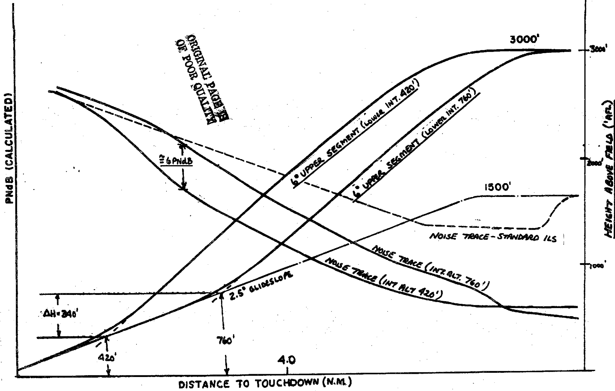
FIGURE 5 - EFFECT OF LOWER INTERSECT ALTITUDE
