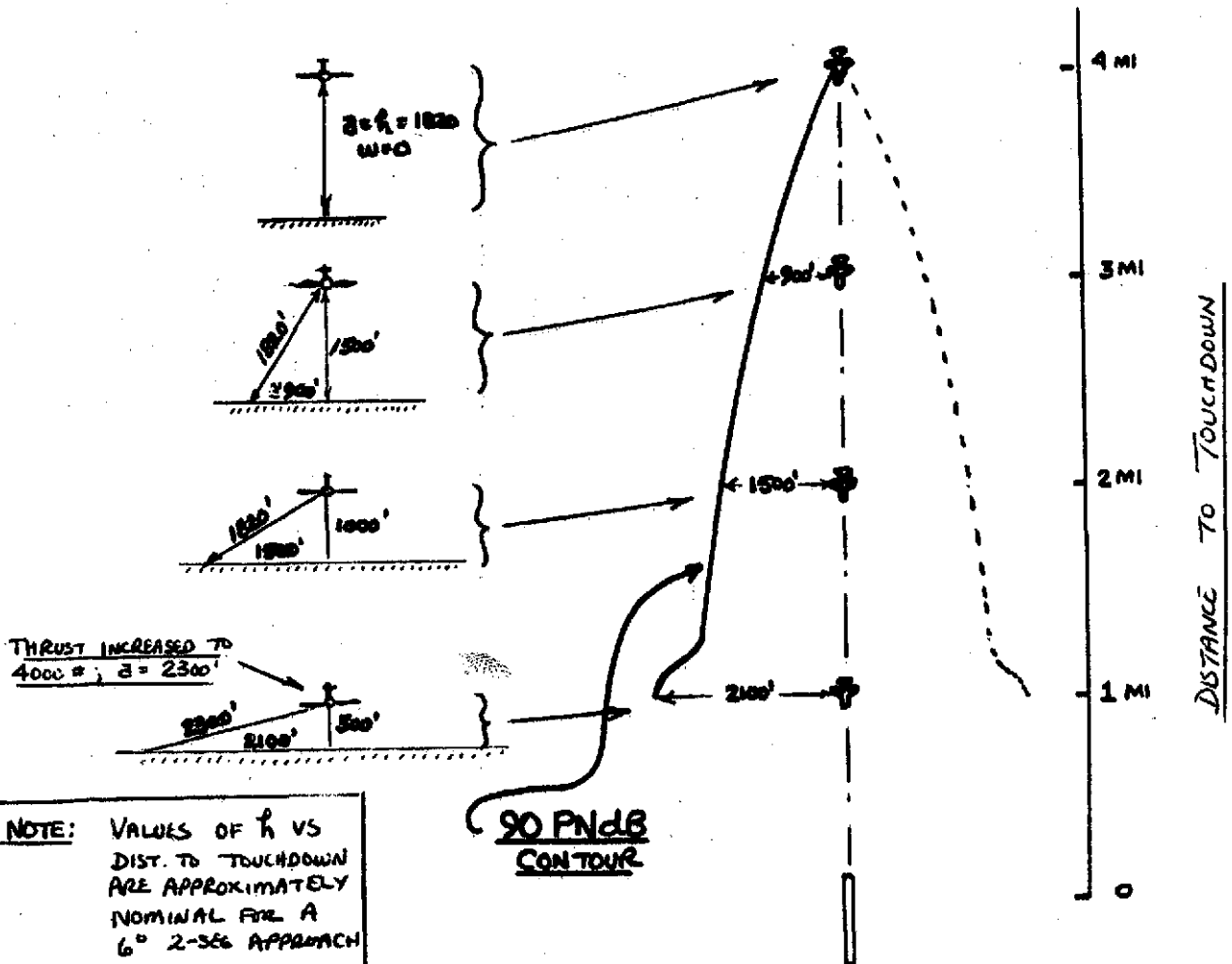
FIGURE 5- 90 PNdB CONTOUR COMPUTATION
