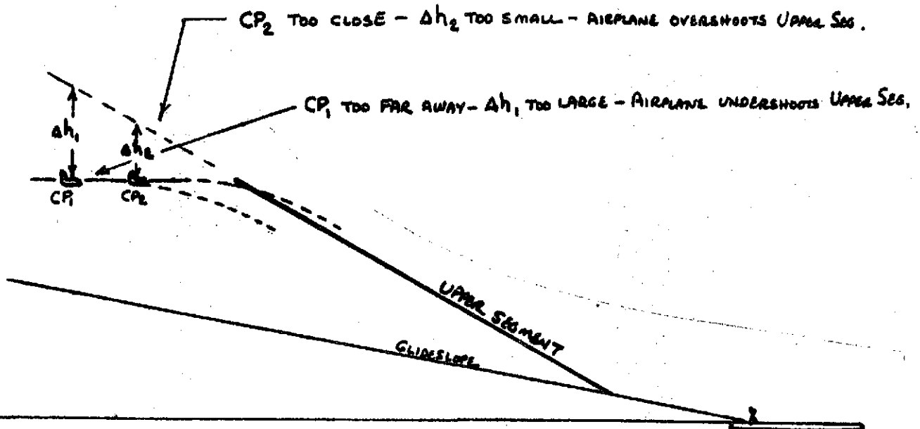
UPPER SEGMENT CAPTURE POINT AS FUNCTION OF \Delta h AND GROUND SPEED
