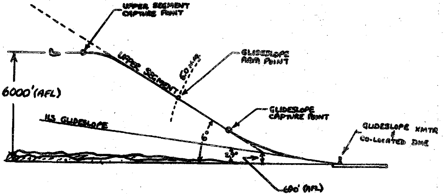
2-SEGMENT PROFILE (ANGLES EXAGGERATED-DIST NOT TO SCALE)
