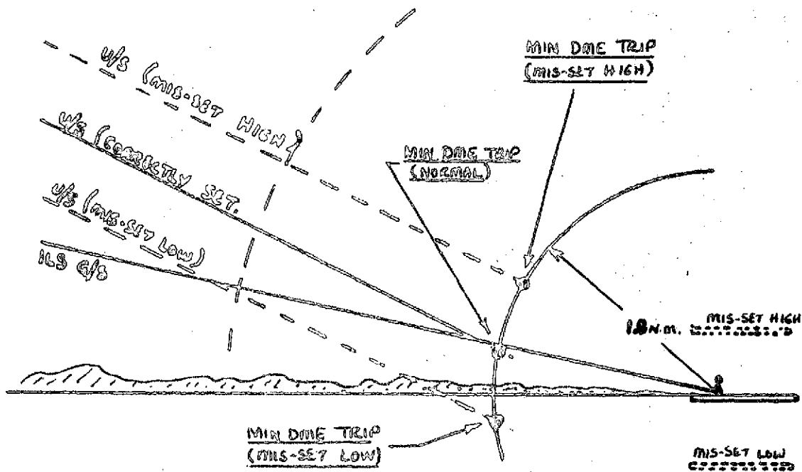
FIGURE 5 - MINIMUM DME TRIP - INCLUDING EFFECT OF MIS-SETTING AIRPORT ELEVATION HIGH OR LOW.
