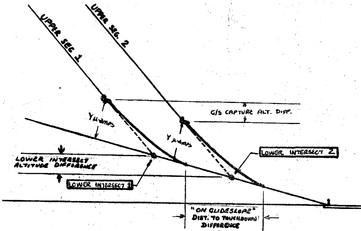
FIGURE 1 - EFFECT OF LOWER INTERSECT ALTITUDE UPON GLIDESLOPE CAPTURE POINT ALTITUDE AND ON-GLIDESLOPE DISTANCE TO TOUCHDOWN.
