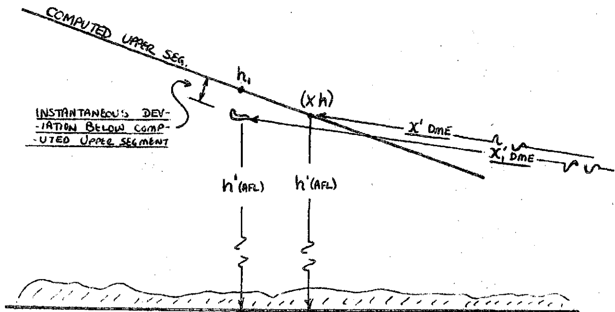
FIGURE 1 - UPPER SEGMENT DEVIATION - DME vs AFL
