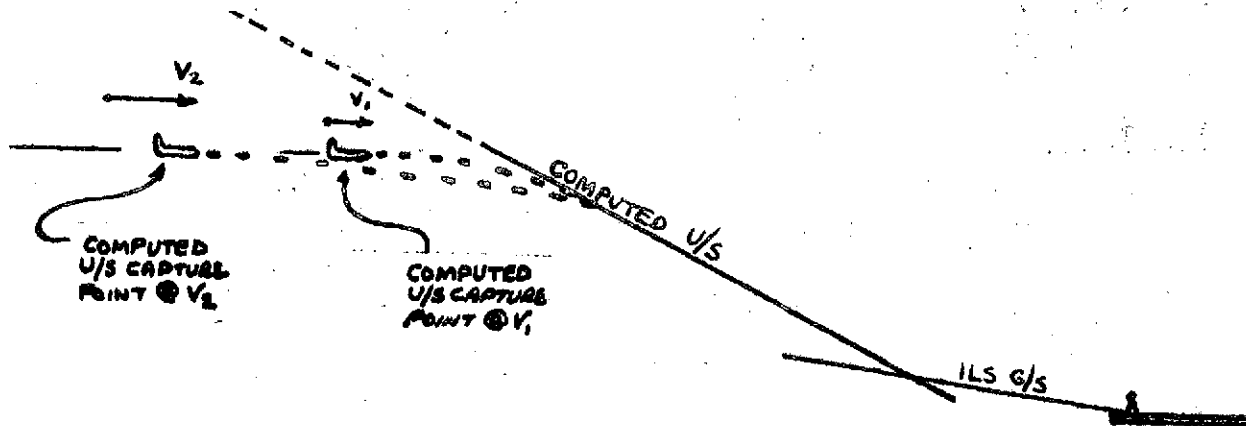
FIGURE 1 - UPPER SEGMENT CAPTURE POINT AS A FUNCTION OF RATE OF APPROACH TO UPPER SEGMENT .
