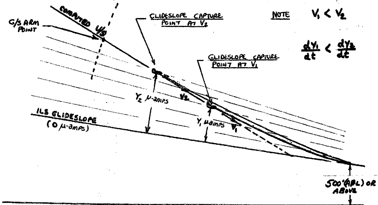
FIGURE 2 - GLIDESLOPE CAPTURE POINT AS A FUNCTION OF HEIGHT ABOVE G/S CENTER AND CLOSURE RATE
