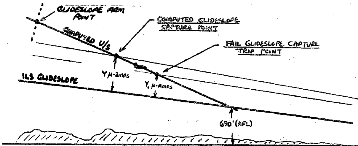
FIGURE 3 - GLIDESLOPE DEVIATION PROTECTOR - FAIL GLIDESLOPE CAPTURE
