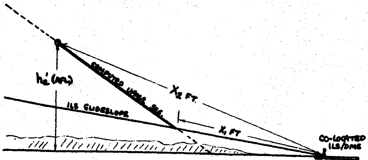
FIGURE 1 - UPPER SEGMENT DEFINITION
