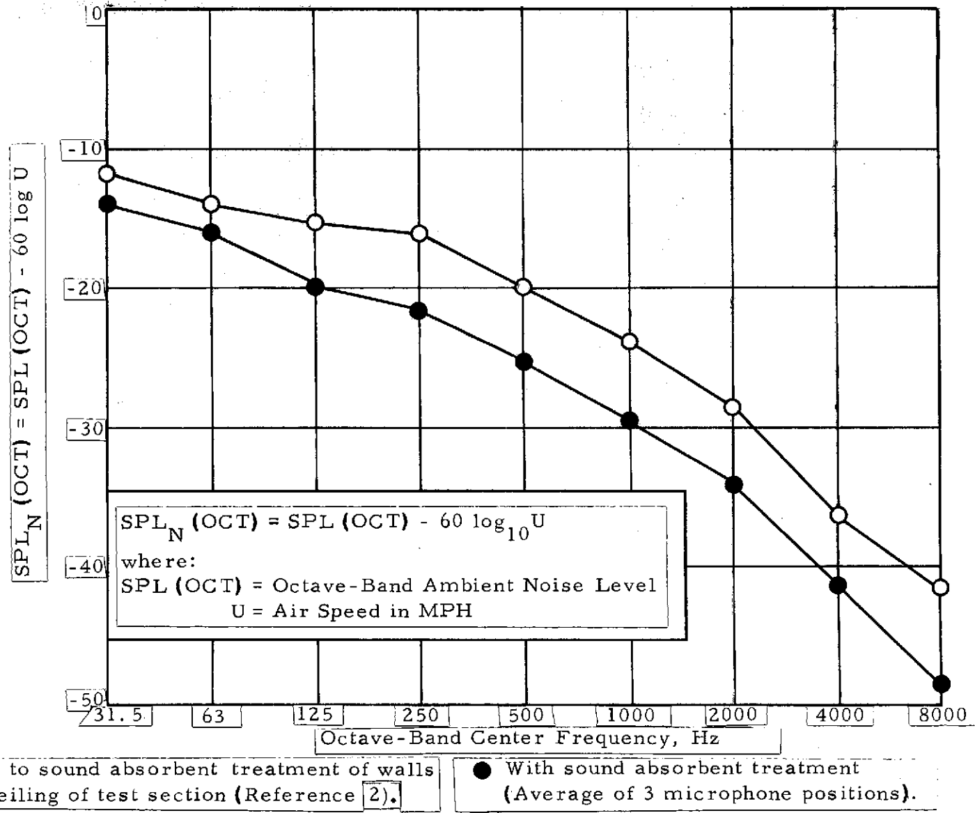
Figure 5. Comparison of Mean Normalized Octave-Band Ambient Noise Measurements Made Prior to and After Sound-Absorbent Treatment of Test Section.
