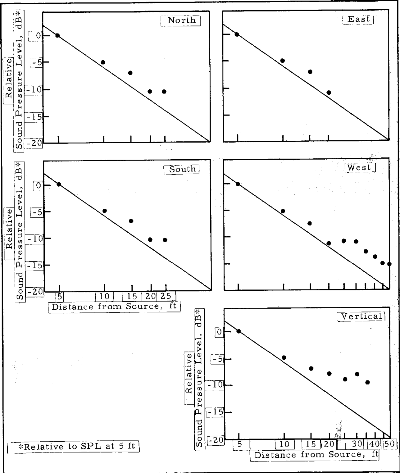
Figure 9c. Measured 250 Hz Octave-Band Sound Pressure Levels in Indicated Directions from Acoustic Source Located at Center of Test Platform.
