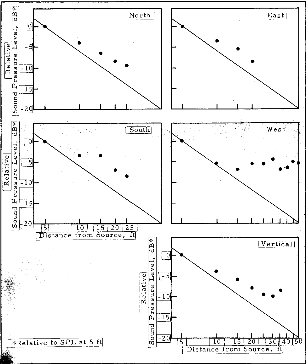
Figure 9a. Measured 63 Hz Octave-Band Sound Pressure Levels in Indicated Directions from Acoustic Source Located at Center of Test Platform.
