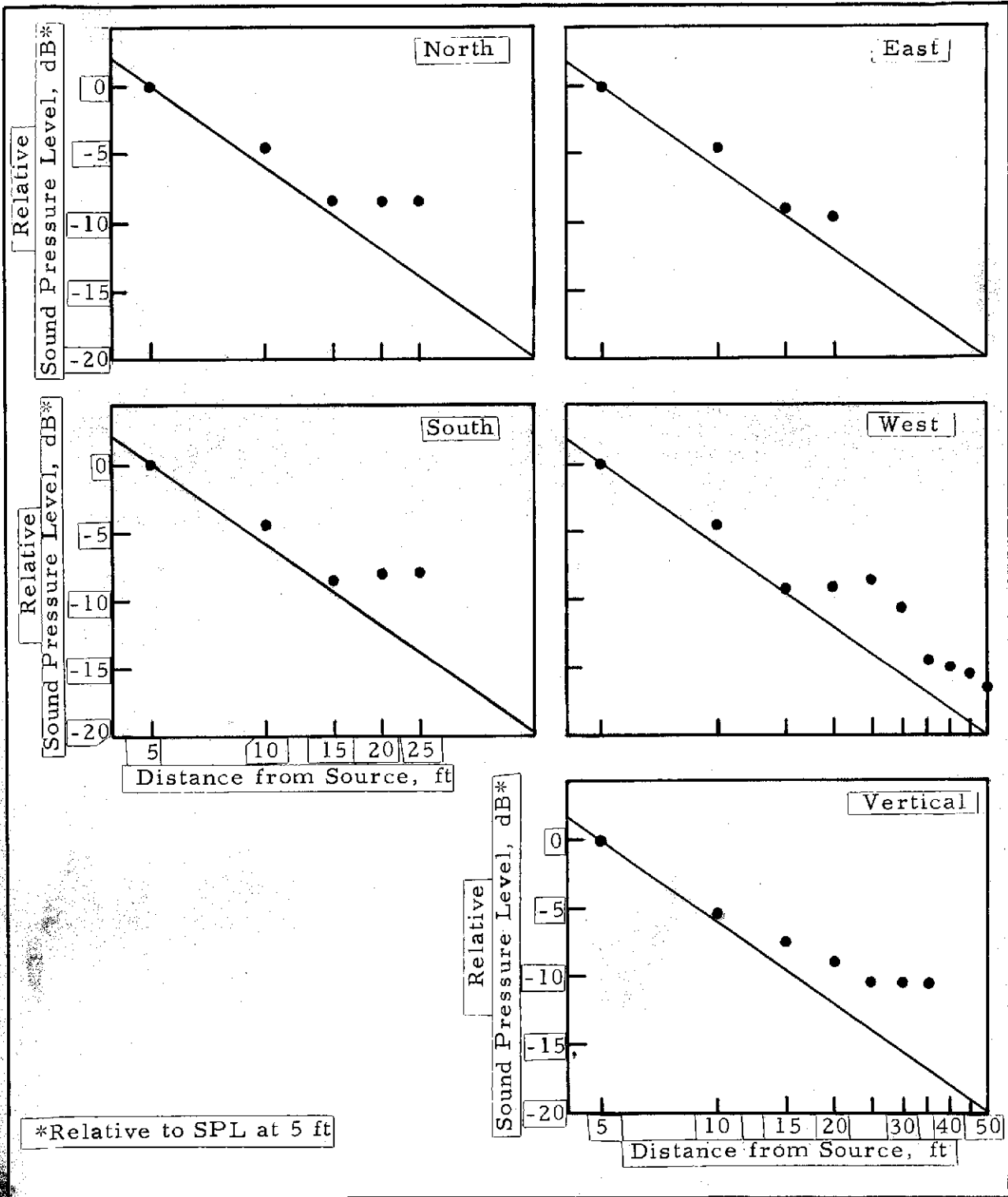
Figure 9b. Measured 125 Hz Octave-Band Sound Pressure Levels in Indicated Directions from Acoustic Source Located at Center of Test Platform.
