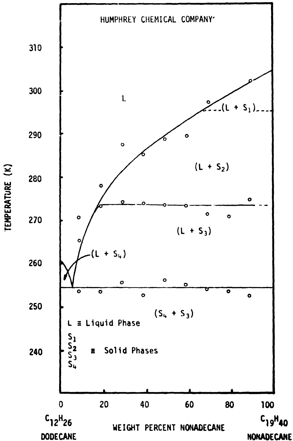
Figure 17. Dodecane - Nonadecane Binary System
