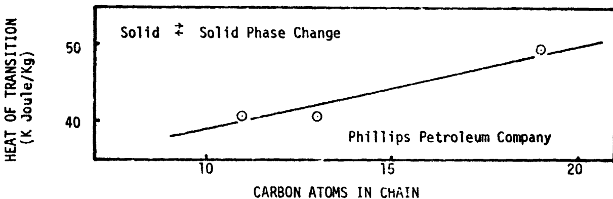
Figure 6(b) Effect of Carbon Chain Length on Heat of Transition
