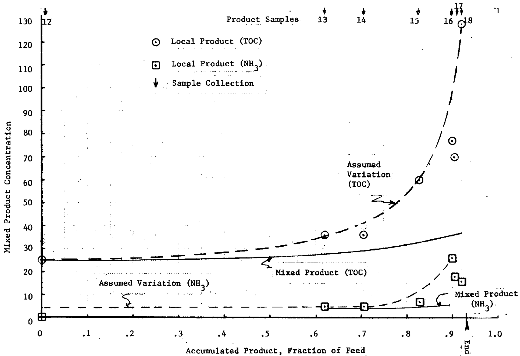
Figure 17 . Calculation of Product Water Quality versus Feed Recovery (P = 6.6 x 10 6 n/m 2 , V = 3to7M/sec, T = 75C)
