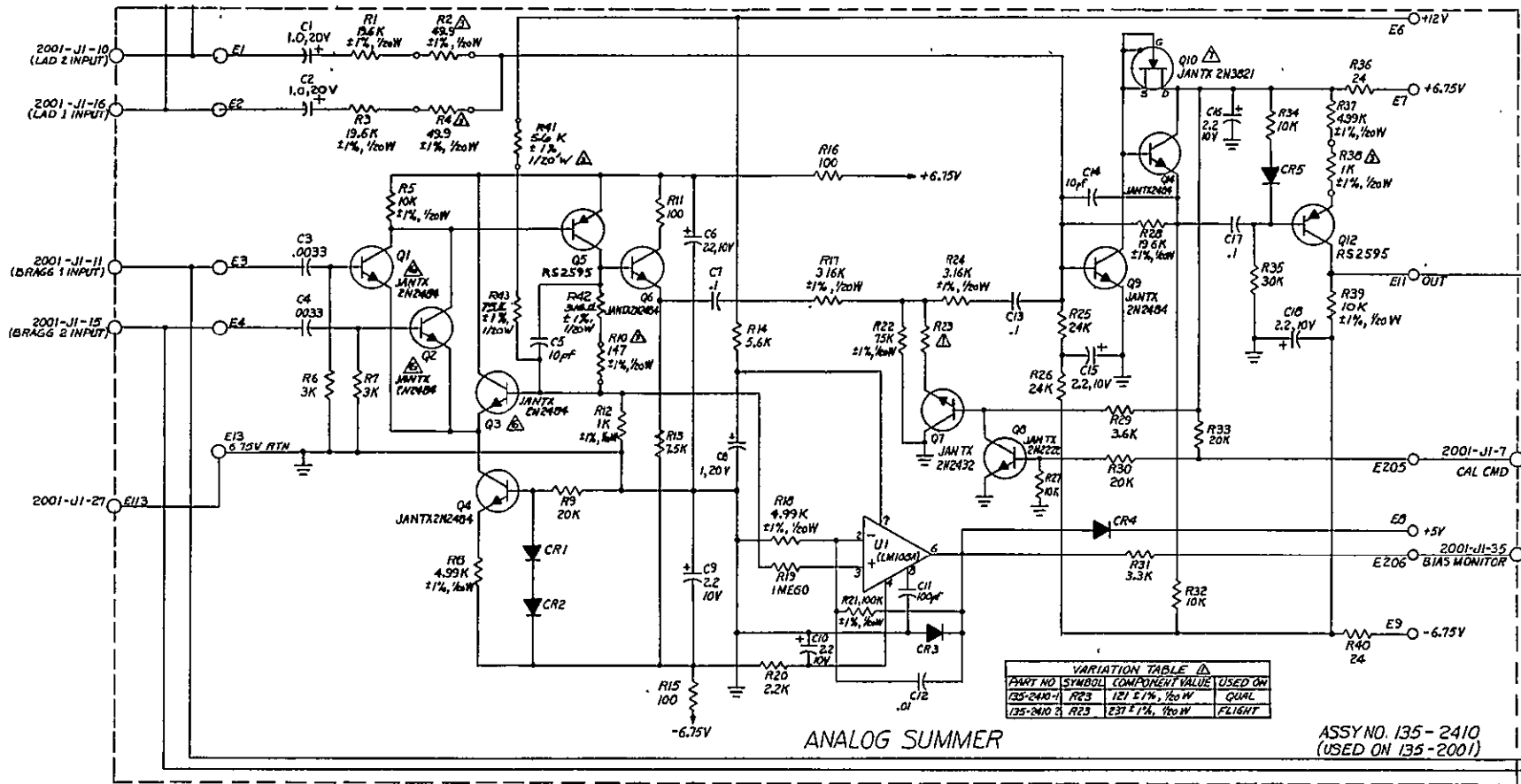
Figure 2-4. Analog Summer Assembly No. 135-2410
