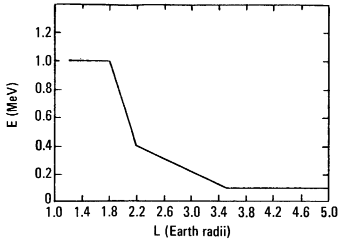
Figure 53.— Recommended low energy limit for Model AP5 (ref. 116).
