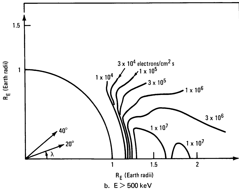
Figure 31.—Model AE5 (ref. 7) omnidirectional electron flux as function of R_E and latitude \lambda (cont.).
