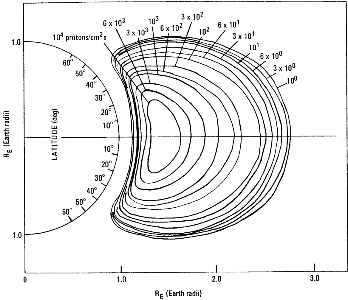
Figure 44.—Model AP7 omnidirectional proton flux as function of R_E and latitude ( > 50 MeV) (ref. 118).
