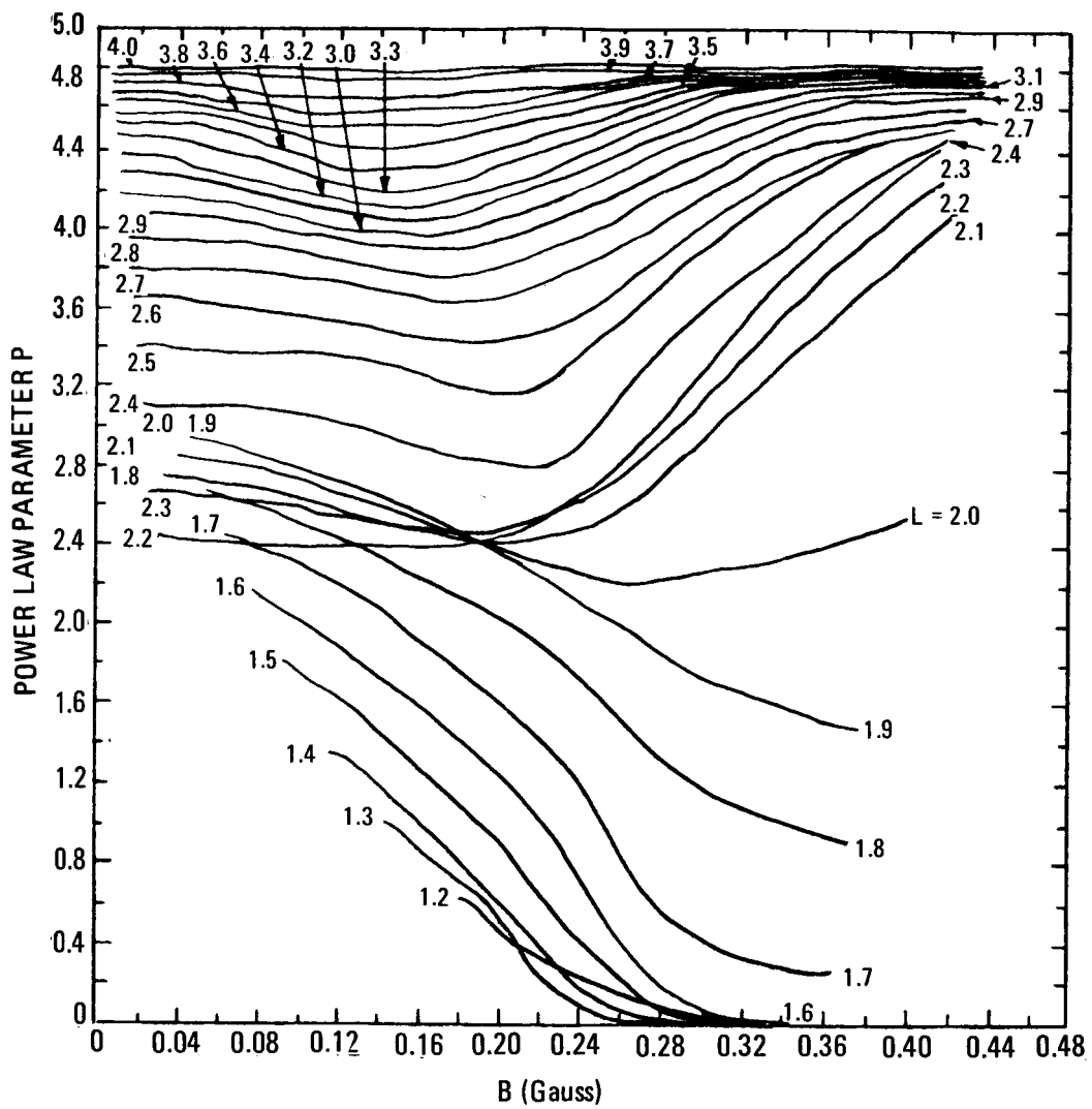
Figure 49.—Spectral parameter P for Model AP6 (ref. 117).
