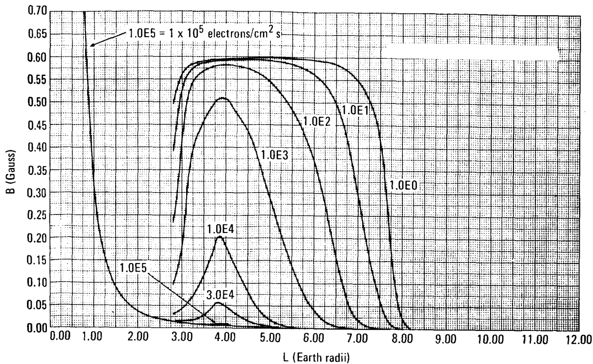
Figure 37.—Model AE4 omnidirectional electron flux for Epoch 1967 as function of B and L (ref. 6).
