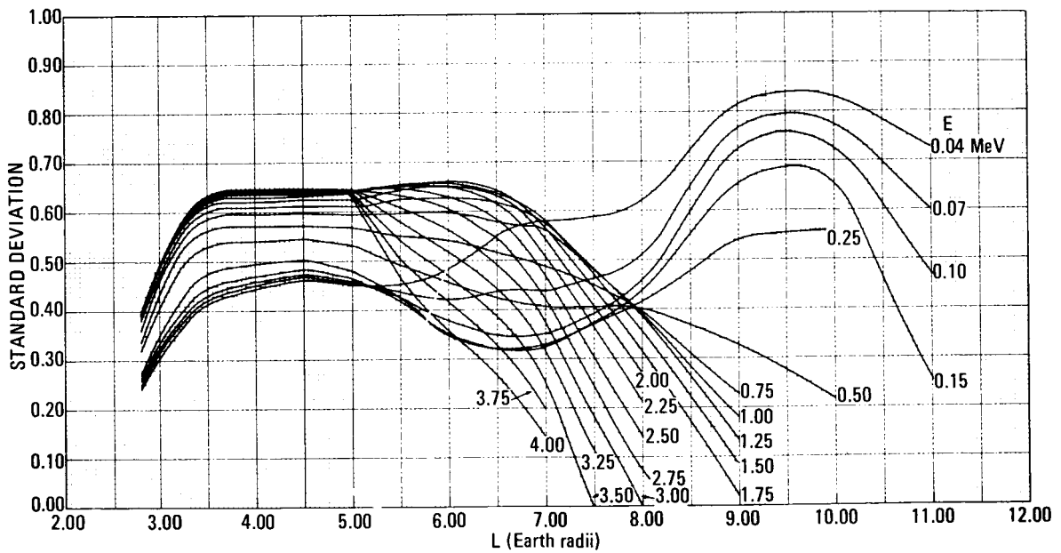
b. L variation for constant energy
