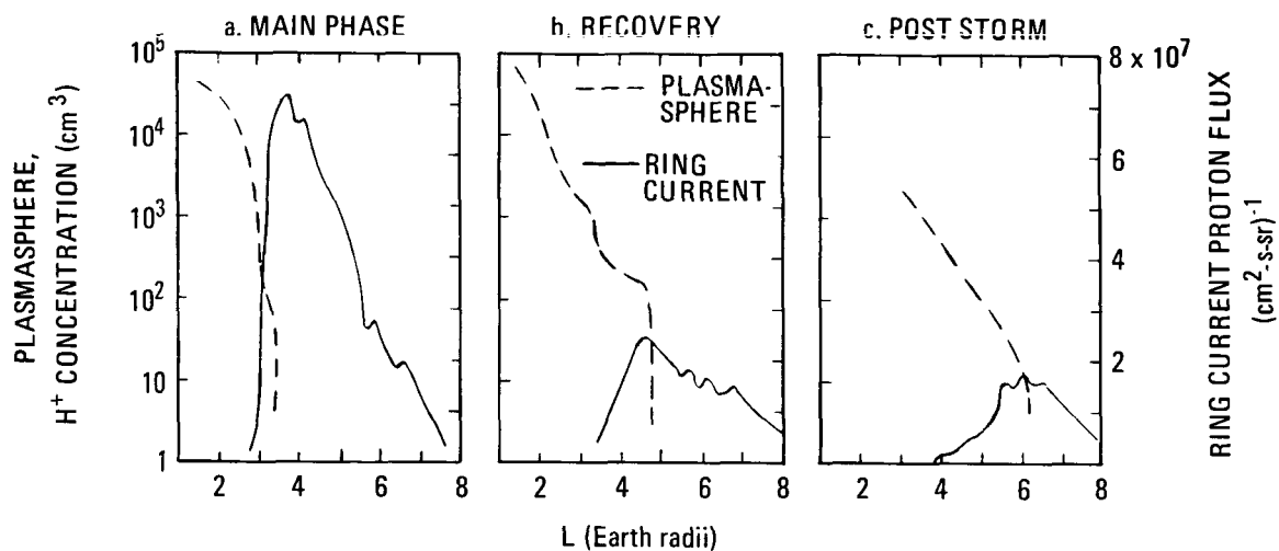
Figure 26.—Location of ring current and plasmopause—July 1966 magnetic storm (ref. 30).
