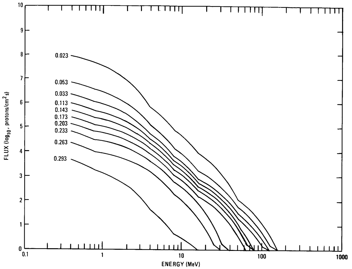
Figure 57.—Energy integrated omnidirectional proton flux (ref. 121).
