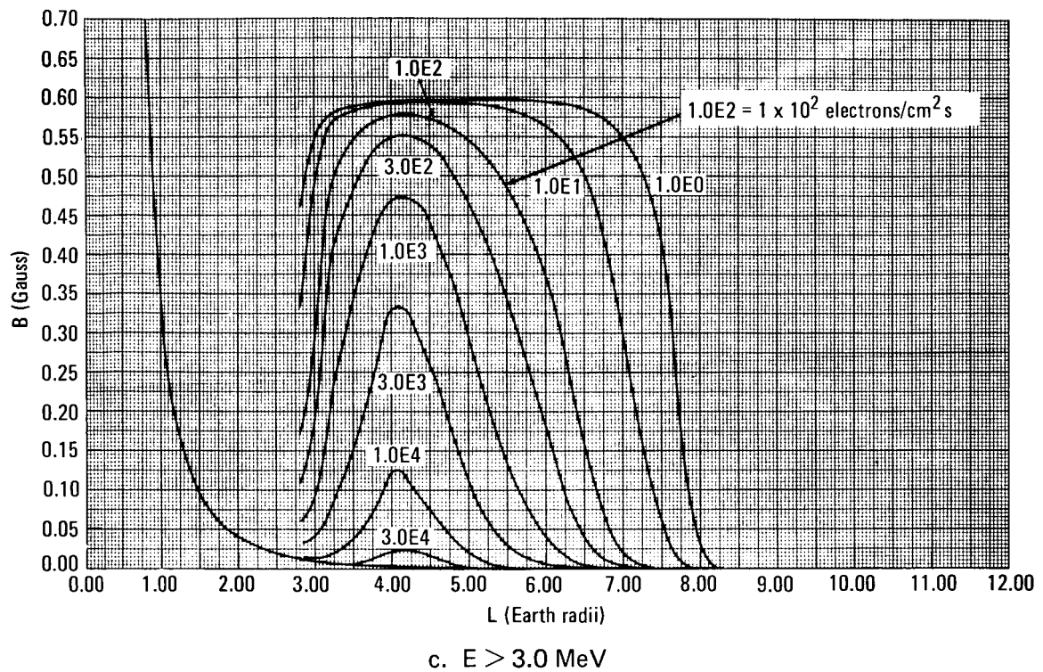
Figure 36.—Model AE4 omnidirectional electron flux for Epoch 1964 as function of B and L (ref. 6).
