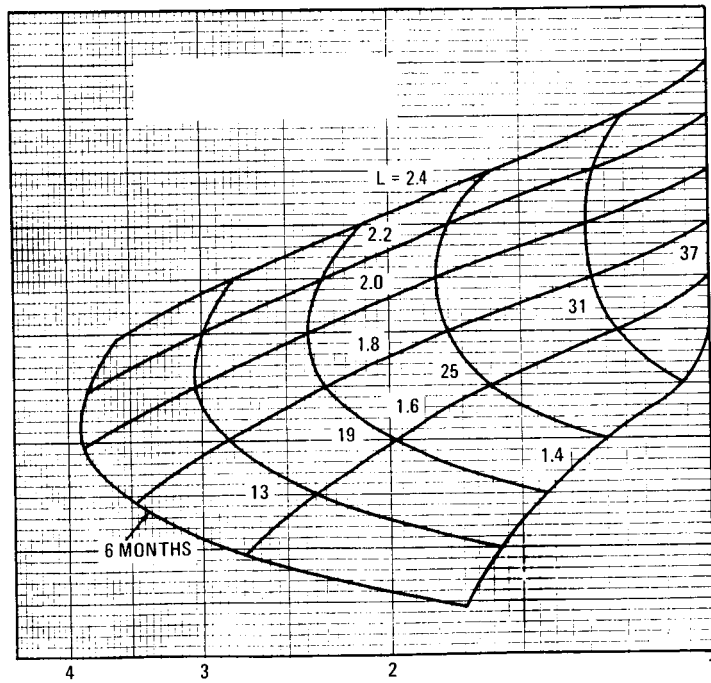
b. E > 100 keV, at 6 month and 0.2 L intervals
