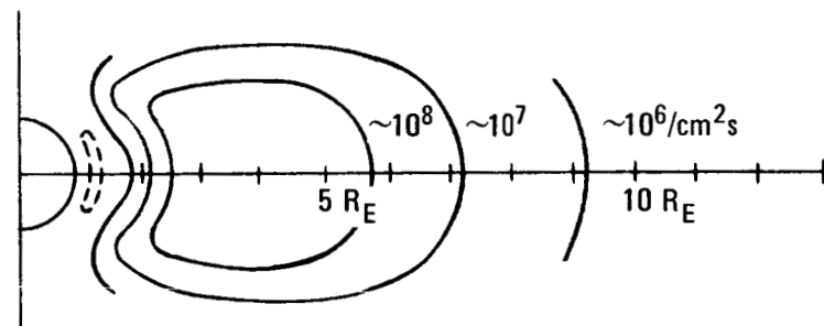
c. PROTON FLUX, 1.0 < E < 5 MeV
