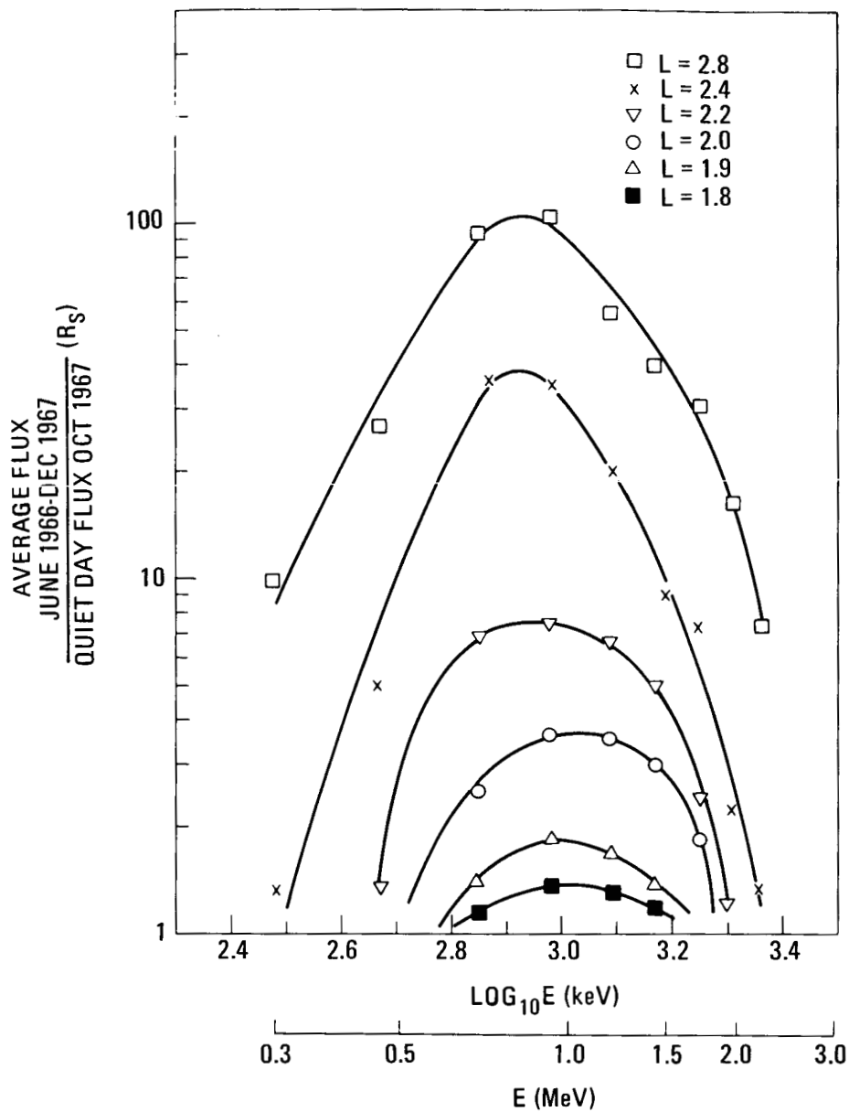
Figure 29.—Magnetic storm flux ratio R_s (ref. 7).
