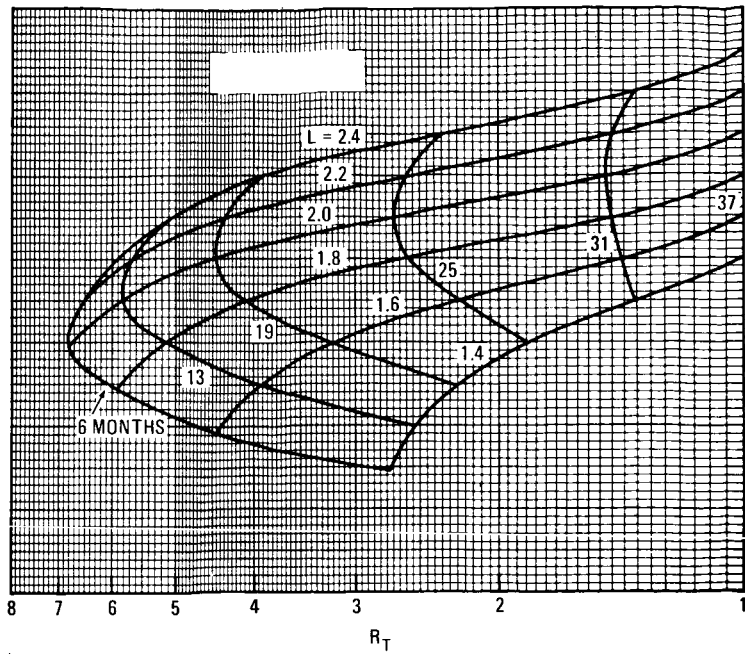
c. E > 250 keV, at 6 month and 0.2 L intervals
