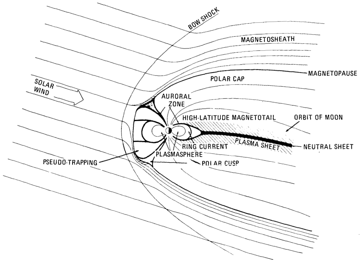
Figure 3.—Regions of the magnetosphere shown in the noon-midnight meridian plane.
