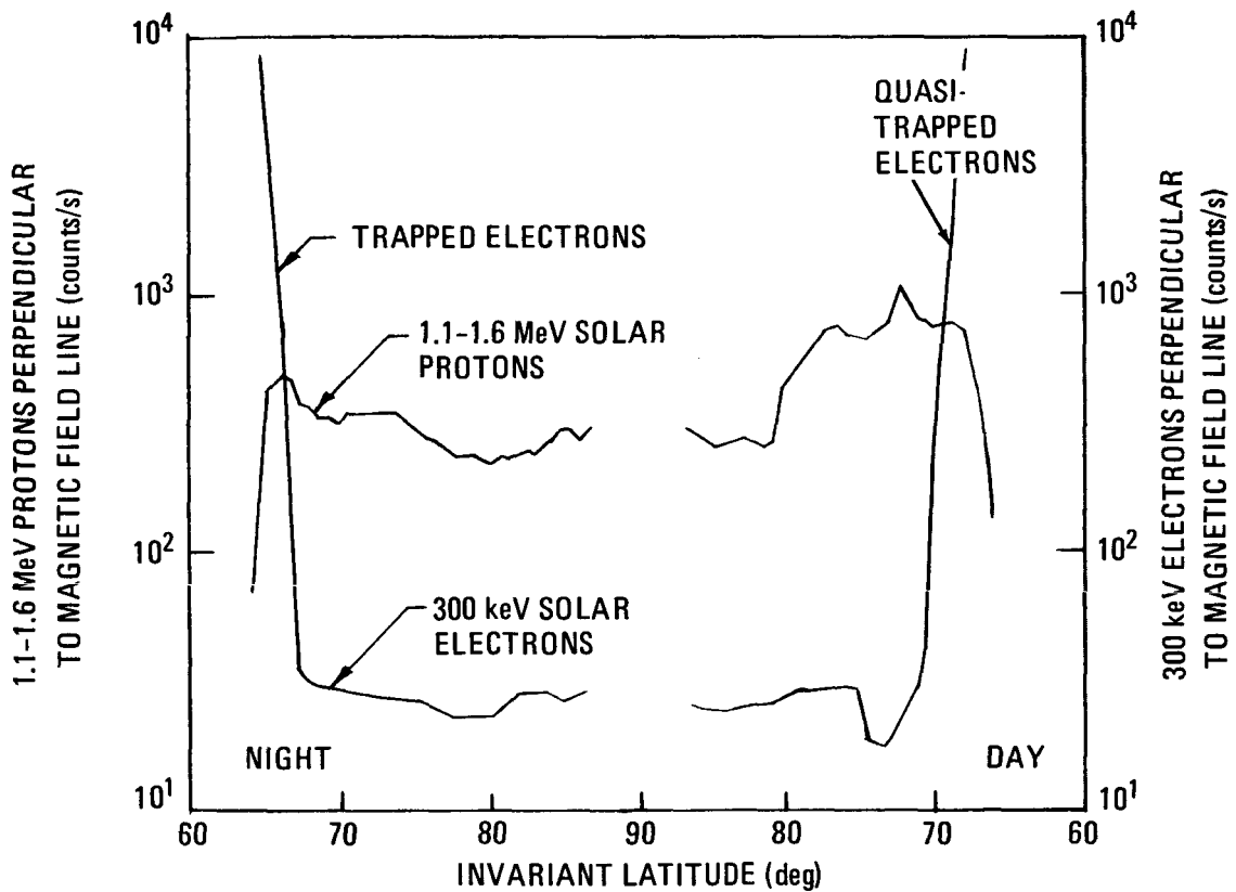
Figure 8.—Polar cap profiles of solar proton and electron fluxes at 4,000 km (ref. 24).
