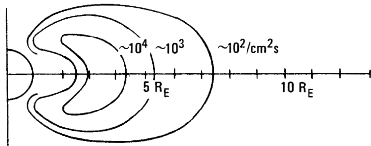
b. ELECTRON FLUX, E > 1.6 MeV
