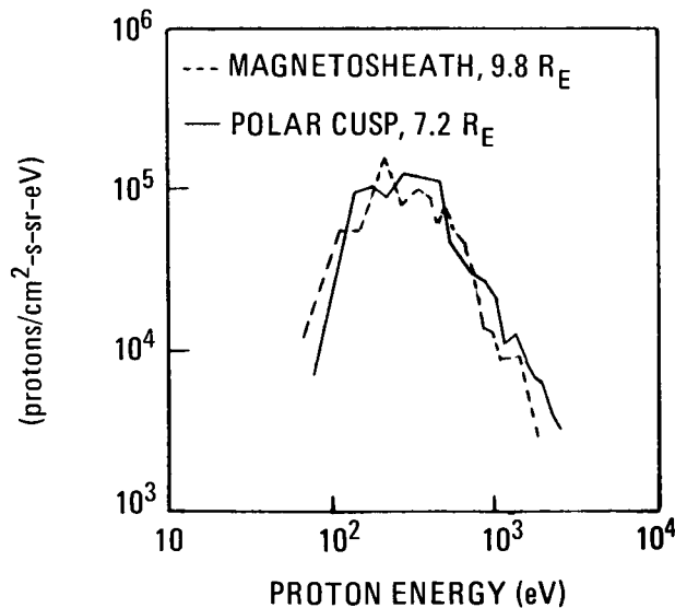
Figure 7.—Proton differential energy spectrums in polar cusp and magnetosheath (ref. 14).
