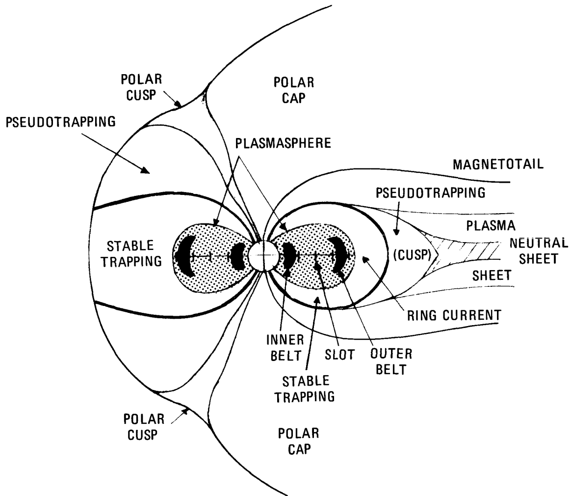
Figure 4.—Trapping regions in the magnetosphere.
