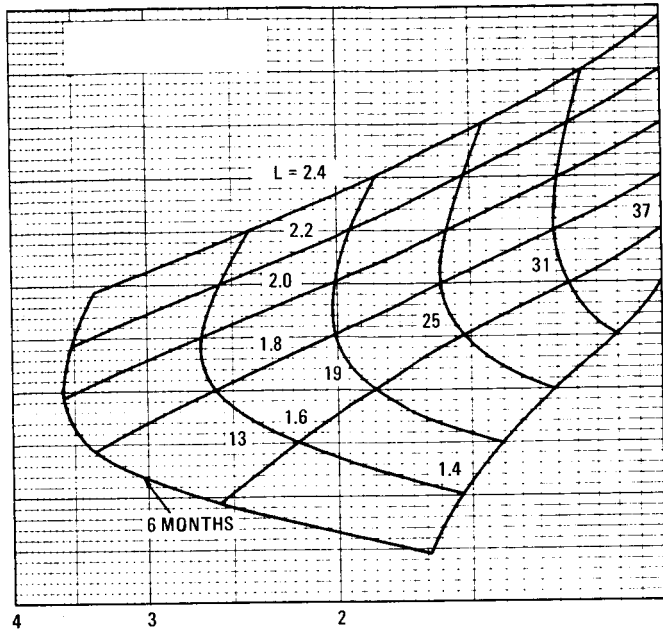
a. E > 40 keV, at 6 month and 0.2 L intervals
