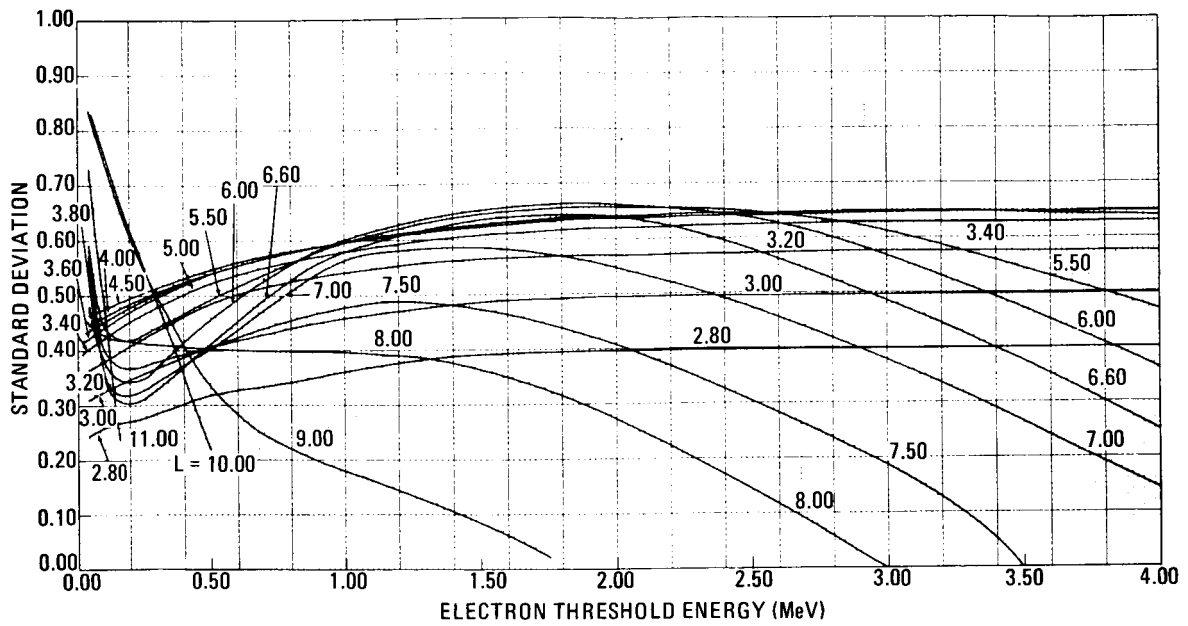
a. Energy variation for constant L
