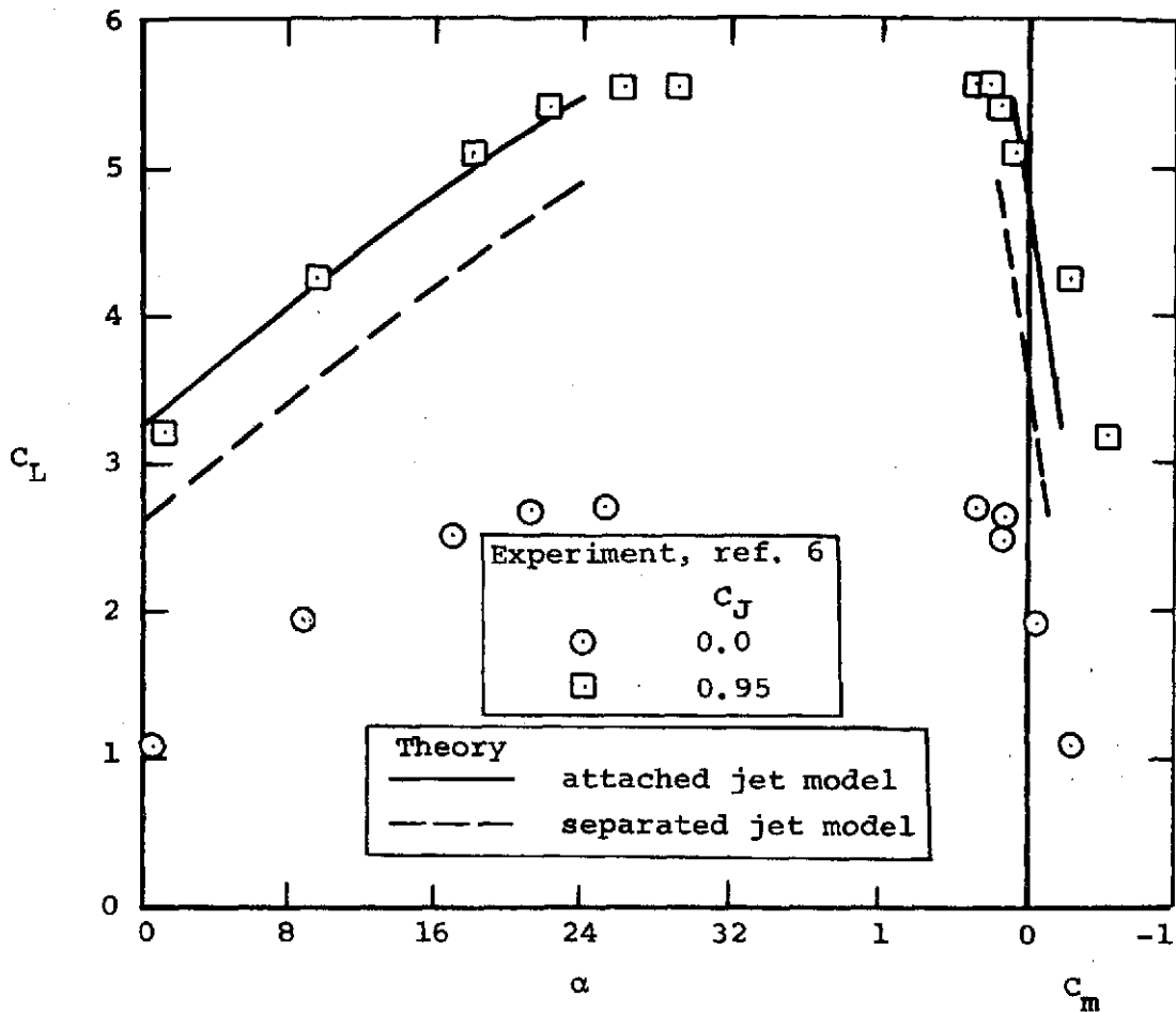
Figure 13.- Effect of jet separation on the predicted lift and pitching-moment coefficients of a two-engine USB model, tail off, \delta_f = 55^\circ .
