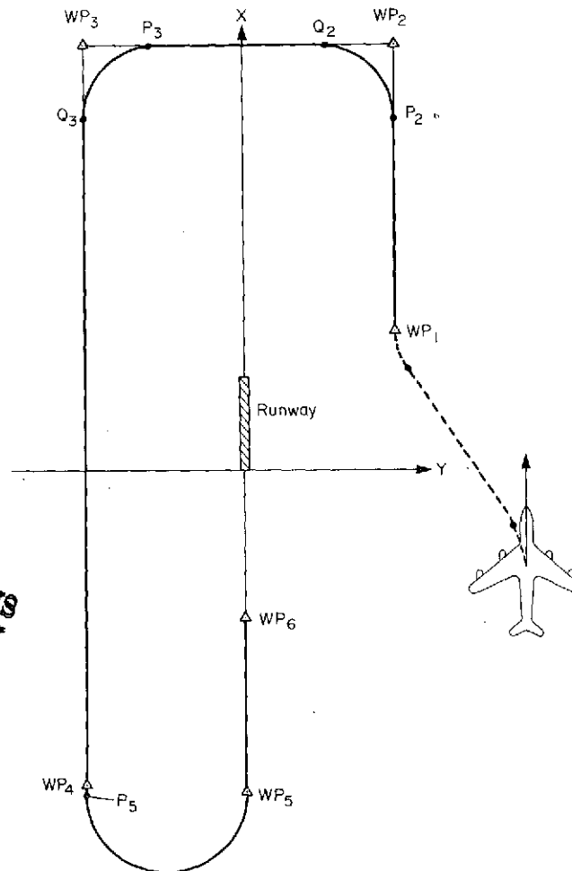
Figure 18.— Ground track for example problem.
