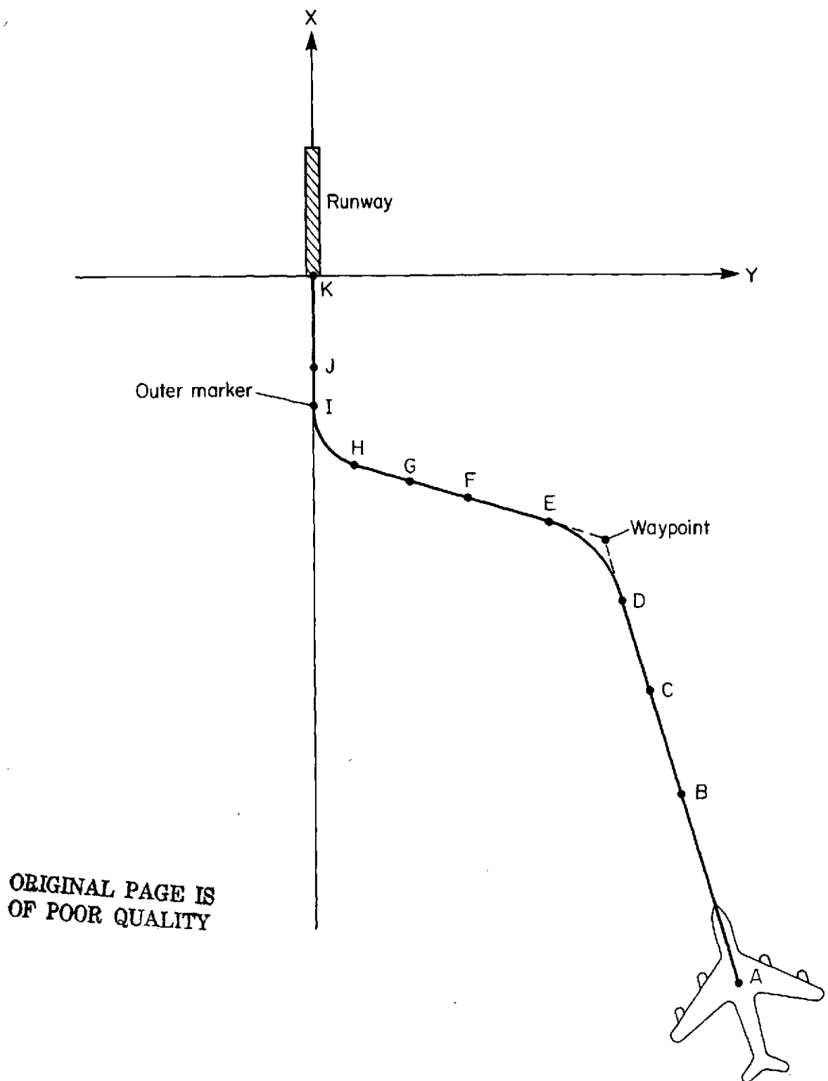
Figure 1.— Ground track of aircraft in terminal area.
