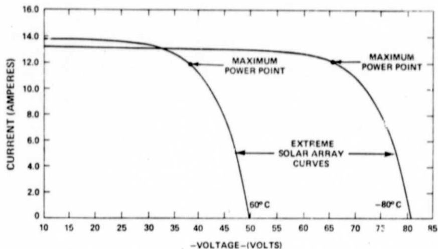
TEMPERATURE EFFECT ON I-V CURVE
