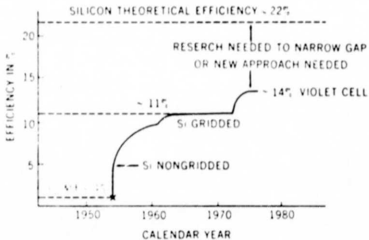
SILICON SOLAR CELL EFFICIENCY VS TIME
