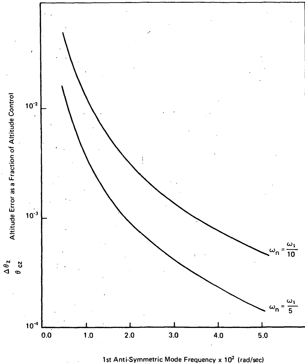
FIGURE 49. — VARIATION OF THE 1st ANTI-SYMMETRIC YAW MODE FREQUENCY WITH ATTITUDE ERROR
