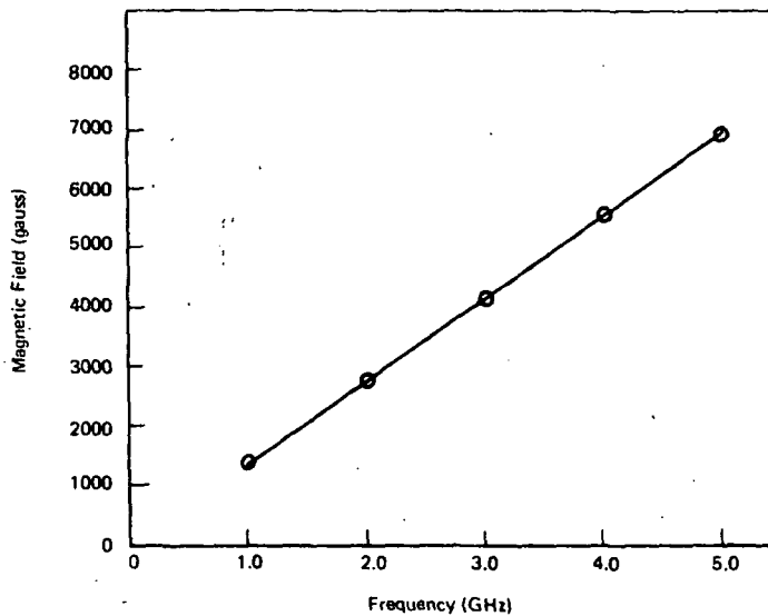
FIGURE 61. – MAGNETIC FIELD VERSUS FREQUENCY
