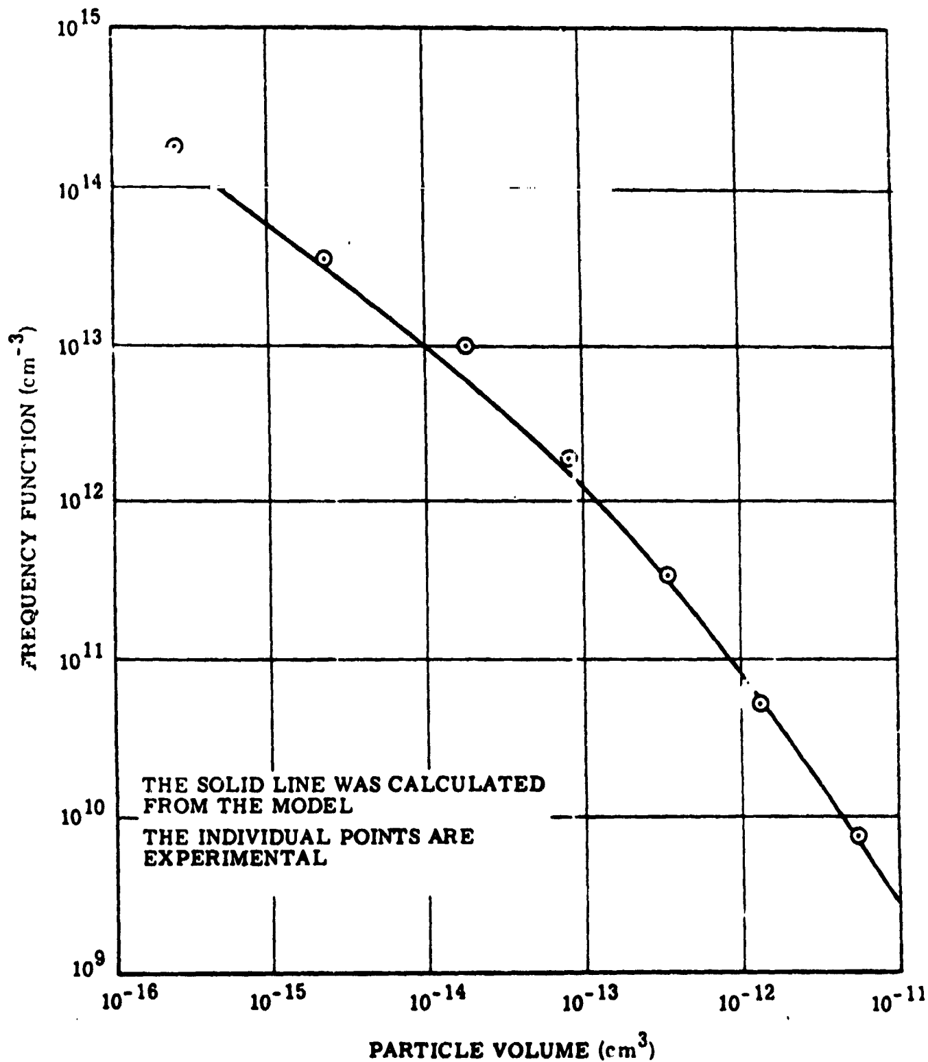
FIGURE 2. THEORETICAL AND EXPERIMENTAL FREQUENCY FUNCTIONS AT A CHAMBER PRESSURE OF 500 PSI (Fein, 1965).
