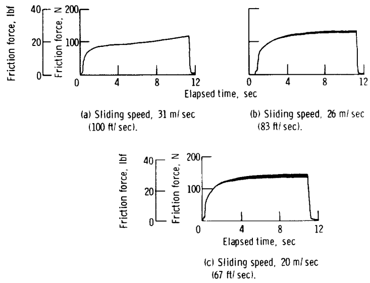
Figure 7. - Friction data obtained from carbon graphite - fine fibers (CG-FF) sliding against a 17-22 AS steel disk under a normal load of 382 N (86 lbf).
