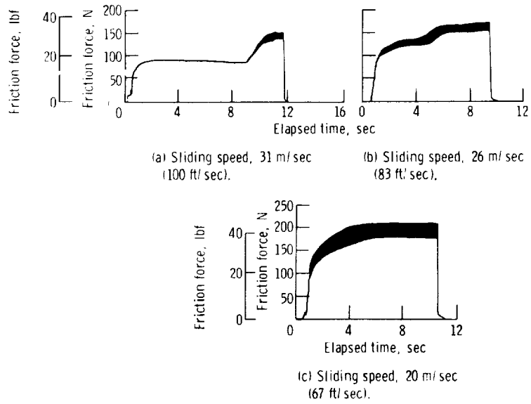
Figure 10. - Friction data obtained from graphite-cloth-reinforced composite (GCRC) sliding against a graphite-cloth-reinforced-composite disk under a normal load of 382 N (86 lbf).
