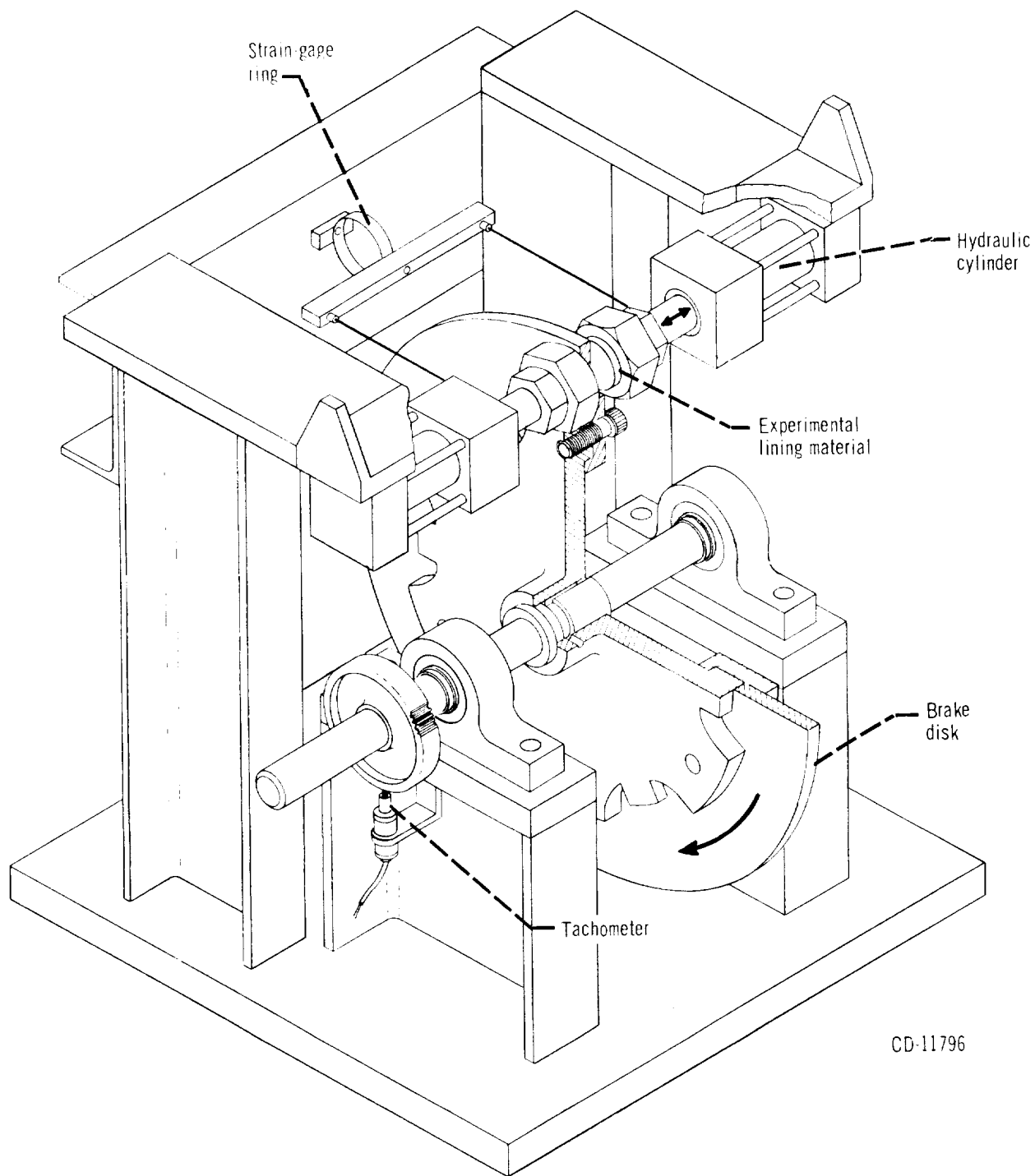
Figure 1. - Brake apparatus.
