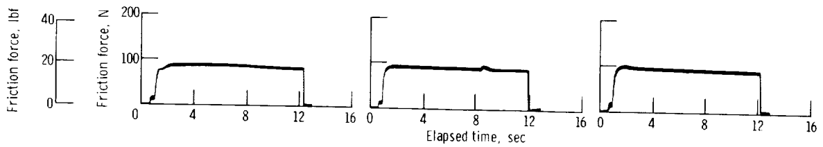
(a-1) Sliding speed, 31 m/sec (100 ft/sec). (a-2) Sliding speed, 26 m/sec (83 ft/sec). (a-3) Sliding speed, 20 m/sec (67 ft/sec).
