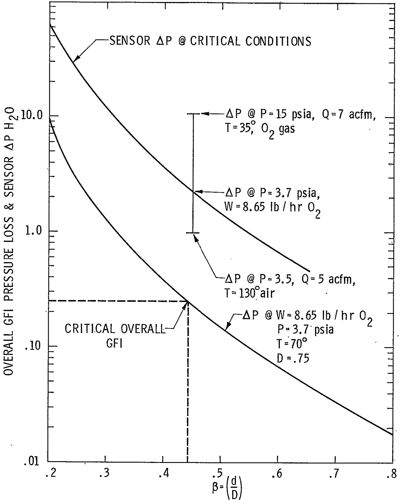
Figure D-10. Venturi Pressure Drop Characteristics
