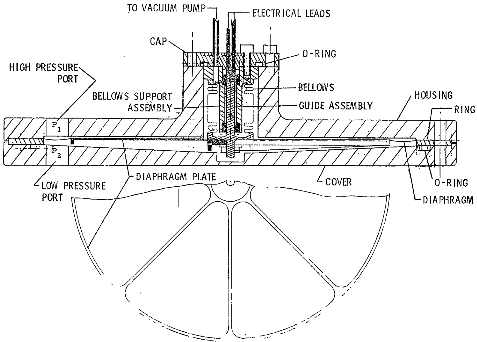
Figure 4. Details of Breadboard Compensator (Initial Design)
