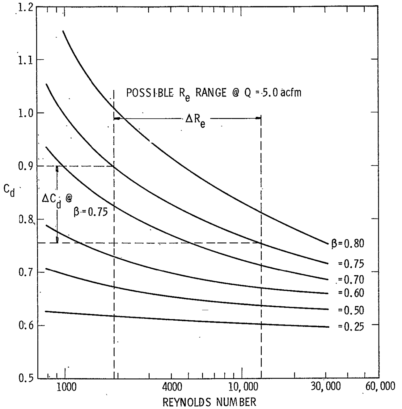
Figure D-5. Orifice C_d vs Re
