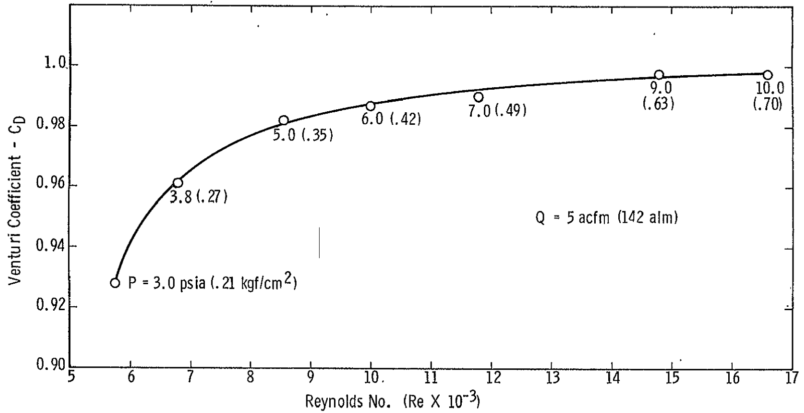
Figure 13. Discharge Coefficient versus Re (Rosemount Venturi)
