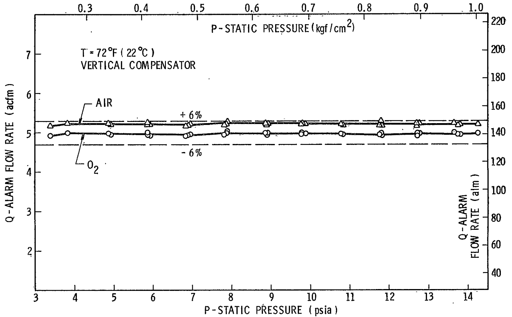
Figure 21. Prototype Alarm Q vs P for Air and O 2
