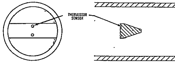
(a) FRONT FACE THERMISTOR TECHNIQUE
