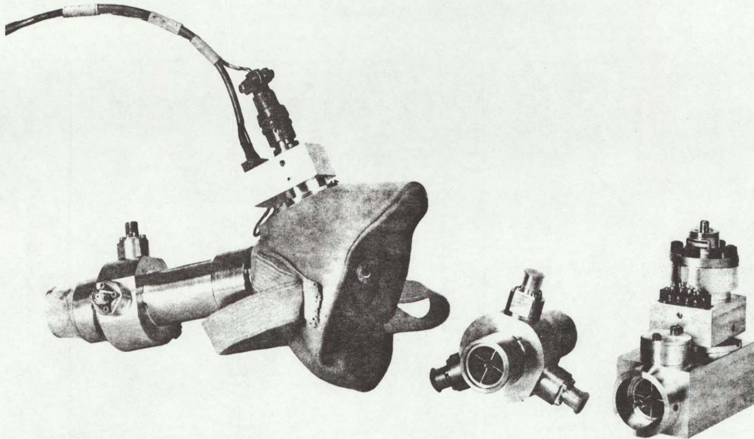
Figure B-5. 3/4" BI-DIRECTION RESPIRATORY FLOWMETER
