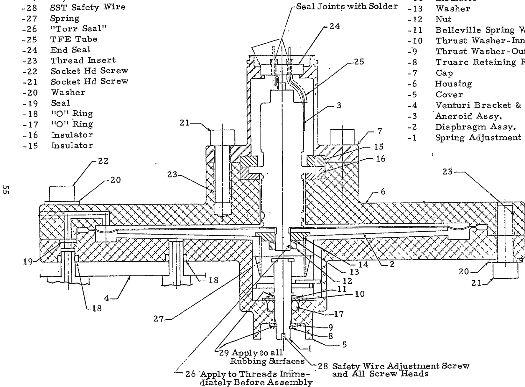
FIGURE 18. GFI ASSEMBLY DRAWING OF COMPENSATOR
