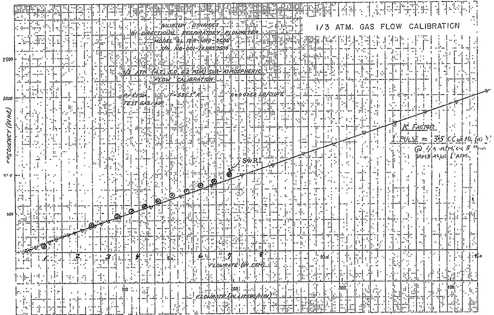
Figure E-2. 1/3 Atm. Gas Flow Calibration
