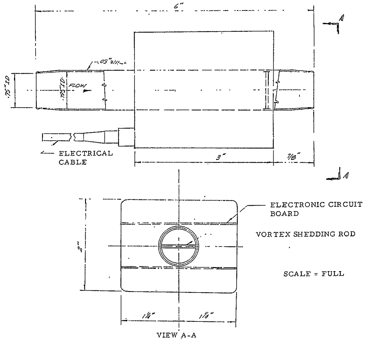
Figure C-8. Dimensional Envelope of VSM-GFI
