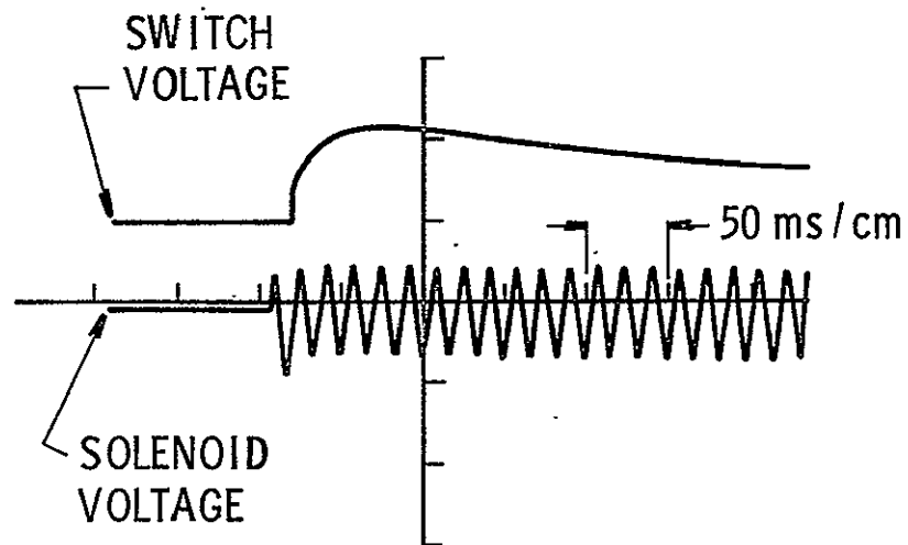
(b) 50 ms/cm
