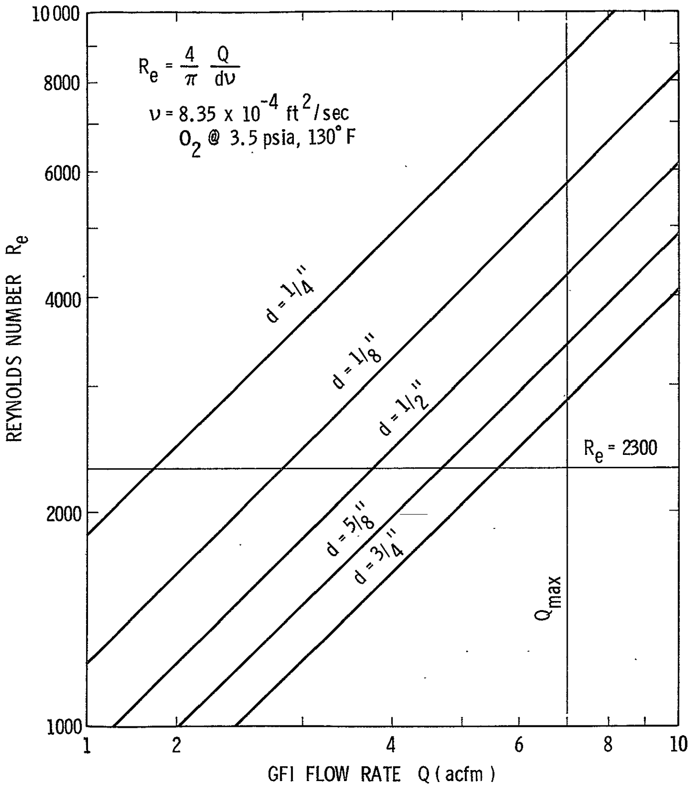
Figure A-6. Reynolds Number versus GFI Flow Rate @ \nu = 8.35 \times 10^5 \text{ ft}^2/\text{sec}
