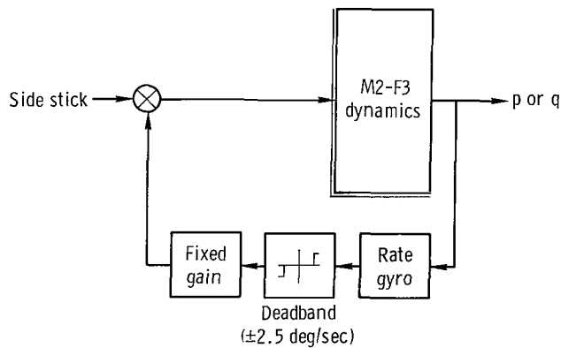
Figure 7. Simplified block diagram of M2-F3 pitch or roll RCS and RAS mechanization.
