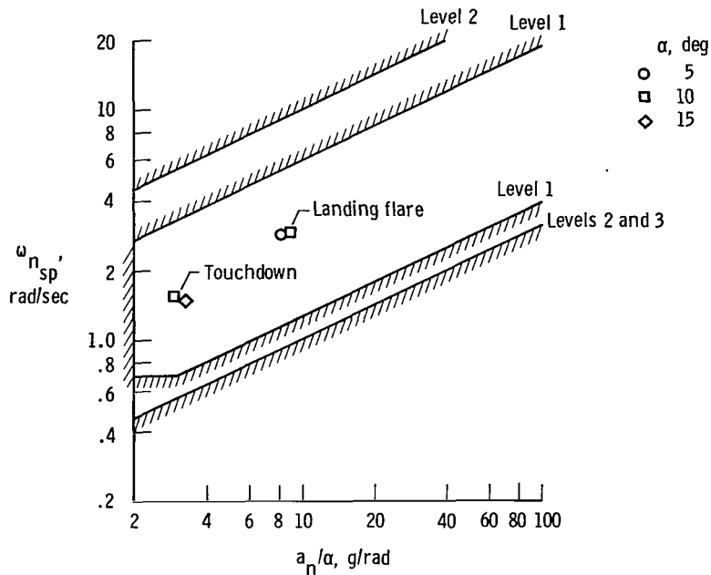
(b) Frequency and acceleration sensitivity, K_q = 0.4 \text{ deg/deg/sec} .
