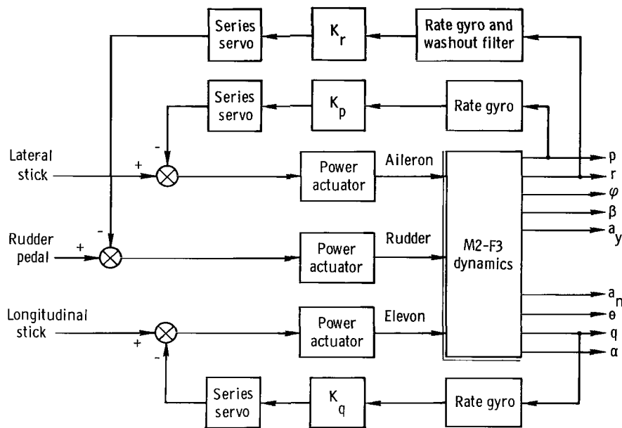
Figure 4. Simplified block diagram of M2-F3 flight control system.
