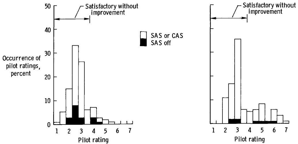
(b) Transonic and supersonic speeds and transonic configuration. SAS or CAS on, 111 ratings (93.3 percent); SAS off, 8 ratings (6.7 percent); total ratings, 119.
