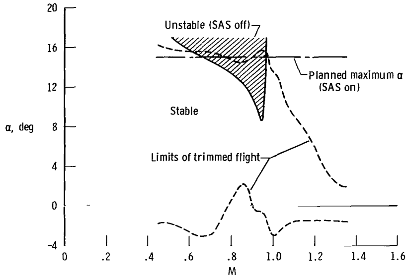
Figure 18. M2-F3 trimmed flight envelope and the longitudinal SAS-off stability boundary. \delta_u = -20^\circ ; center of gravity = 0.496\bar{c} .
