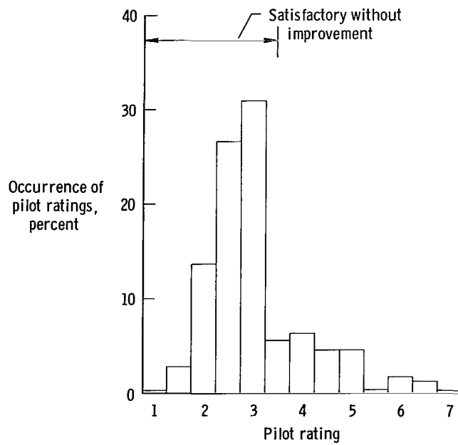
Figure 12. Percentage distribution of pilot ratings. Total ratings, 423.
