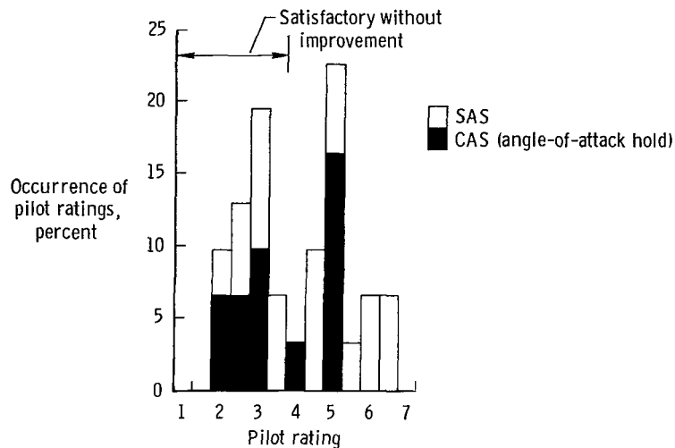
Figure 19. Percentage distribution of longitudinal transonic speed and transonic configuration pilot ratings for powered boost. Total ratings, 31.
