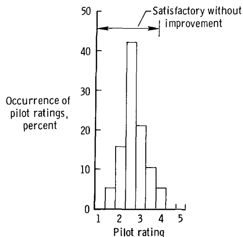
Figure 24. Percentage distribution of longitudinal pilot ratings for the landing task. Total ratings, 19.
