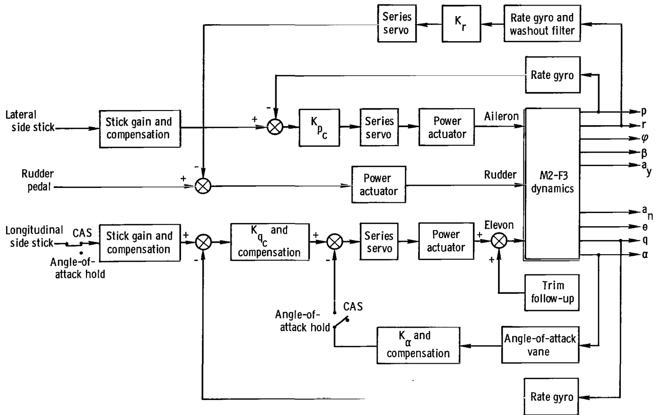
Figure 5. Simplified block diagram of M2-F3 command augmentation system. CAS engaged; angle-of-attack hold disengaged.
