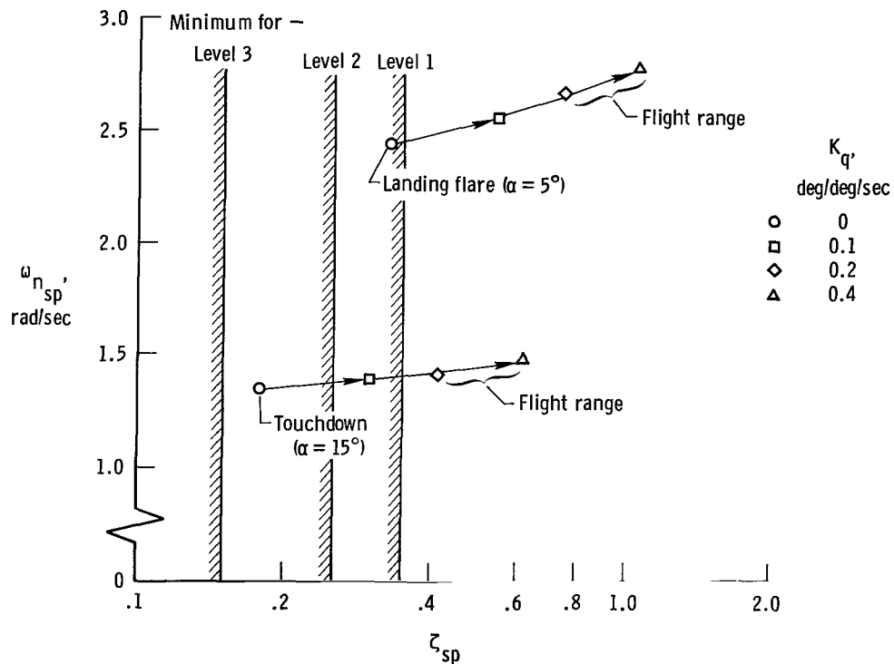
(a) Frequency and damping.
