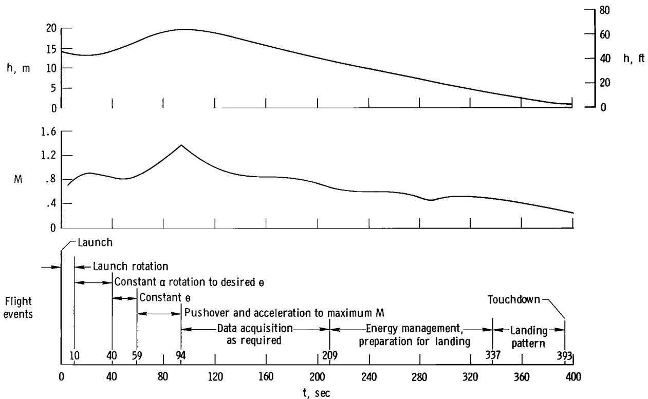
Figure 11. Typical M2-F3 powered flight profile.
