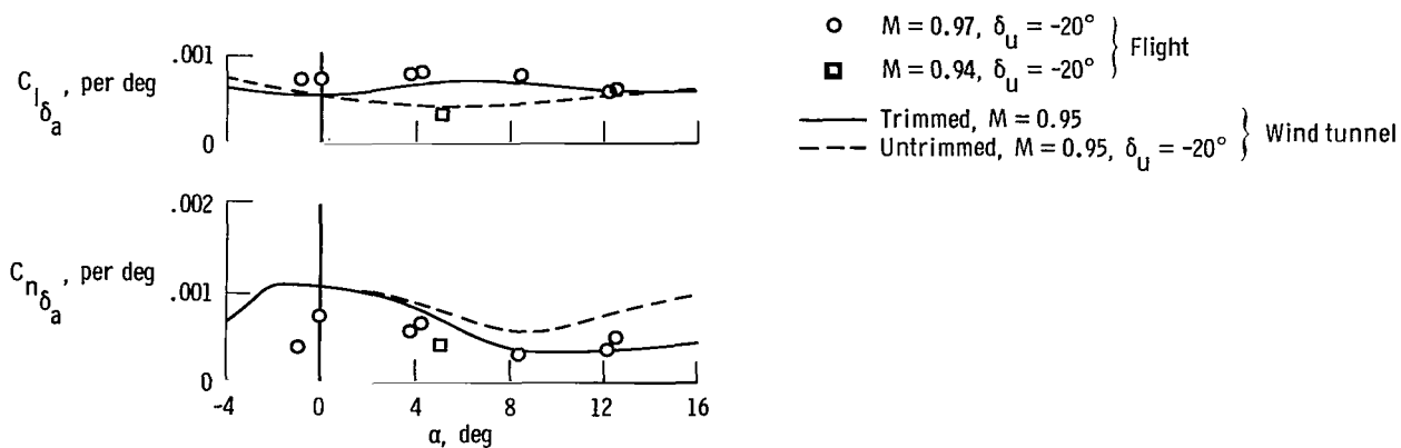
Figure 28. Comparison of aileron rolling-moment and yawing-moment effectiveness obtained from transonic flight data (ref. 6) and wind-tunnel data.
