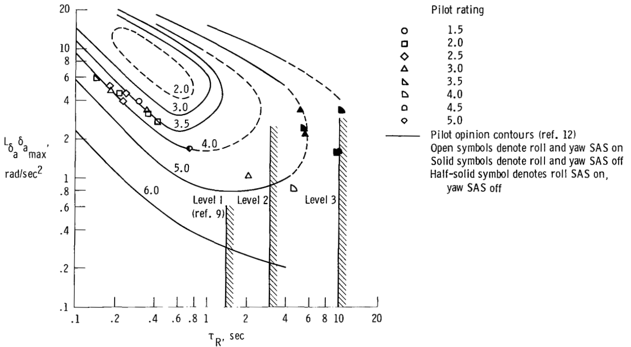
Figure 26. Comparison of M2-F3 lateral control power and roll mode time constant with criteria from references 9 and 12.
