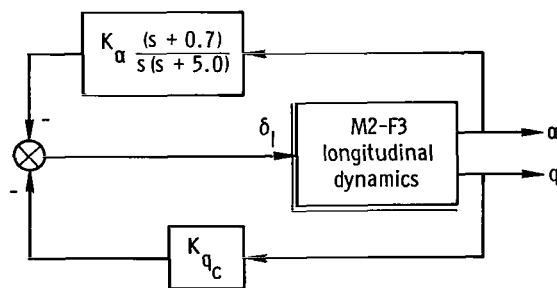
(c) Angle-of-attack hold.
