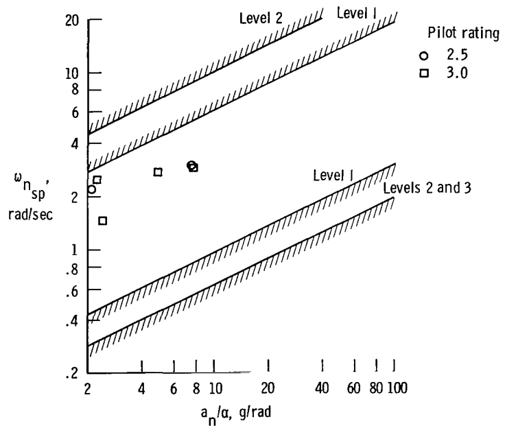
Figure 21. Comparison of M2-F3 longitudinal short-period mode frequency and acceleration sensitivity characteristics with Category B requirements from reference 9. M = 0.51 to 1.10 ; \alpha = 1.0^\circ to 8.5^\circ ; K_q = 0 to 1.0 deg/deg/sec.
