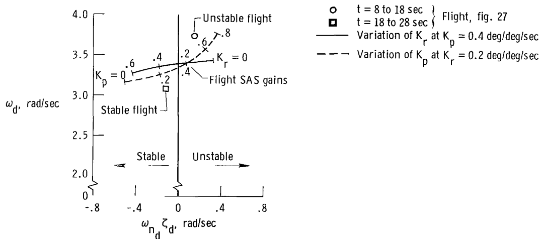
Figure 29. Theoretical root loci of the M2-F3 Dutch roll mode instability of figure 27 using linear flight-determined derivatives from reference 6. \alpha = 2.7^\circ ; M = 0.93 ; V = 283.5 m/sec (930 ft/sec); \bar{q} = 57.5 hN/m 2 (120 lb/ft 2 ).
