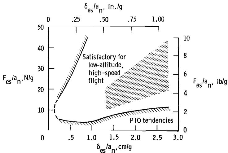
Figure 23. Comparison of the M2-F3 longitudinal stick force and stick travel per unit load factor (for the dynamics of fig. 22(a)) with the criterion of reference 11.
