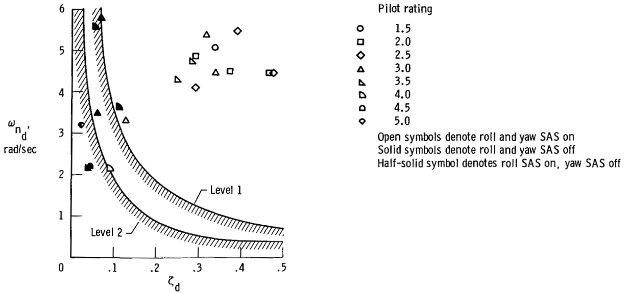
Figure 25. Comparison of M2-F3 Dutch roll mode frequency and damping ratio with criterion of reference 9 for Class II aircraft, Category B.
