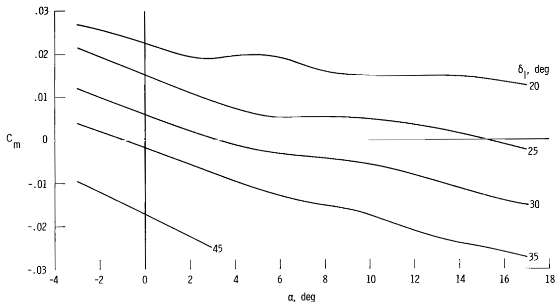
Figure 16. Pitching-moment curve from wind-tunnel data (ref. 6). M = 0.95 ; \delta_u = -20^\circ ; center of gravity = 0.496\bar{c} .
