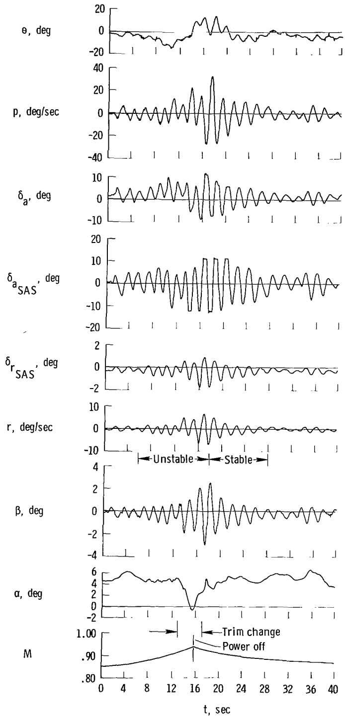
Figure 27. M2-F3 transonic SAS-on Dutch roll mode instability. K_p = 0.4 deg/deg/sec; K_r = 0.2 deg/deg/sec.
