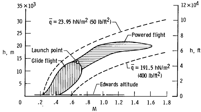
Figure 9. Approximate M2-F3 altitude and Mach number envelope.
