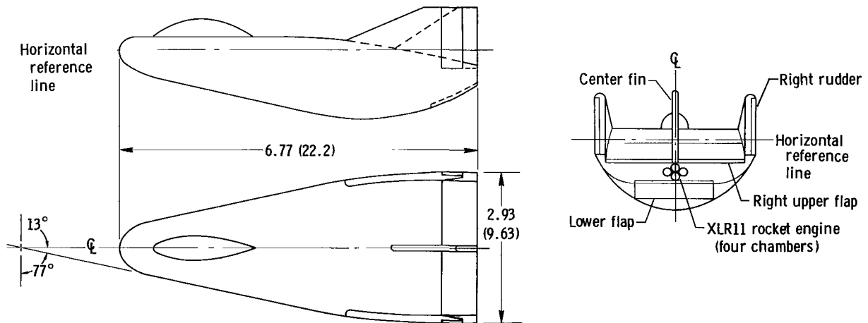
(b) Three-view drawing. Dimensions in meters (feet).
