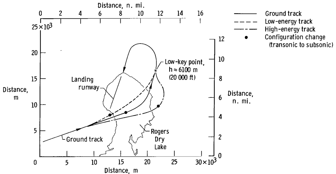
Figure 10. Typical M2-F3 flight ground tracks for the terminal approach and landing pattern.
