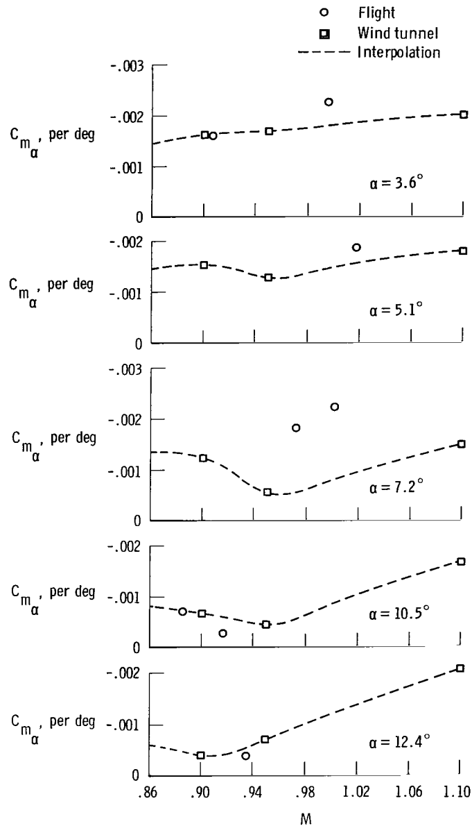
Figure 17. Comparison of static stability parameter obtained from flight data in the transonic speed region with wind-tunnel predictions (ref. 6). \delta_u = -20^\circ ; \delta_\ell as required for trim.
