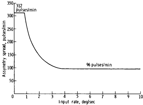
Figure 2. - Abort sensor assembly asymmetry requirements.
