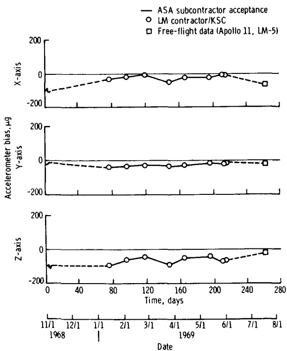
Figure 5. - Accelerometer bias history.
