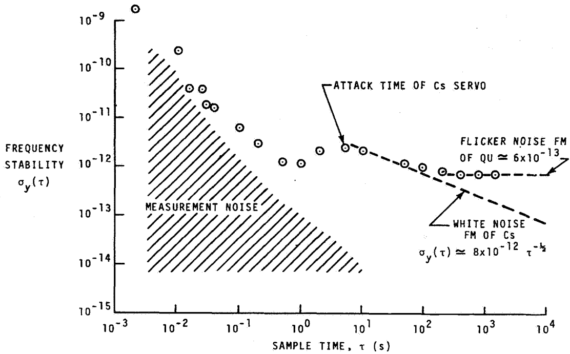
FIG.18 A \sigma_y(\tau) versus \tau plot of the fractional frequency fluctuations, y(t) between a high performance commercial cesium beam frequency standard and a commercial quartz crystal oscillator.
