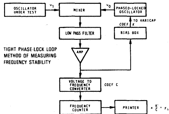
FIG. 3 A frequency fluctuation measurement system. The attack time of the phase lock loop in this case is much less than a second. The amplifier (AMP) output voltage fluctuations for sample times significantly larger than the servo loop attack time will be proportional to the frequency fluctuations between the oscillators.
