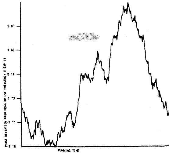
FIG 11 The residual time fluctuations between a high performance commercial cesium standard and one of the NBS primary frequency standards, NBS-5, after subtracting a mean frequency difference. The vertical scale is in units of 0.1 \mu\text{s} , and the abscissa shows 41100 s duration ( \sim 1/2 day). The peak-to-peak deviation is about 0.9 \mu\text{s} .
