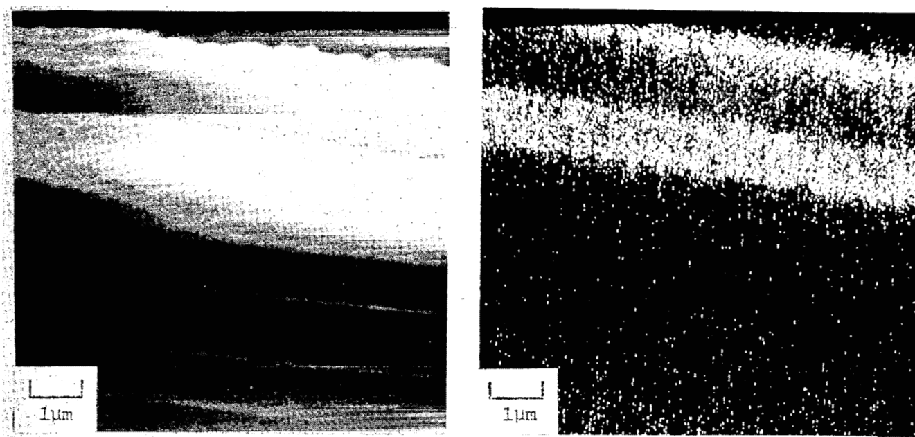
Fig. 7. SEM photomicrographs of Thornel 75 fiber wet-chemical-dipped three times with Ti solution; no coking heat-treatment between dips. (a) Specimen image, and (b) Ti x-ray image.
