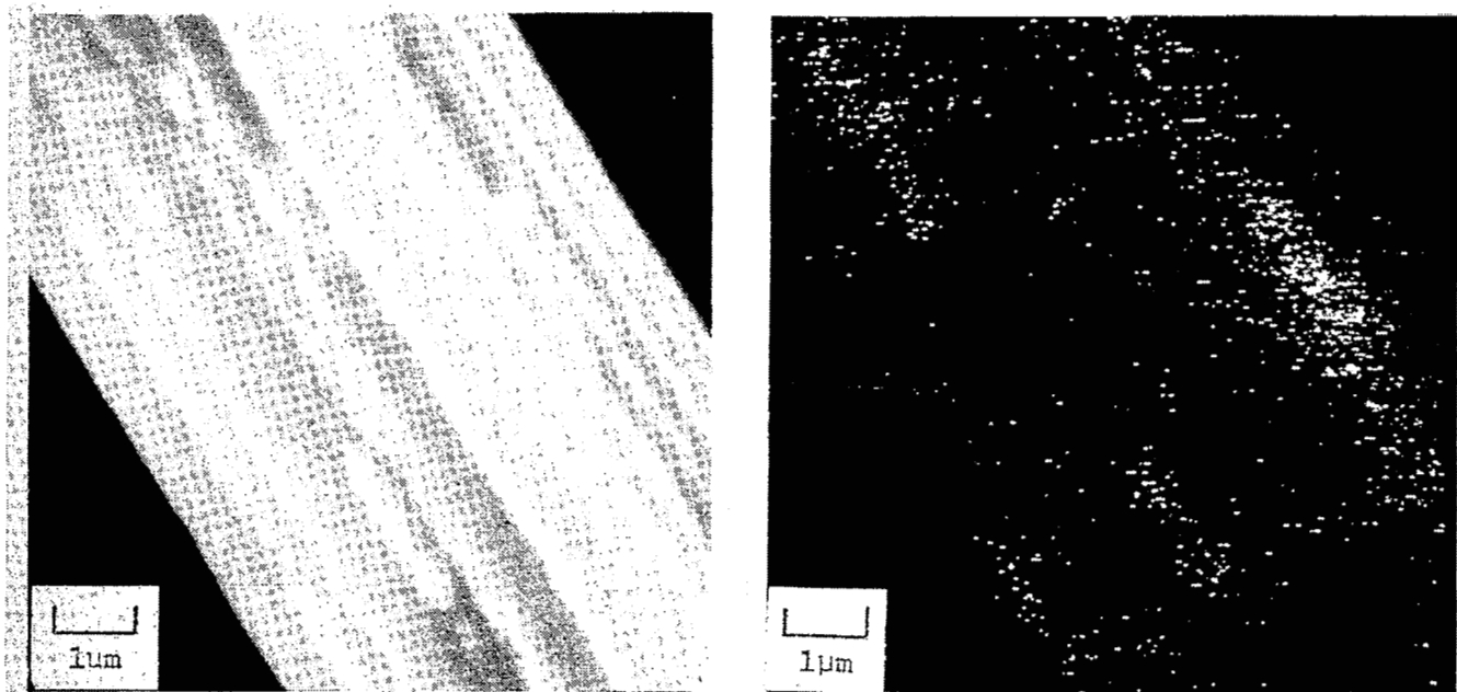
Fig. 8. SEM photomicrographs of Thornel 75 fiber wet-chemical-dipped three times with Ti solution; 1173 K (900°C) coking heat-treatment between dips. (a) Specimen image, and (b) Ti x-ray image.
