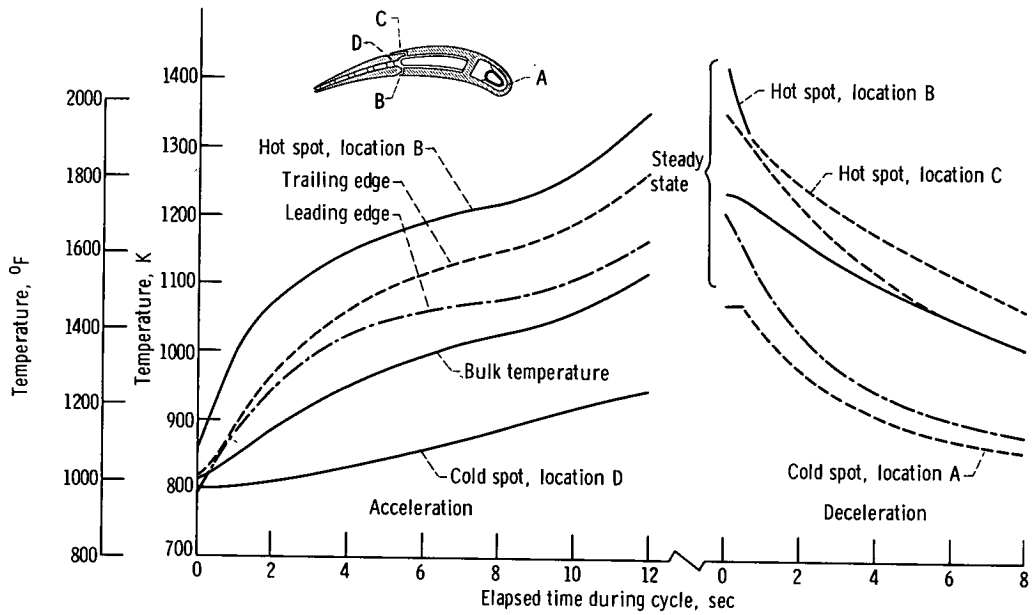
Figure 3. - Vane temperature response for case 1. Gas temperature range, 922 to 1644 K (1200 o to 2500 o F); coolant temperature, 811 K (1000 o F); gas and coolant inlet pressure, 31 N/cm 2 (45 psia); coolant- to gas-flow ratio, 0.035.
