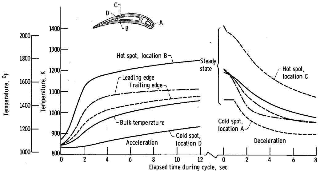
Figure 6. - Vane temperature response for case 4. Gas temperature range, 922 to 1644 K (1200 o to 2500 o F); coolant temperature, 811 K (1000 o F); gas and coolant inlet pressure, 31 N/cm 2 (45 psia); coolant- to gas-flow ratio, 0.075.
