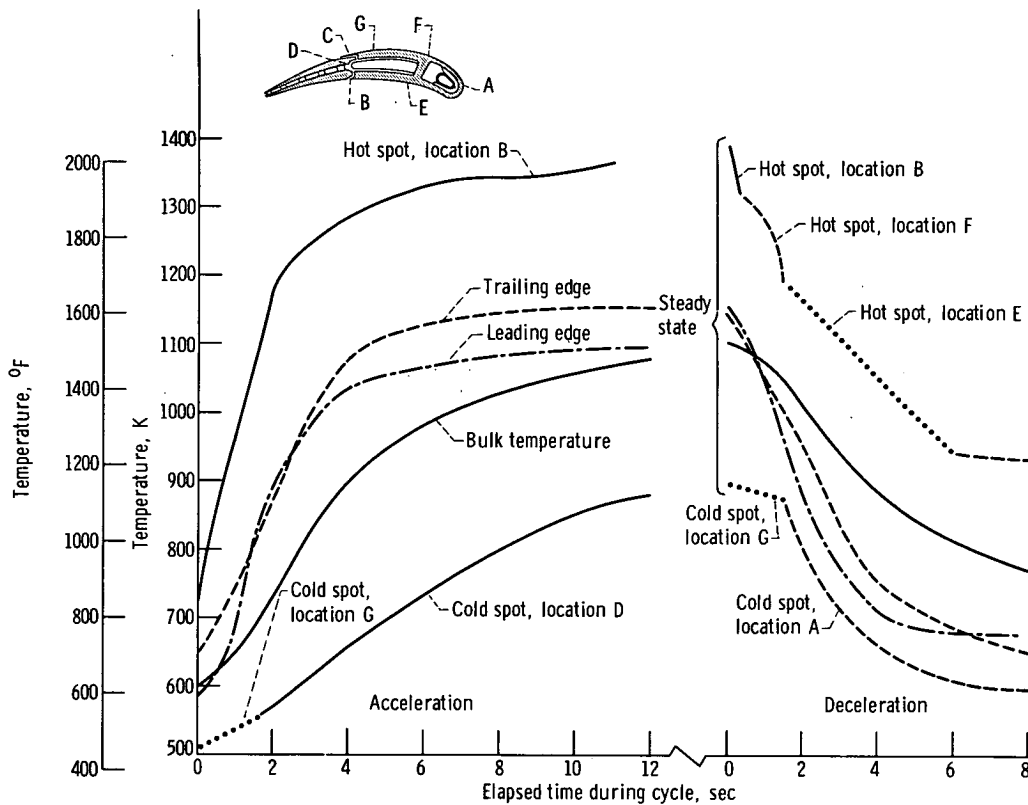
Figure 4. - Vane temperature response for case 2. Gas temperature range, 922 to 1644 K (1200 o to 2500 o F); coolant temperature, 300 K (80 o F); gas and coolant inlet pressure, 31 N/cm 2 (45 psia); coolant- to gas-flow ratio, 0.035.
