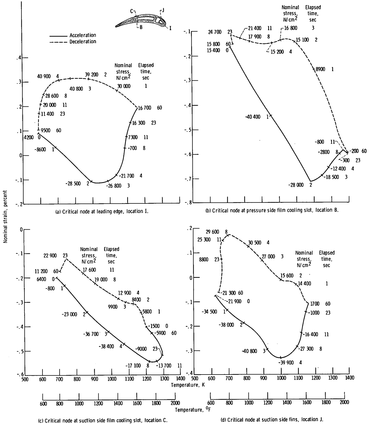
Figure 8. - Strain-temperature response of vane for case 2. Gas temperature range, 922 to 1644 K (1200 o to 2500 o F); coolant temperature, 300 K (80 o F); gas and coolant inlet pressure, 31 N/cm 2 (45 psia); coolant- to gas-flow ratio, 0.035; no hold time, fifth cycle.
