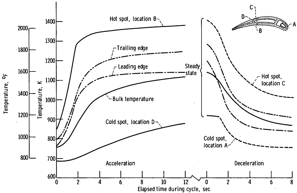
Figure 5. - Vane temperature response for case 3. Gas temperature range, 922 to 1644 K (1200 o to 2500 o F); coolant temperature, 589 K (600 o F); gas and coolant inlet pressure, 83 N/cm 2 (120 psia); coolant- to gas-flow ratio, 0.035.
