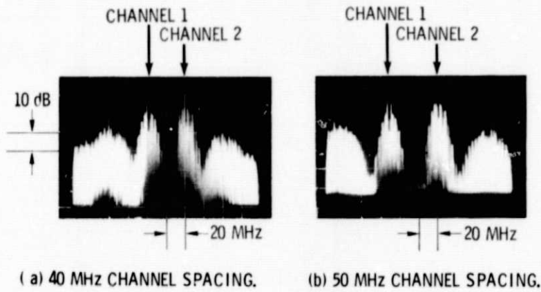
Figure 12. - Output spectrums for 18 MHz deviation, dual channel FM video signals.
