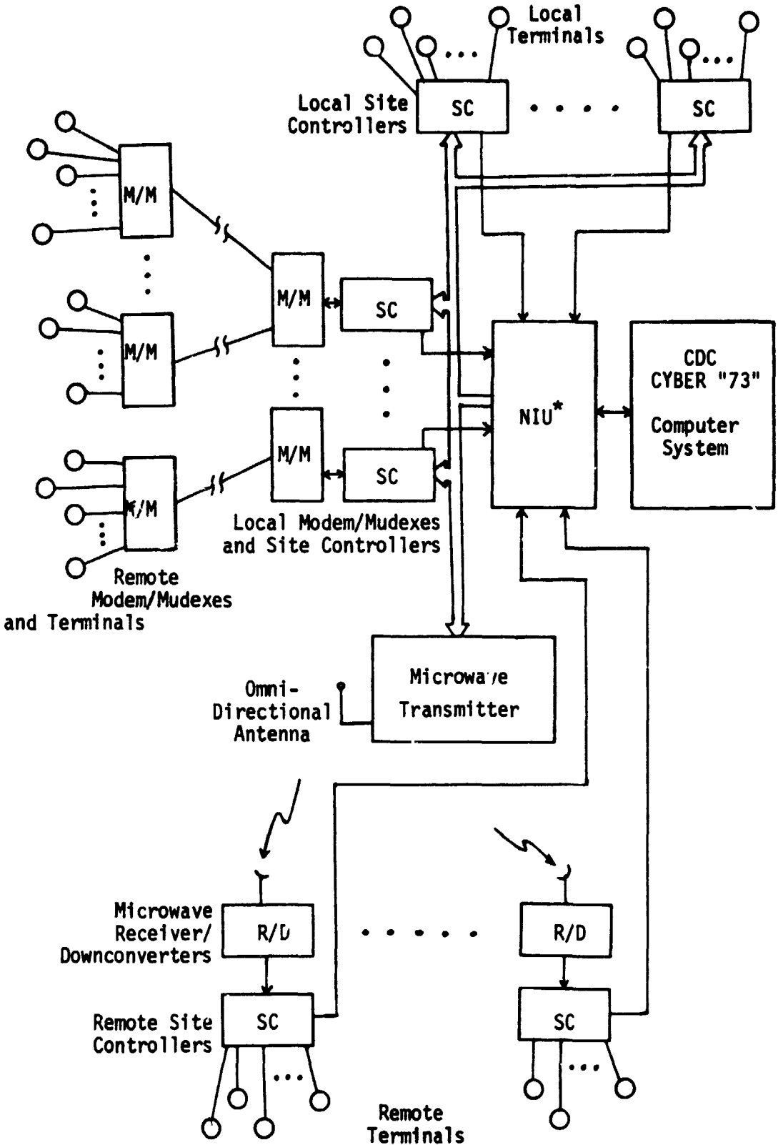
*Note: All lines into NIU are 4800B/S; those to SC's from NIU are 1.2MB/S Figure 2.2: Examples of Present PLATO IV Network (7)
