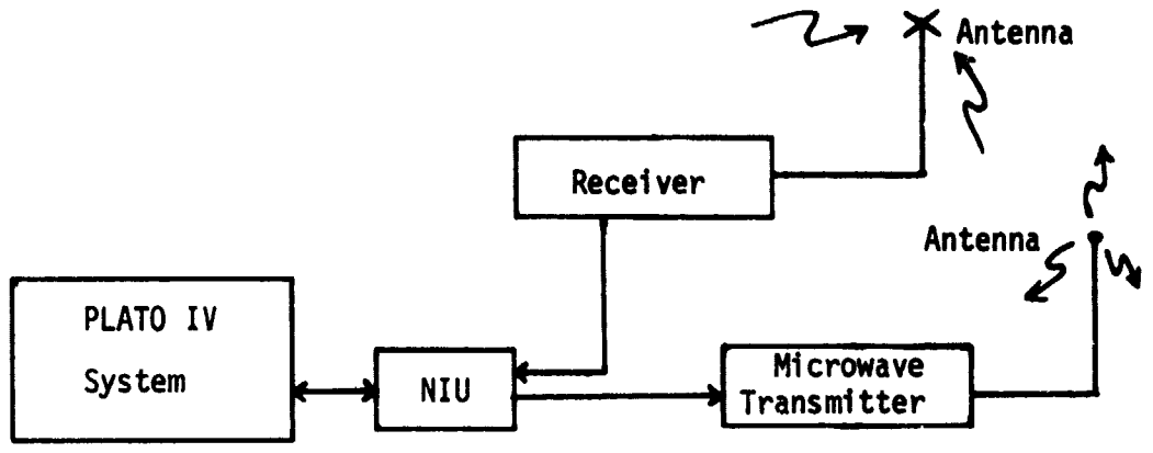
a) Computer site equipment
