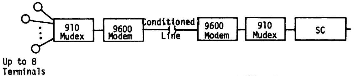
d) 9600B/S Modem and 910 muxer
