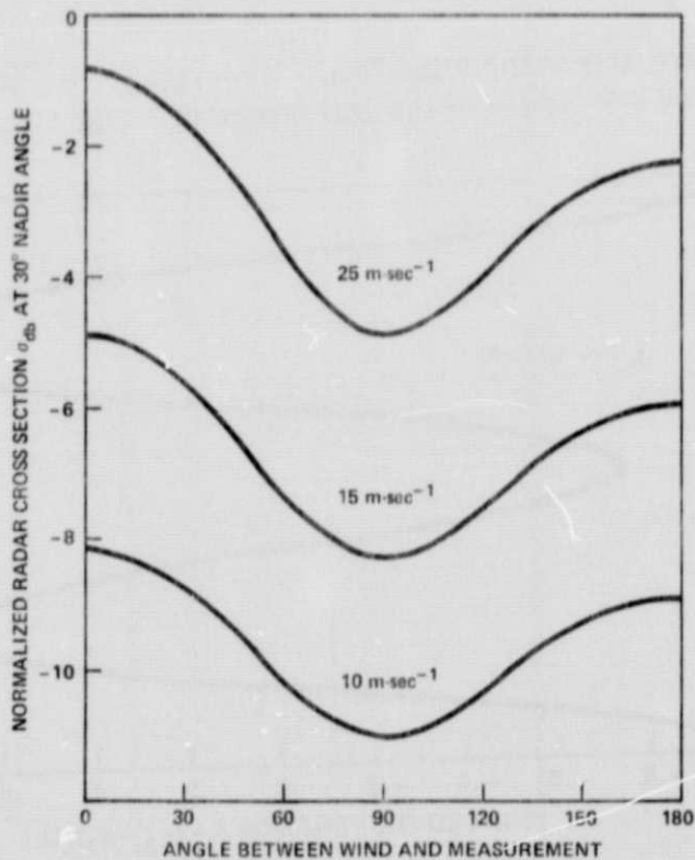
Figure 2. Variation of Radar Cross Section Versus Look Angle for Representative Values of Wind Speed. The Curves are Symmetric About 0^{\circ}
