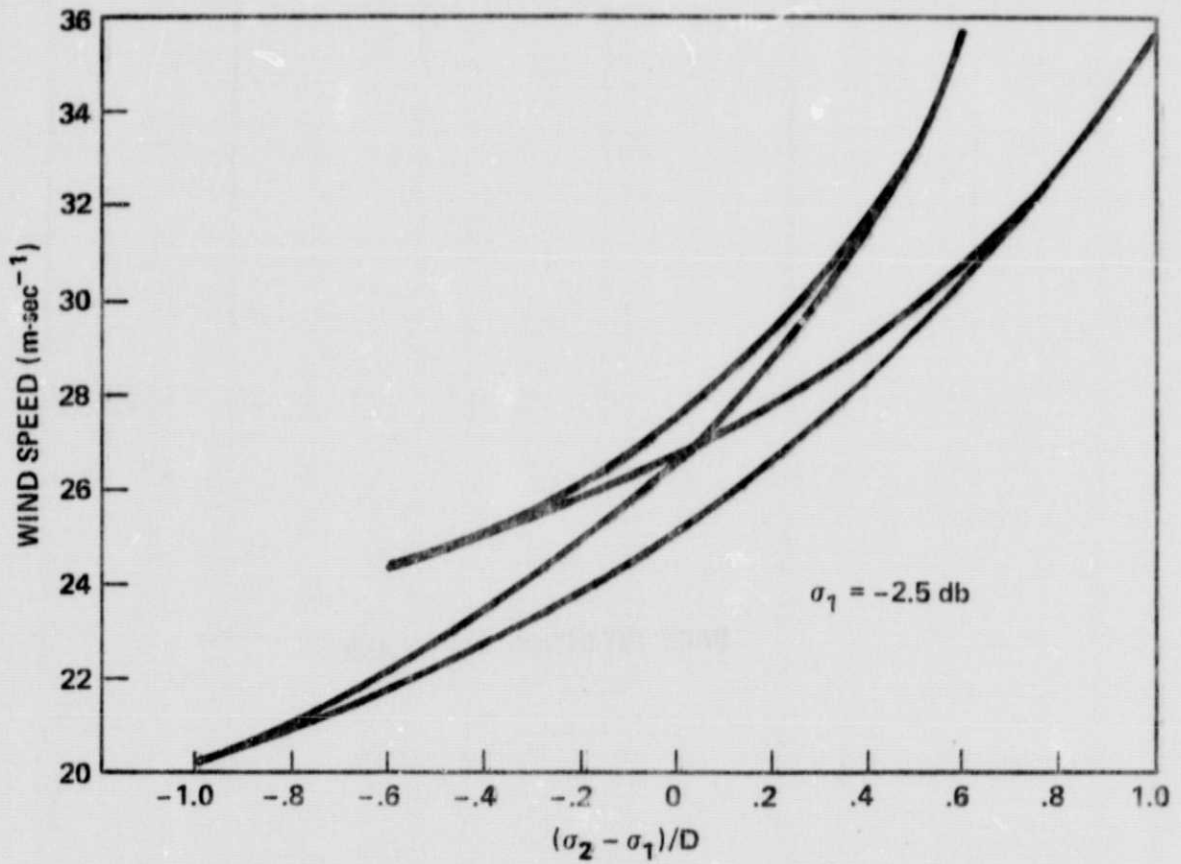
Figure 5. Solution Curve for Wind Speed for High Winds as a Function of the Difference in Radar Cross Sections
