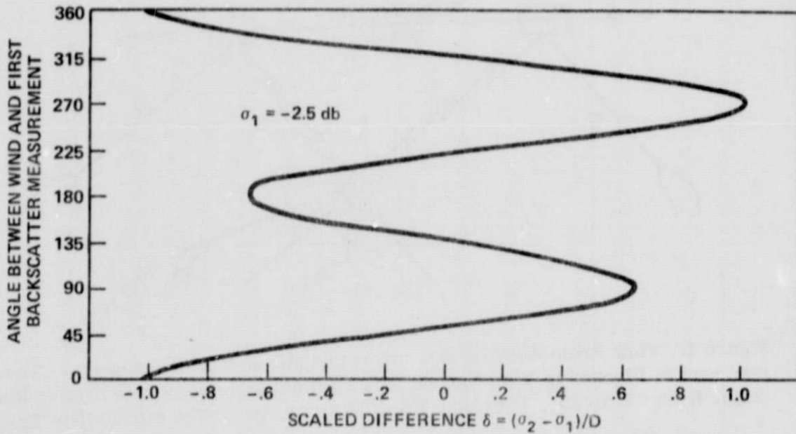
Figure 3. Solution Curve for Wind Angle Moderately High Winds ( \sigma_1 = -2.5 ) as a Function of the Difference in Radar Cross Sections
