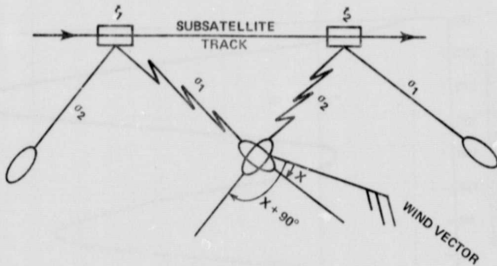
Figure 1. View From Above of Scatterometer Measurement Geometry. The Instrument is Planned to View Left as Well as Right (Shown), and to Scan in Nadir Angle from 25^{\circ} to 45^{\circ} , Providing Parallel Swaths Along the Subsattellite Track
