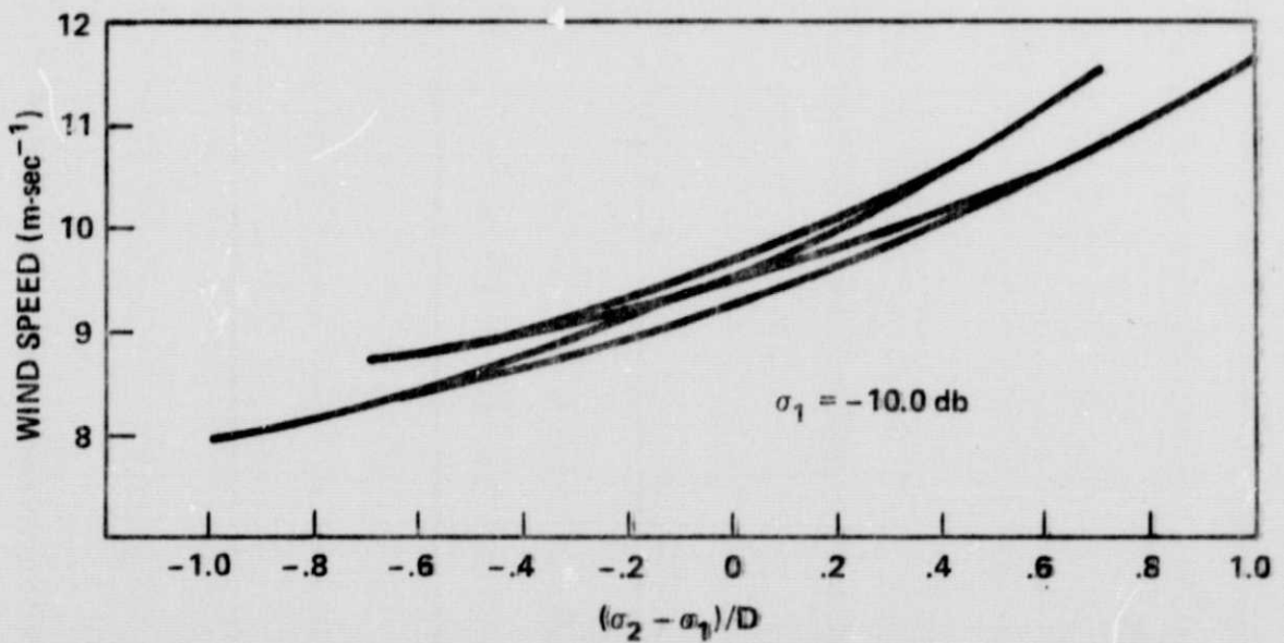
Figure 6. Solution Curve for Wind Speed at Low Winds ( \sigma_1 = -10.0 db)
