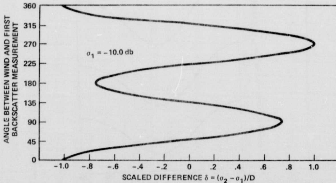
Figure 4. Solution Curve for Wind Angle for Low Wind Speed ( \sigma_1 = -10.0 ) as a Function of the Difference in Radar Cross Sections
