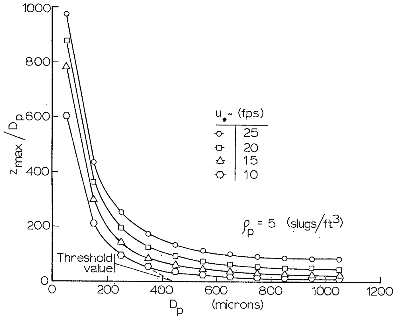
Figure 42. Normalized trajectory height for Mars, effect of friction speed (laminar sublayer)
