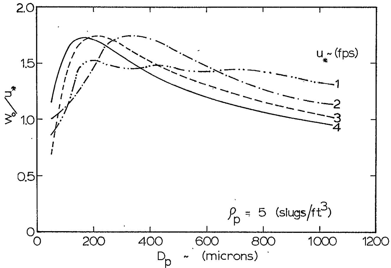
Figure 33. Maximum vertical velocity for Earth, effect of friction speed (laminar sublayer)
