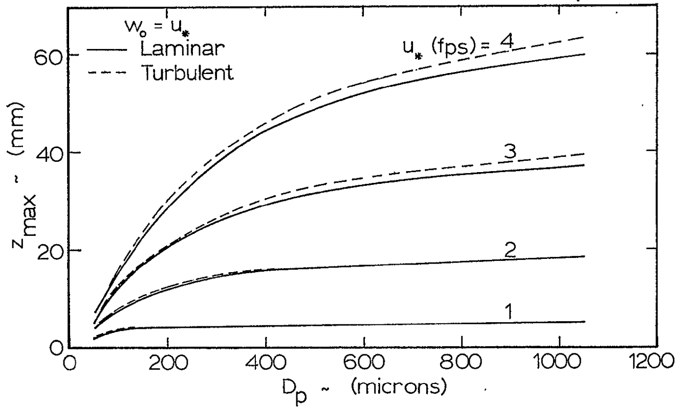
Figure 29. Maximum trajectory height for Earth, no lift, w_0 = u_*
