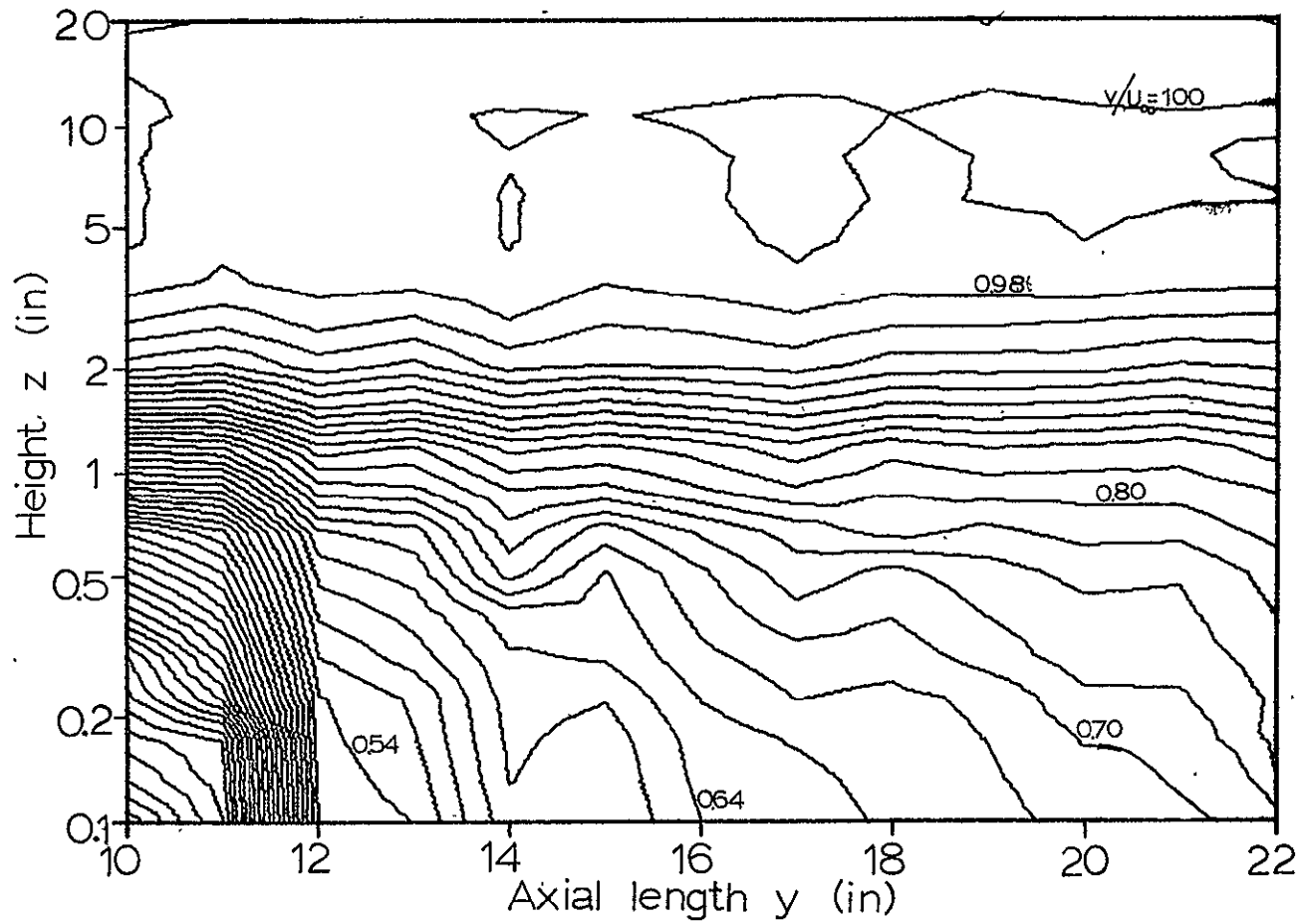
Figure 18. Crater wake longitudinal isotachs for x = 0 in.
