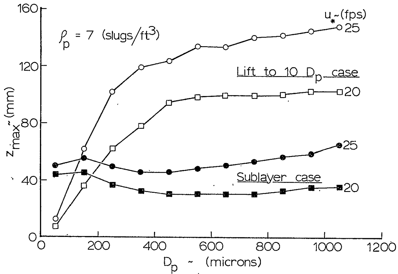
Figure 46. Maximum trajectory height for Mars, comparison of lift model
