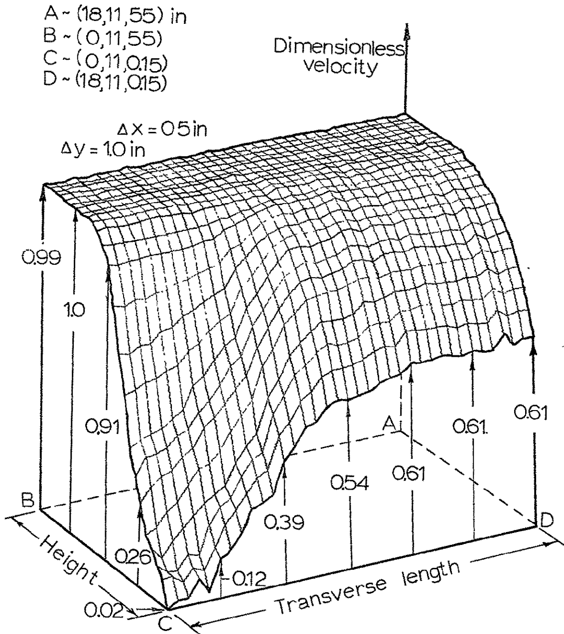
Figure 22. Crater wake velocity surfaces for y = 11 in.
