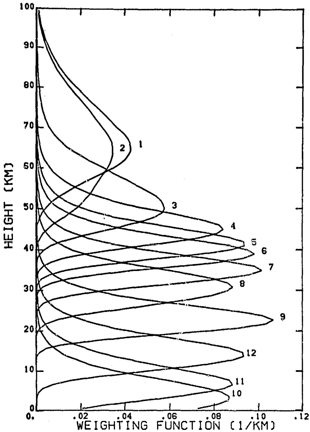
4.2(h) 53.5^\circ weighting functions, magnetic pole, circular polarization.
