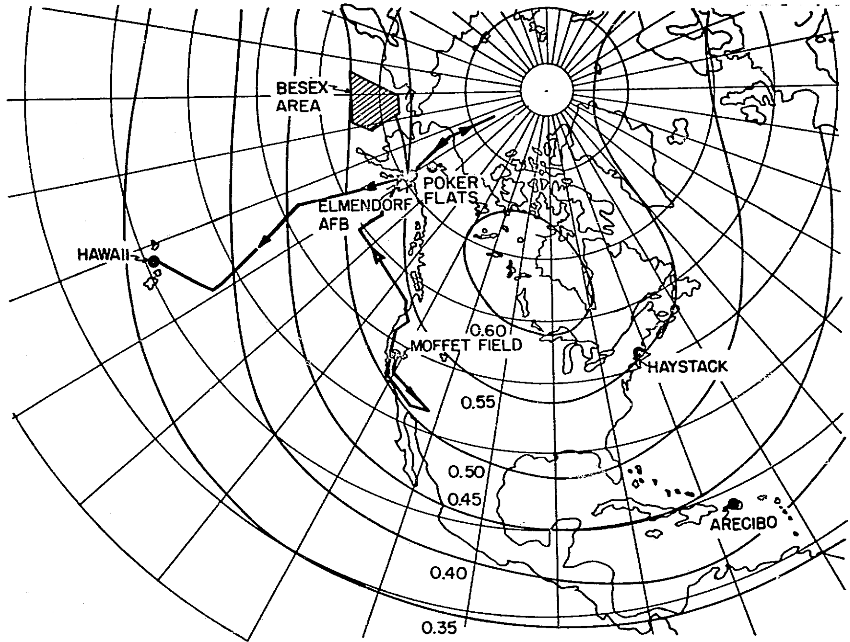
2.9 BESEX flights. Contours of the earth's magnetic field are also shown.
