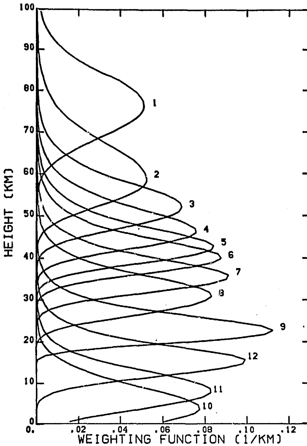
4.2(f) 53.5^\circ weighting functions, magnetic equator, circular polarization, looking east.
