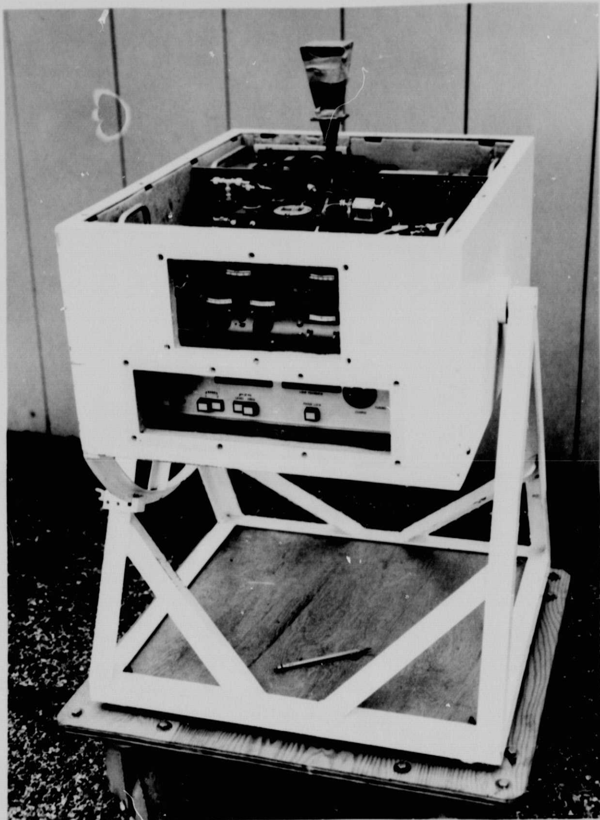
2.2 Radiometer and phase-lock box mounted in a tiltable box.
