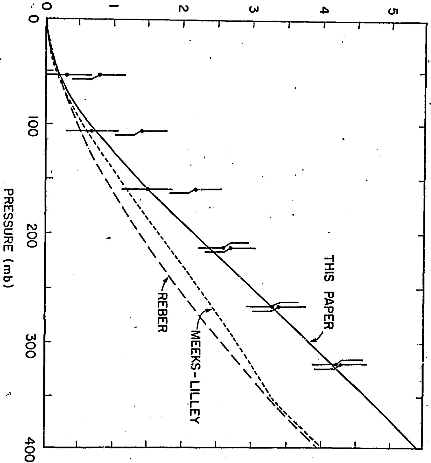
3.2 Absorption in dry air at 58.82 GHz and 295 K, computed for three models. Measurements are by Poon (1974).
