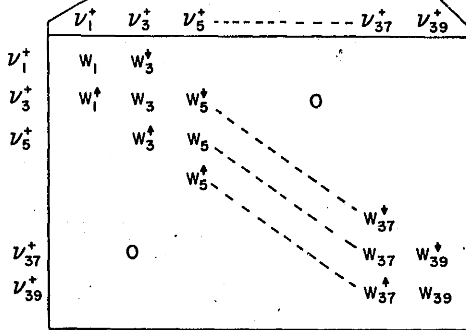
3.1 The W matrix. Elements associated with the zero frequency lines have been merged. The four shaded submatrices are alike.
