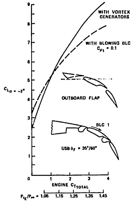
Fig. 19 Comparison of vortex generators with flap knee blowing BLC.
