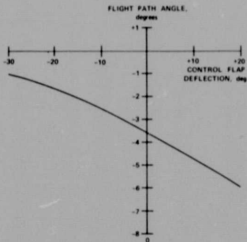
Fig. 14 Effect of control flap deflection on flight path angle: C_T = 1.0 , \delta_F = 82^\circ , W/S = 65 \text{ lb/ft}^2 , V = 70 knots.
