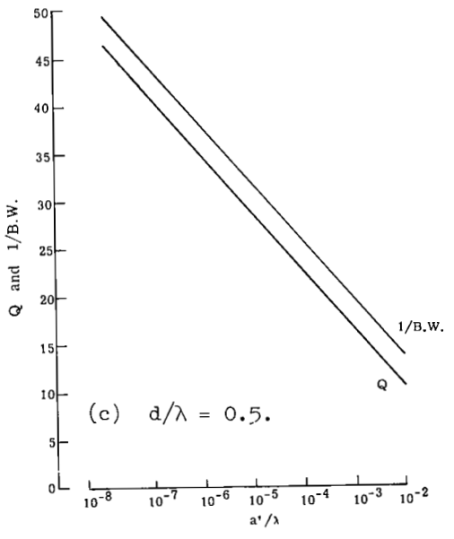
Figure 6.- Quality factor and reciprocal of relative bandwidth as a function of a'/\lambda for a/\lambda = 0.3 and b/\lambda = 0.6 .
