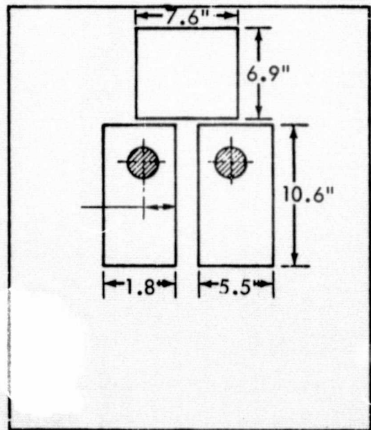
Launch Pad with Widened Nominal Holes
