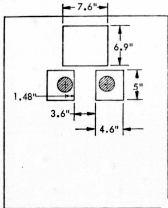
Launch Pad with Reduced Nominal Holes
