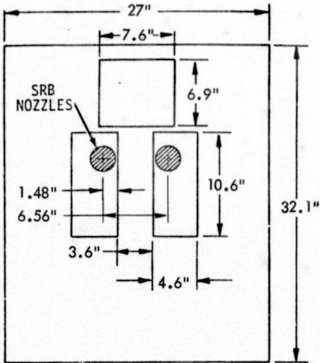
Launch Pad with Nominal Holes
