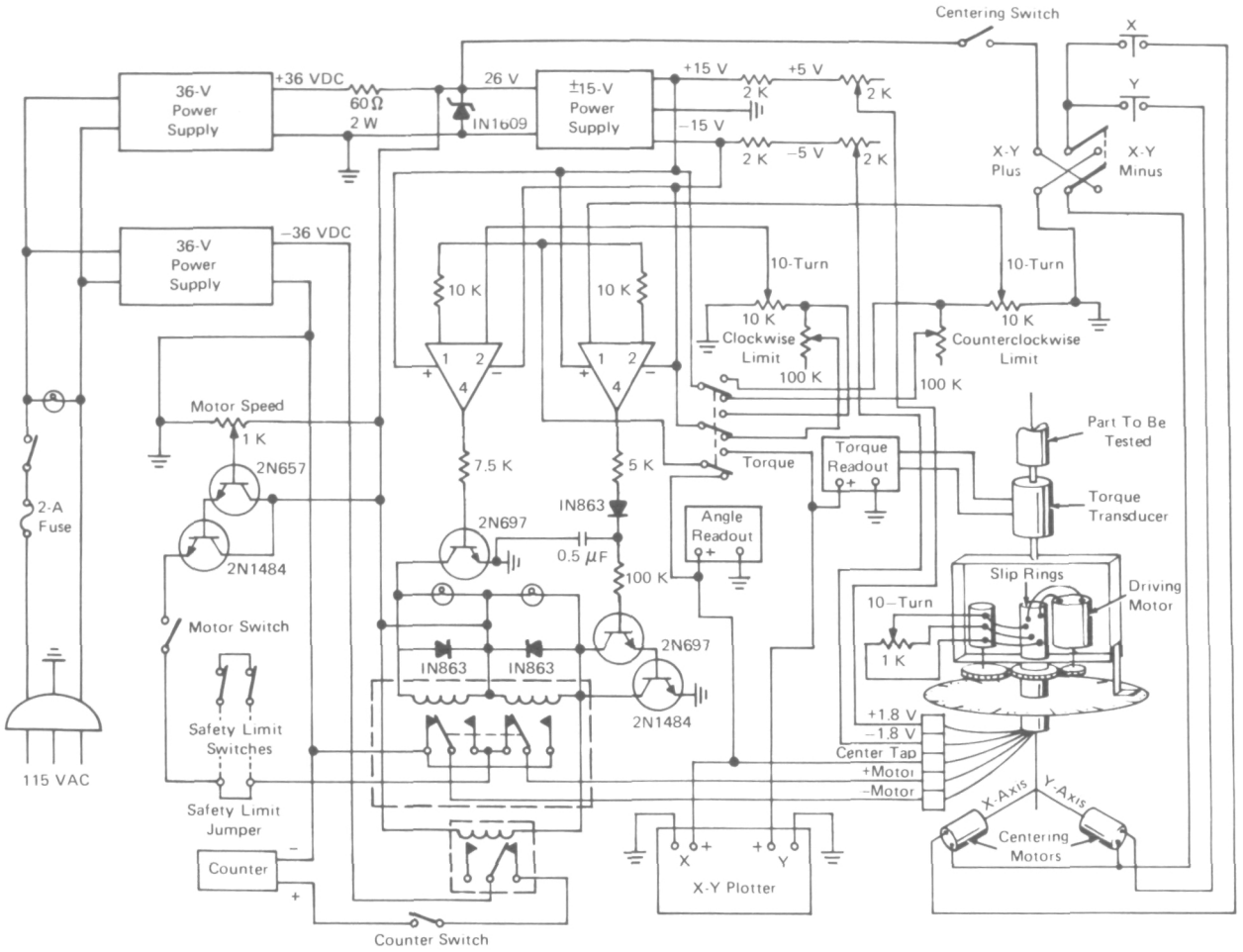
Torsion-Measuring System
