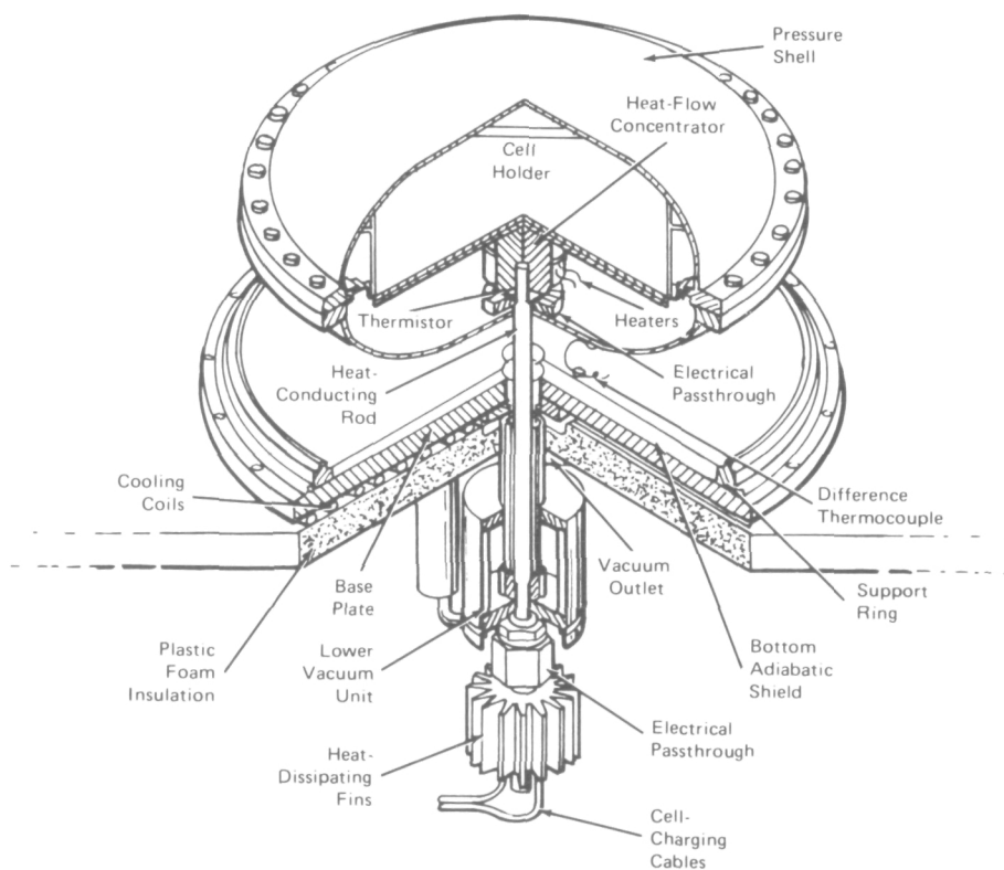
Figure 2. Quarter-Section Drawing of Calorimeter
