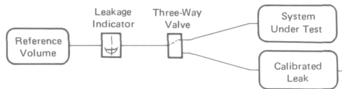
Leakage Indicator
