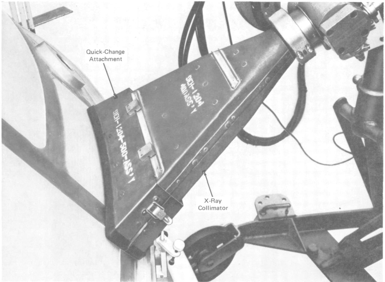
Radiographic-Collimator Attachment
