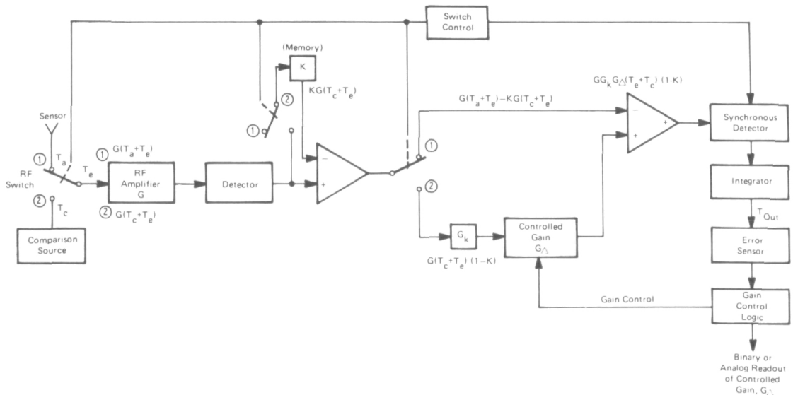
Figure 2. Self-Balancing Radiometer
