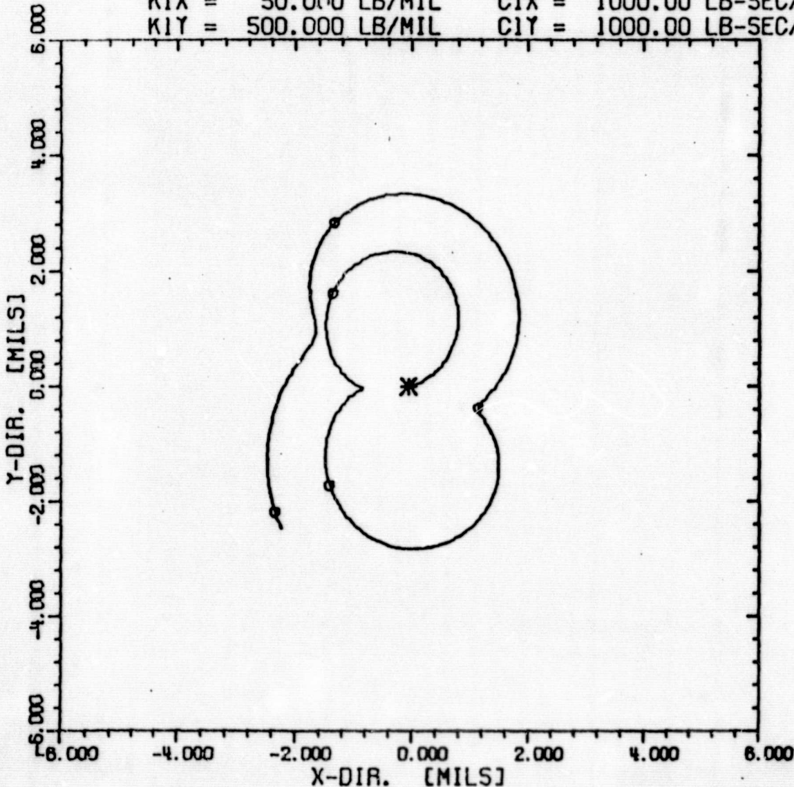
COMPRESSOR WITH HIGH AERODYNAMIC CROSS COUPLING-OPTIMUM DAMP - HIGH VERTICAL SUPPORT STIFFNESS -
