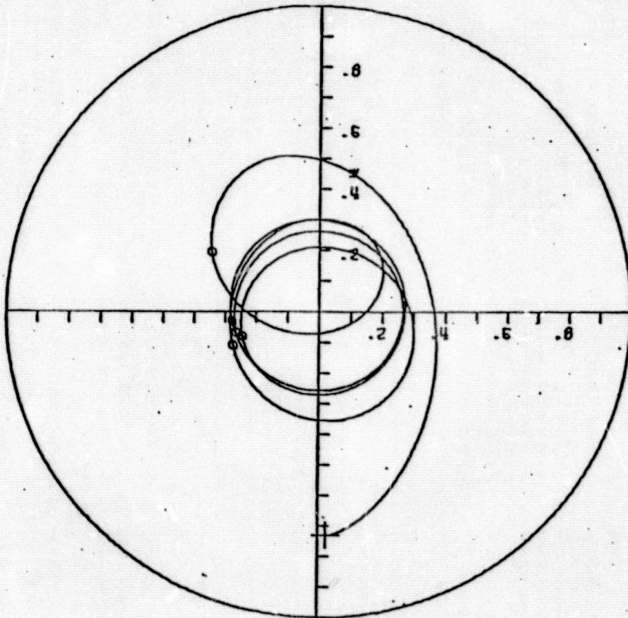
Figure 4-8 Vertical Unbalanced Rotor in Squeeze Film Bearing - Effect of Unbalance Magnitude - Unbalance Eccentricity = 1.75 Mils
