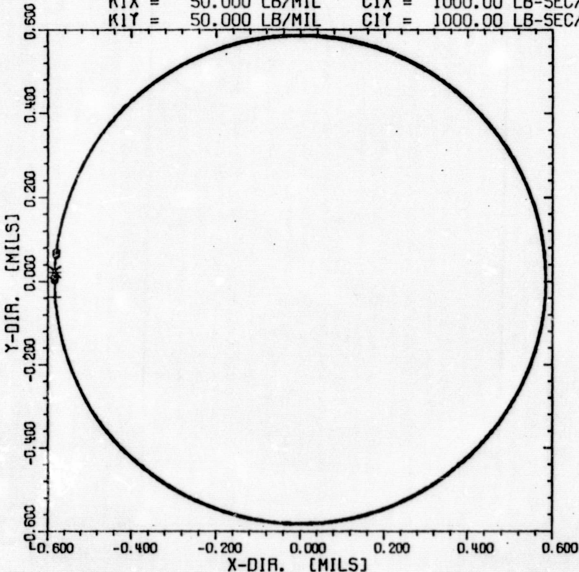
COMPRESSOR WITH HIGH AERODYNAMIC CROSS COUPLING-OPTIMUM DAMPING - LOW SUPPORT STIFFNESS -
