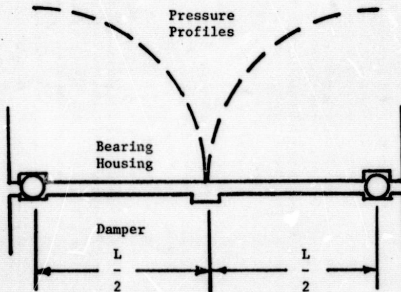
b. Damper with Circumferential Oil Groove and Flexible "O" Ring End Seals
