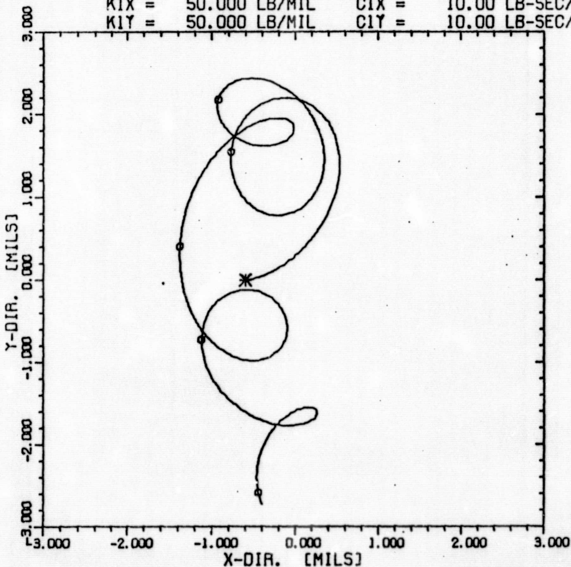
COMPRESSOR WITH LOW AERODYNAMIC CROSS COUPLING-UNDERDAMPED SUPPORT - UNSTABLE SYSTEM -
