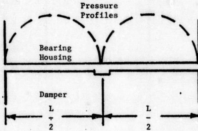
a. Damper with Circumferential Oil Groove
