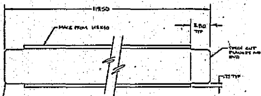
-011 DETAIL (5 REQD) MATERIAL ASTM A36 STEEL -W8x40
