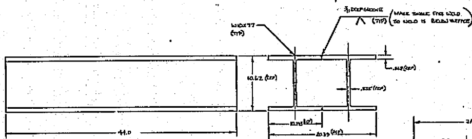
-COIL ASSY - 4 REQD MATERIAL: ASTM A 36 STEEL
