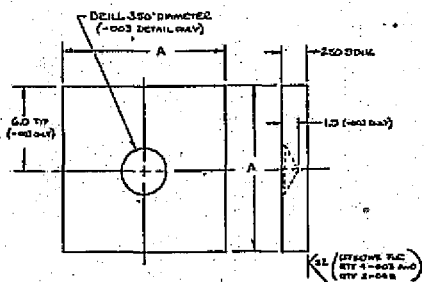
-003 DETAIL A = 12.0 (4 REQD) -004 DETAIL A = 15.0 (1 REQD) -007 DETAIL A = 16.0 (1 REQD) -008 DETAIL A = 12.0 (4 REQD)
