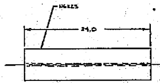
-COIL DETAIL - 8 REQD MATERIAL: ASTM A 36 STEEL
