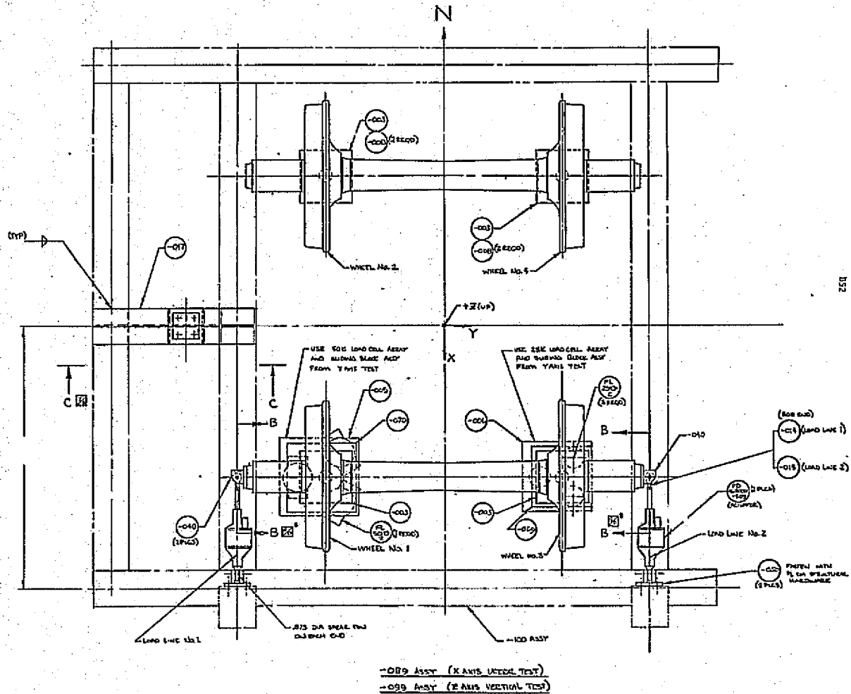
FIGURE 7.5 TEST FIXTURES
