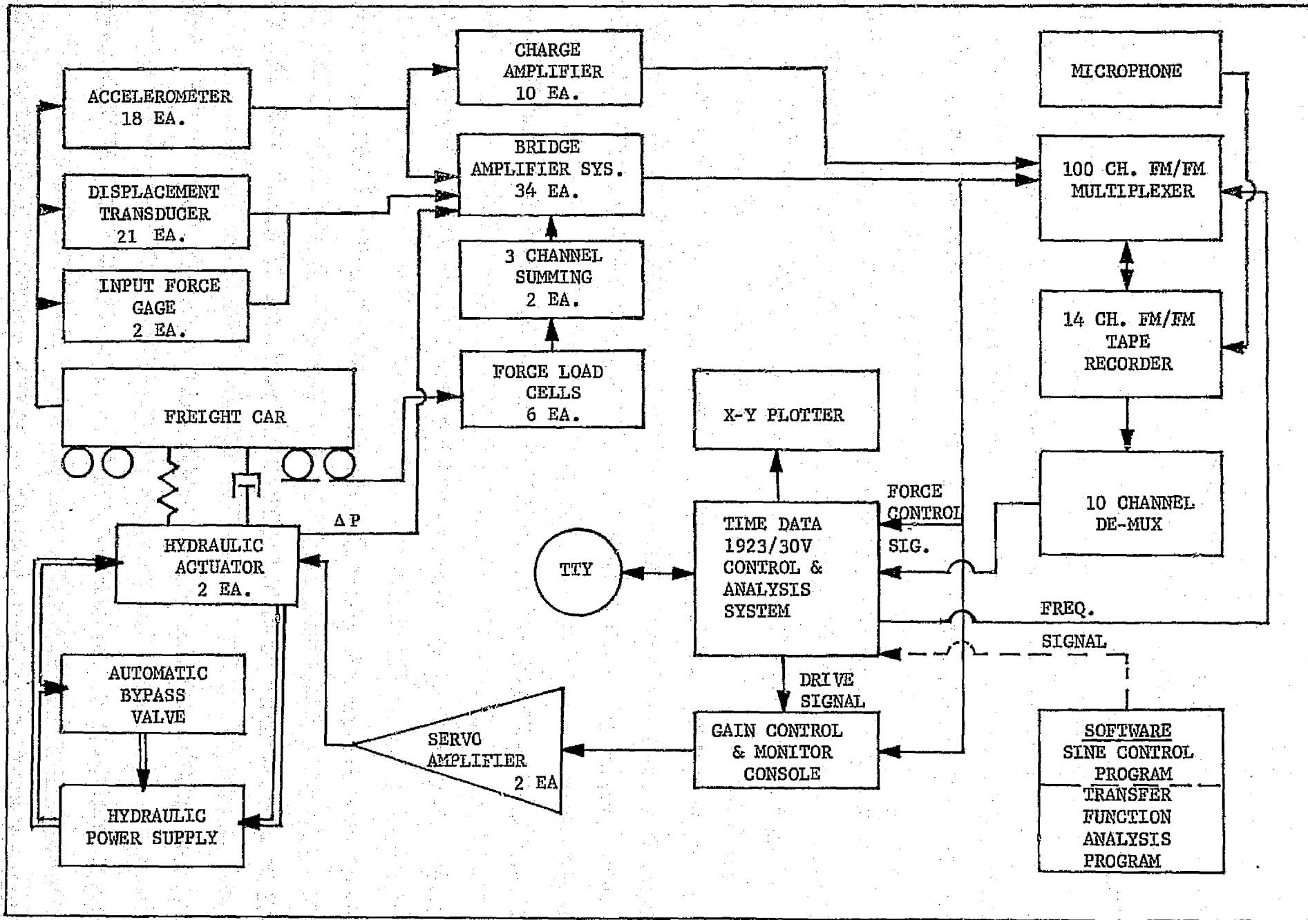
R FIGURE 7.4 TEST INSTRUMENTATION & CONTROL SYSTEM BLOCK DIAGRAM
