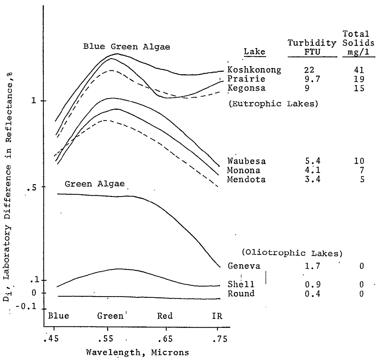
FIGURE 4 - Laboratory Difference in Reflectance Curves, D_i , for different non-tannin water samples with various amounts of algae. D_i = Laboratory Apparant Reflectance of Sample minus Reflectance for Distilled water. The more the algae the higher the curve and the eutrophic the lake.
