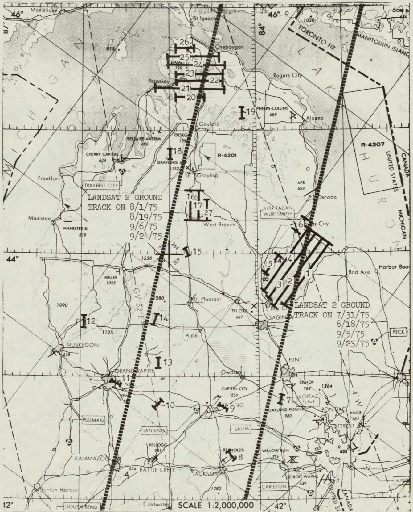
Figure 2. Flight lines for scheduled aircraft coverage of Saginaw Bay and inland test lakes by NASA JSC.
