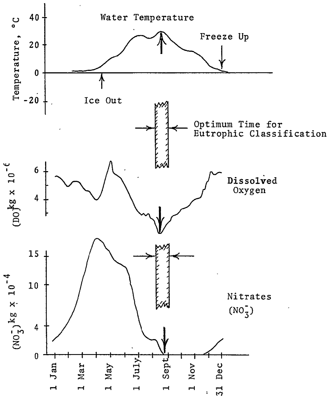
Figure 2 . Water Temperature, Dissolved Oxygen, and Nitrates (Algal Nutrients) Plotted Against Time. Lake Mendota, 1971.
