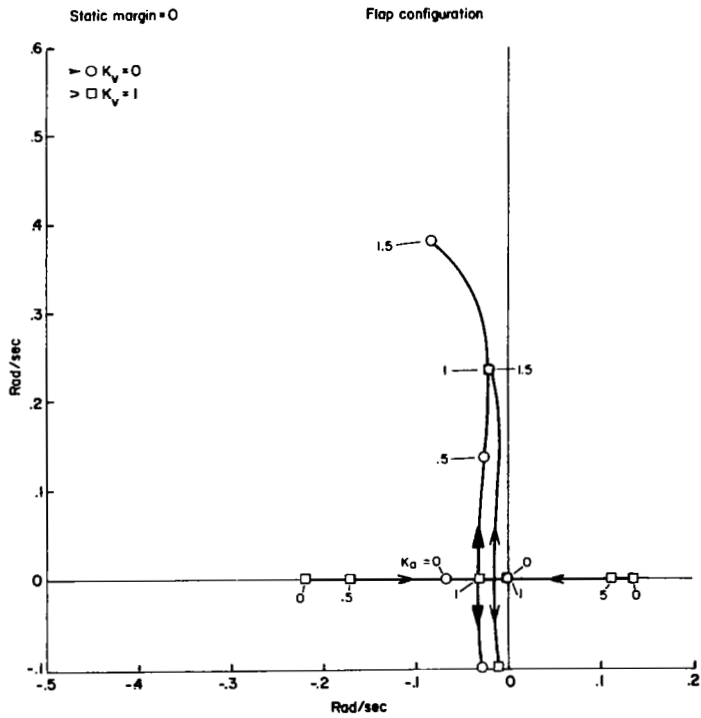
Figure 2 Root Locus of Flap-Configured Aircraft as a Function of Vertical Gust Alleviation Gain
