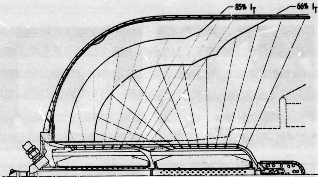
Fig. 10. Quench Impingement Patterns
