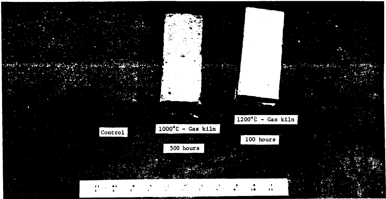
Figure 7. - Irish Refrasil fiber cake samples.
