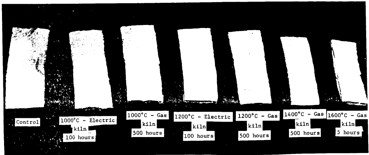
Figure 14.- Kaowool 1400 blanket samples.
