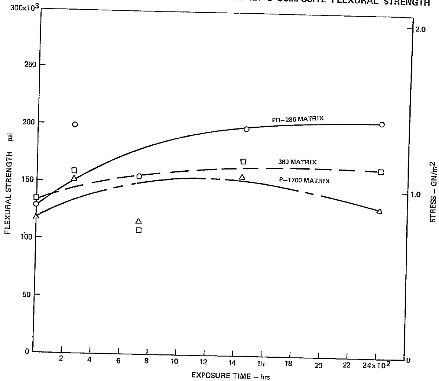
EFFECT OF R.H. AND U.V. AND TEMP. ON 121°C COMPOSITE FLEXURAL STRENGTH
