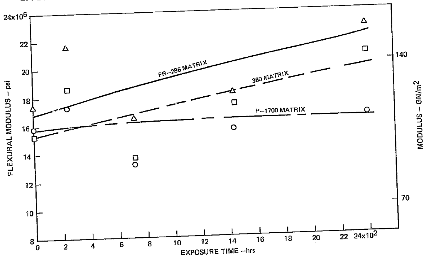
EFFECT OF R.H. AND U.V. AND TEMPERATURE ON 121°C COMPOSITE FLEXURAL MODULUS
