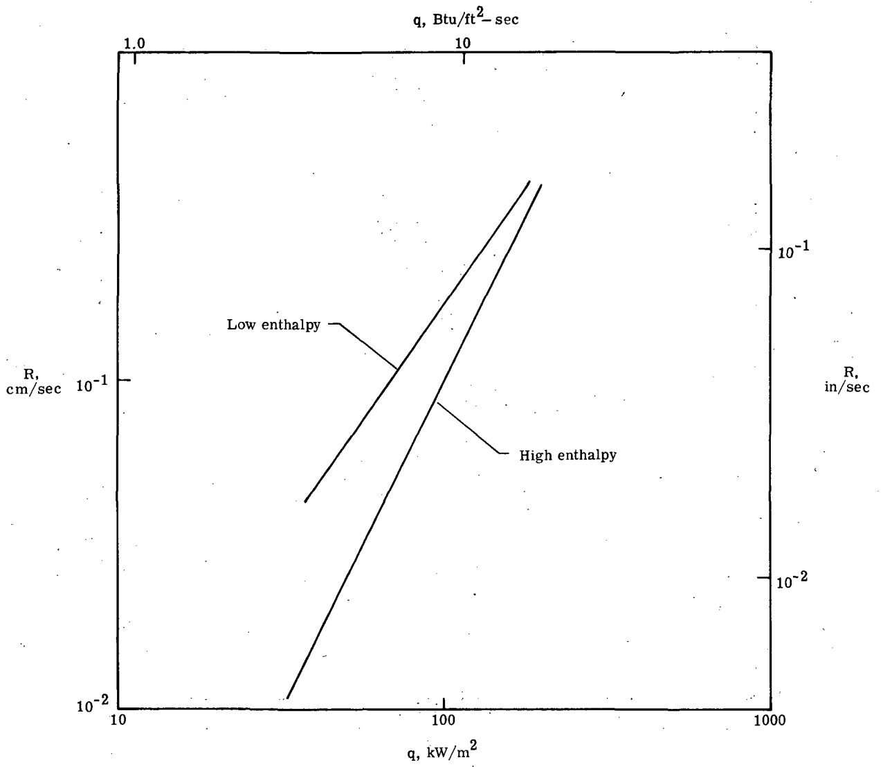
Figure 10.- High and low enthalpy curves.
