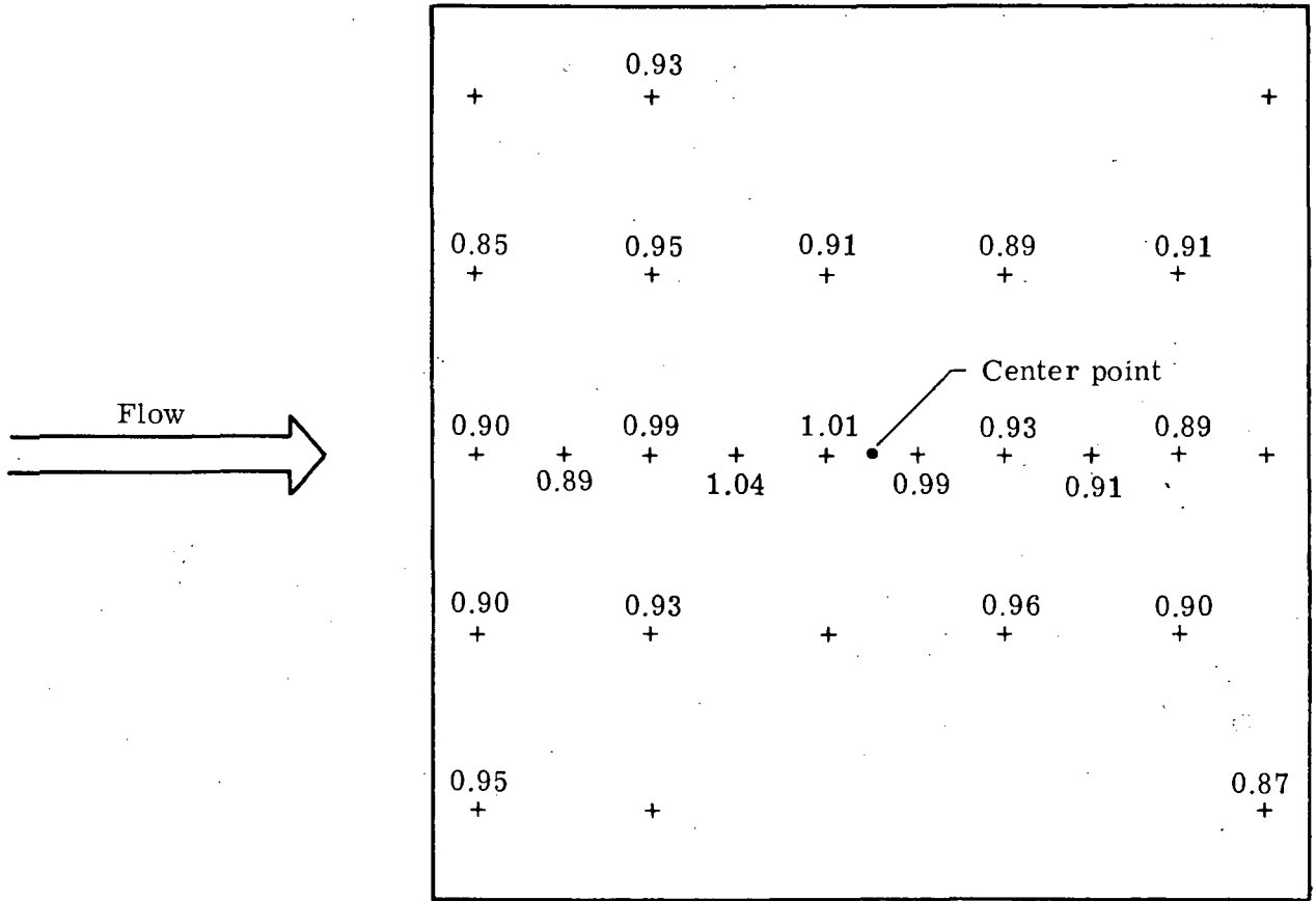
Figure 4.- Typical heating rate distribution (normalized to center point) for high enthalpy tests. Drawn to scale.
