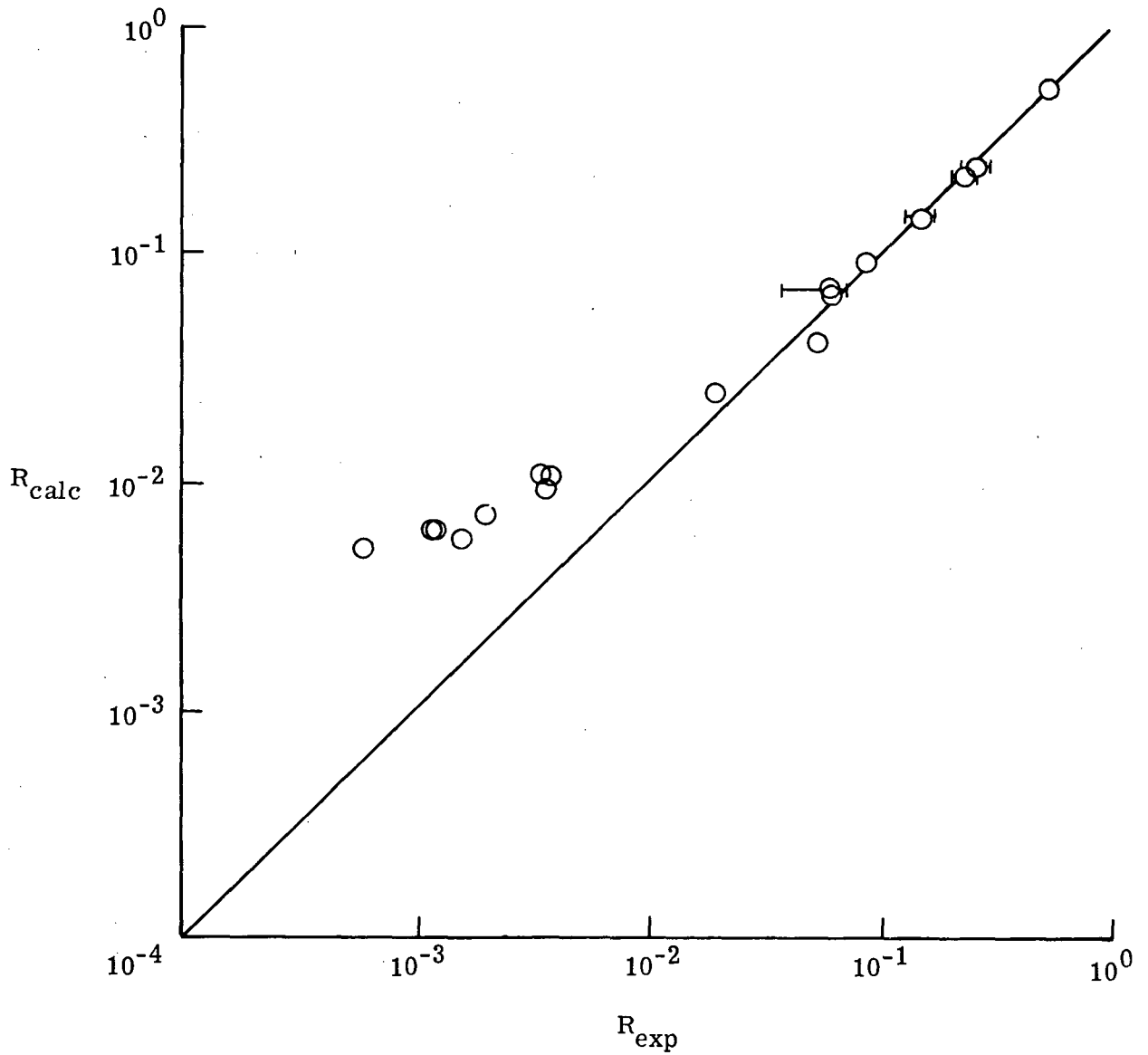
Figure 14.- Data correlation of calculated and experimental recession rates including subsonic, high pressure data. Weighted.
