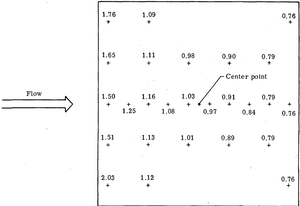
Figure 5.- Typical heating rate distribution (normalized to center point) for low enthalpy tests. Drawn to scale.
