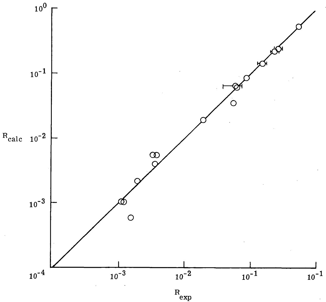
Figure 15.- Data correlation of calculated and experimental recession rates including subsonic, high pressure data. Weighted and modified.
