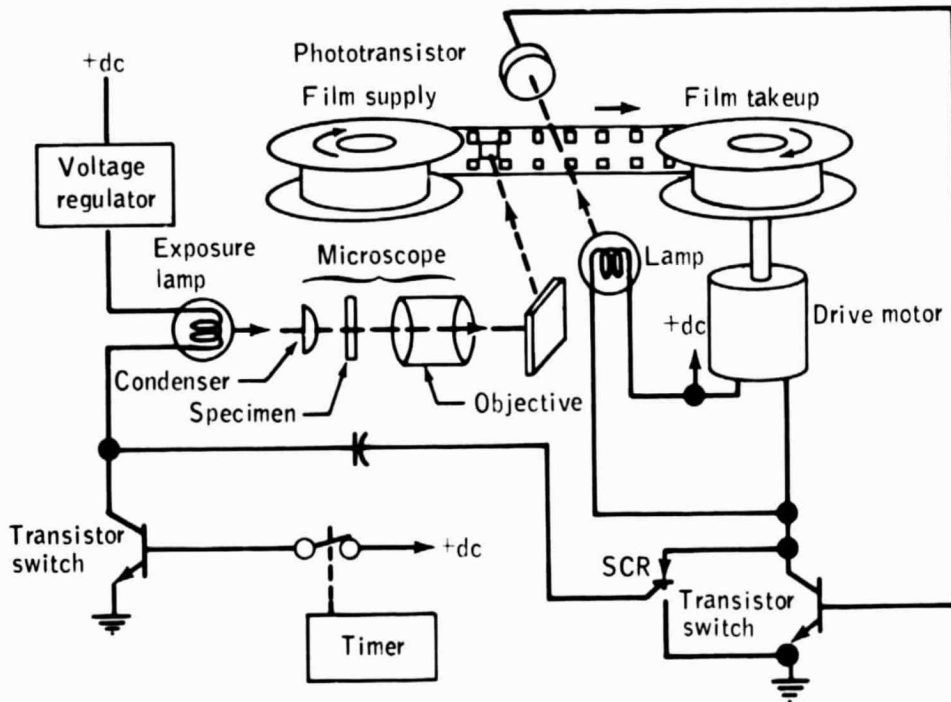
Figure 8.- Camera-microscope diagram.
