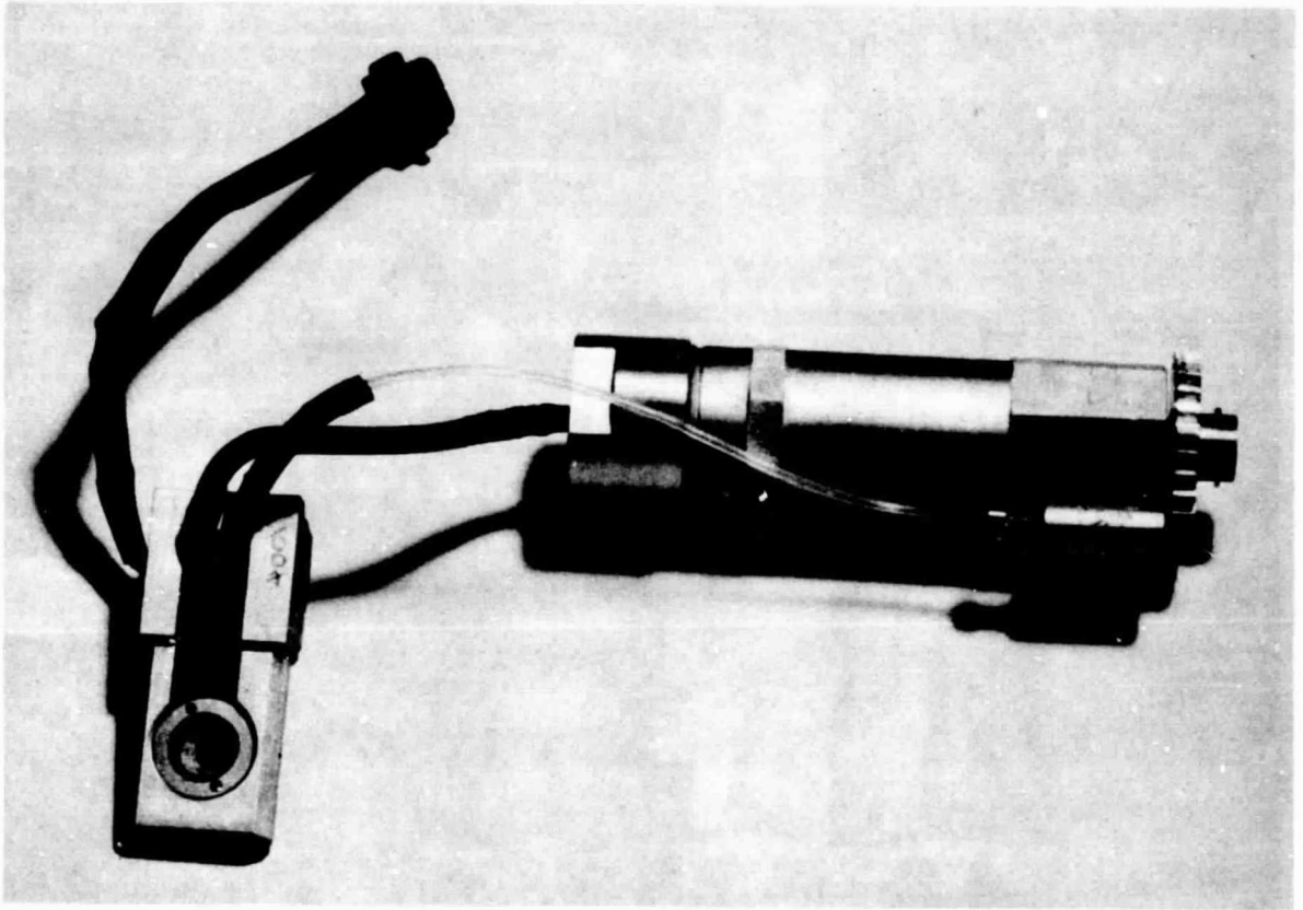
Figure 9.- Microscope pump/chamber assembly.
