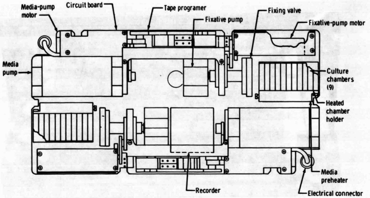
Figure 5.- Growth curve module.
