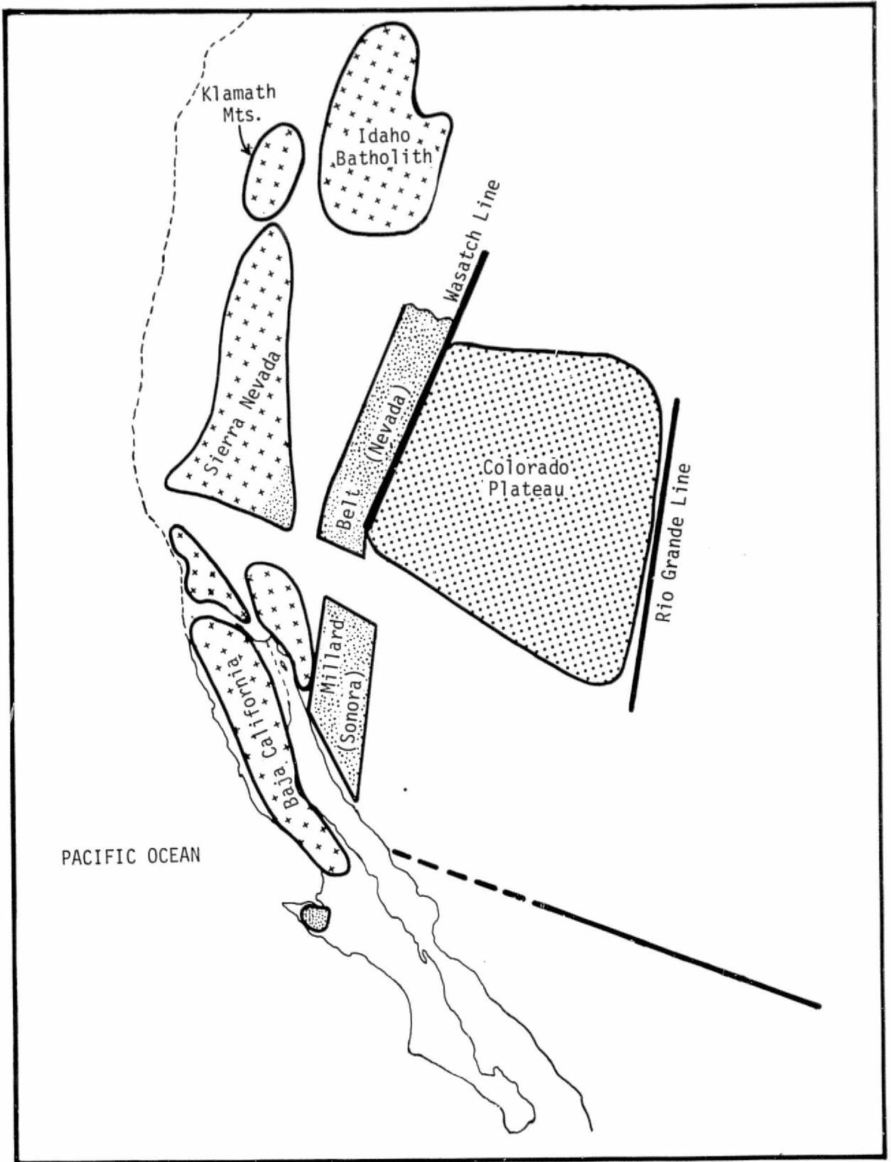
FIGURE 26 RECONSTRUCTION MODEL FOR SELECTED BLOCKS IN WESTERN CORDILLERA
