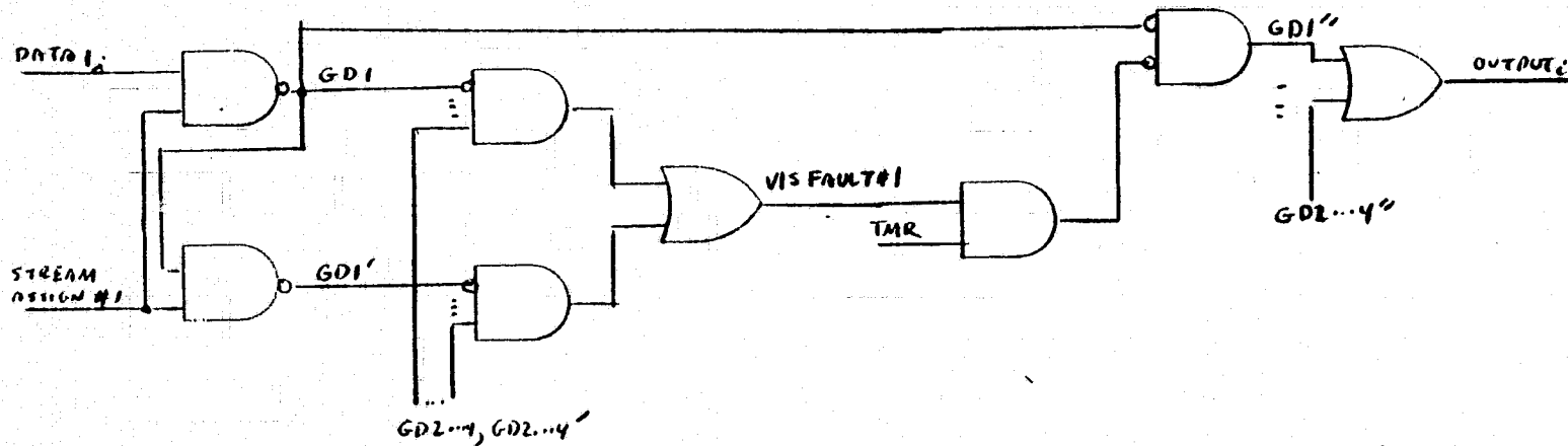
MEMORY VOTER / SWITCH WITH FAULT DETECTION (10 DIPS/BIT)
