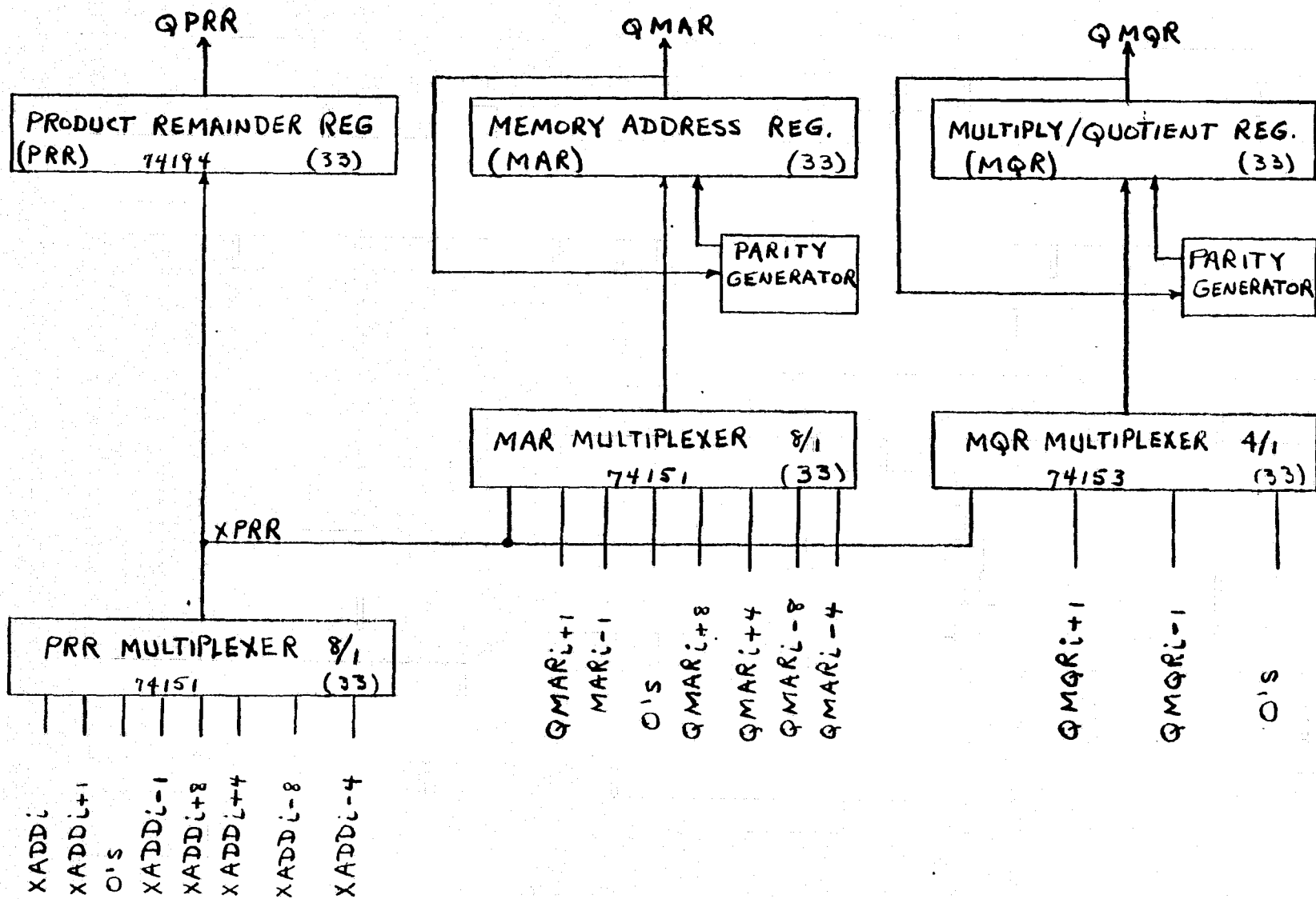
Figure 4-13 PRR - MAR - MQR REGISTERS
