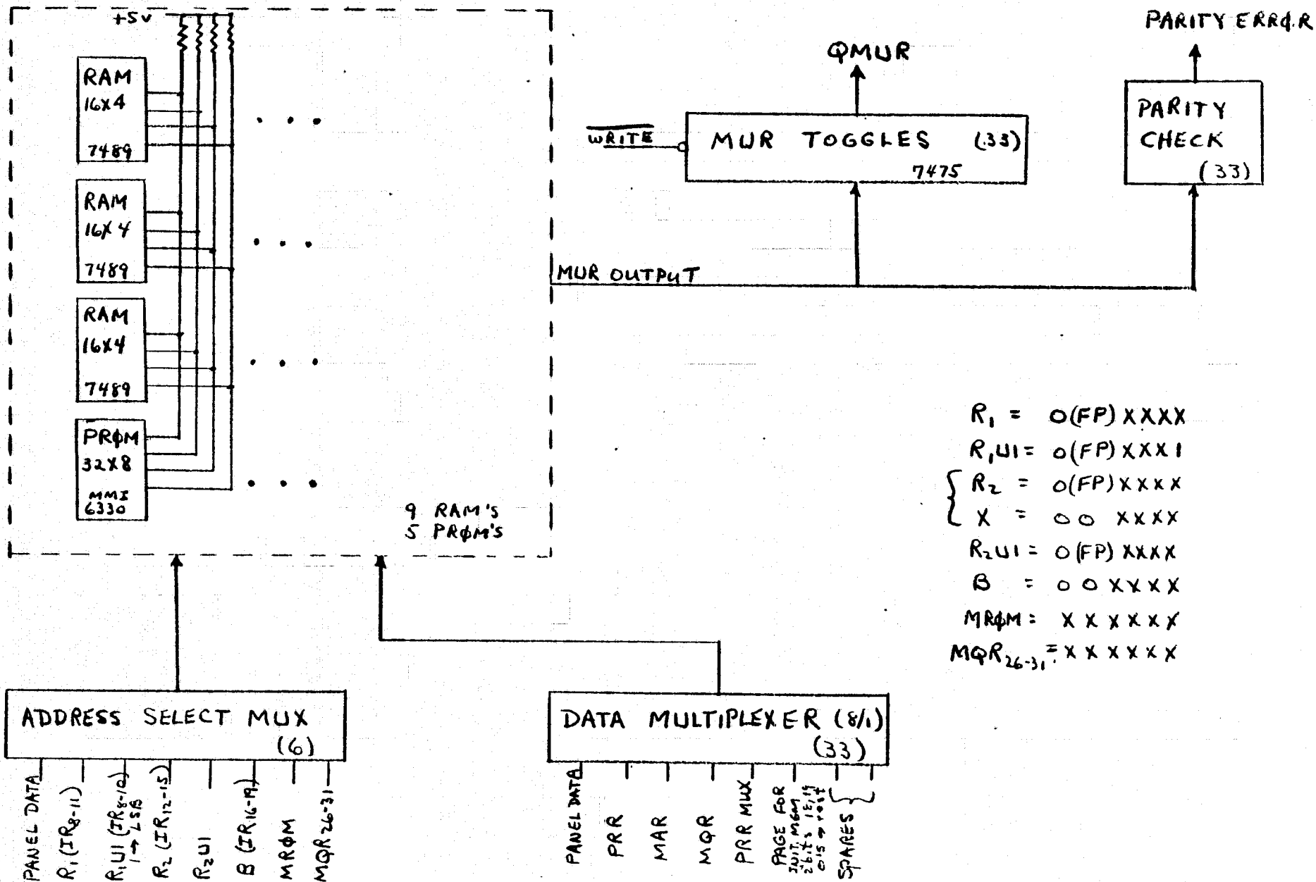
Figure 4-11 MULTIPLE-USAGE REGISTERS (MUR)
