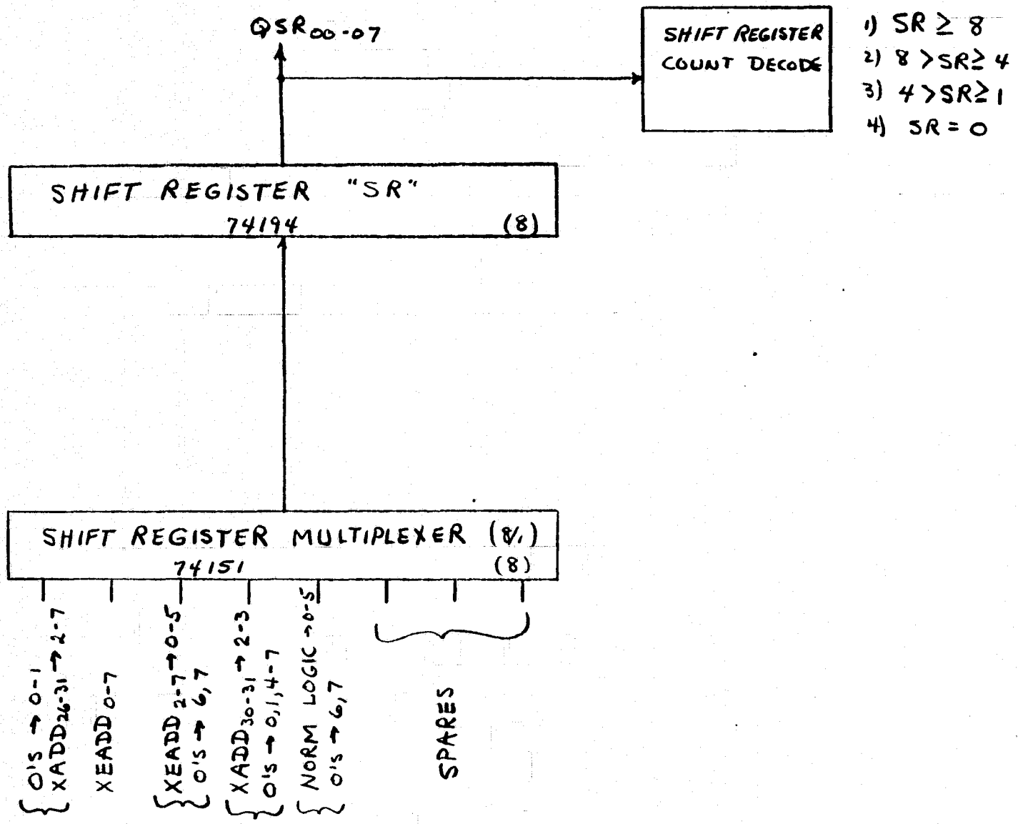
Figure 4-5 SHIFT REGISTER
