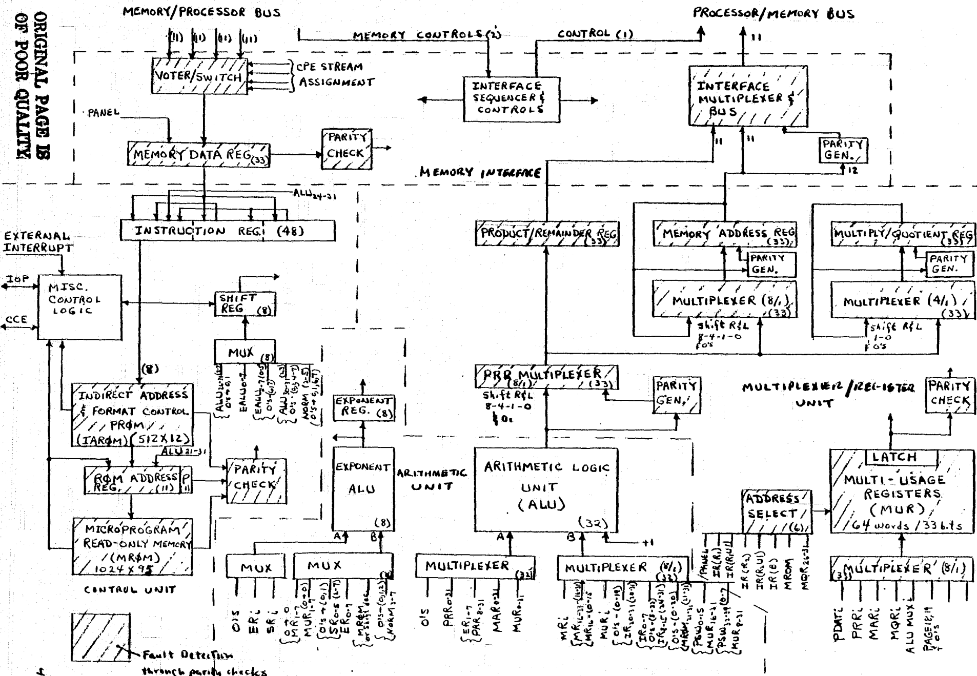
Figure 4-2 CENTRAL PROCESSING ELEMENT (CPE) BLO. DIAGRAM
