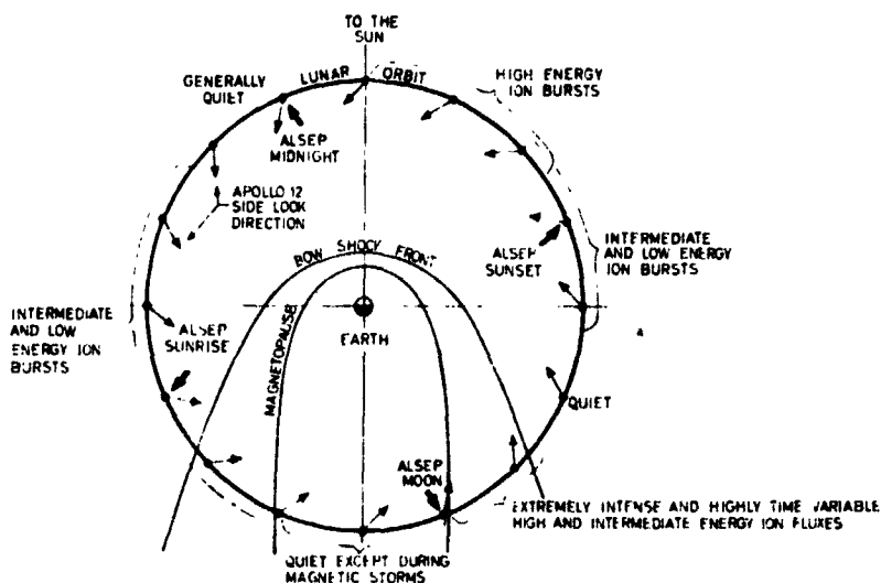
FIG. 3. Capaul summary of the location of diurnal phenomena along the lunar orbit.
