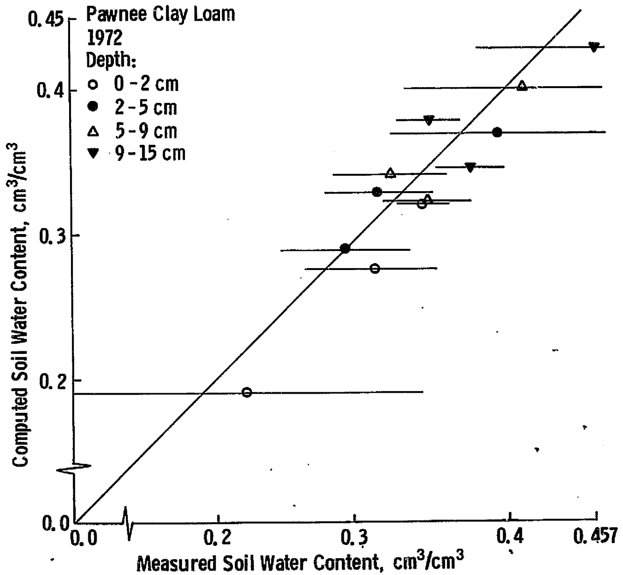
Figure 14. Comparison of computed and measured soil water contents. Data set TS4. Horizontal bars designate standard deviation.
