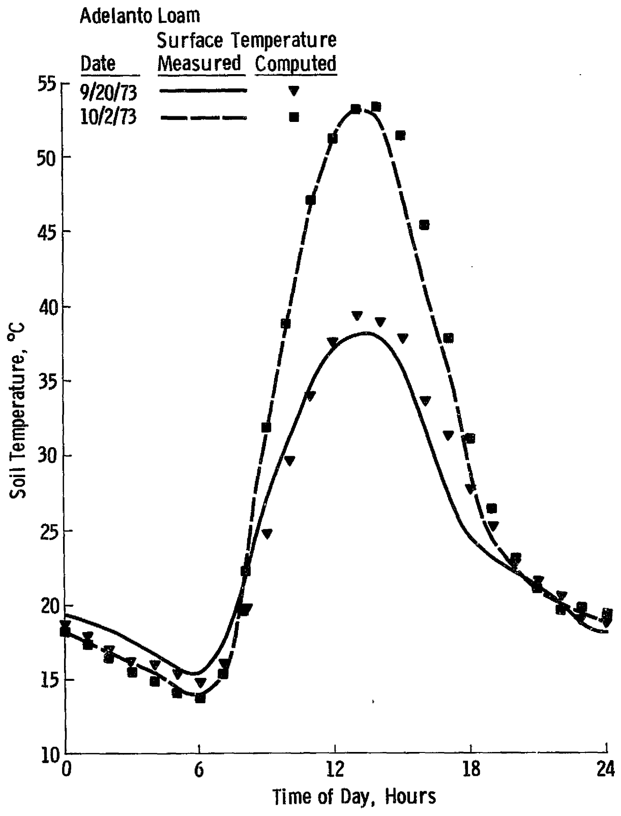
Figure 33. Comparison of computed and measured surface soil temperatures for dry and wet soil.
