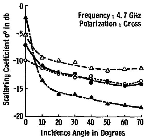
Figure 10c. Cross Polarization
