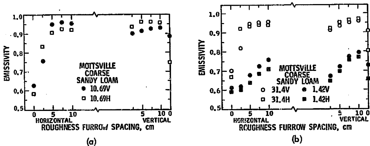
Figure 59. Moisture and roughness effects for sandy loam. From Blinn and Quade (1973).
