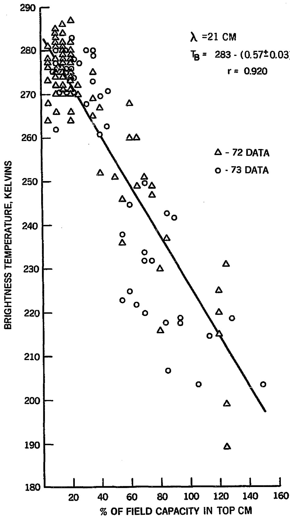
Figure 67. Plot of 21 cm brightness temperature versus soil moisture in top 1 cm expressed as a percent of field capacity. From Ulaby, et al. (1975).
