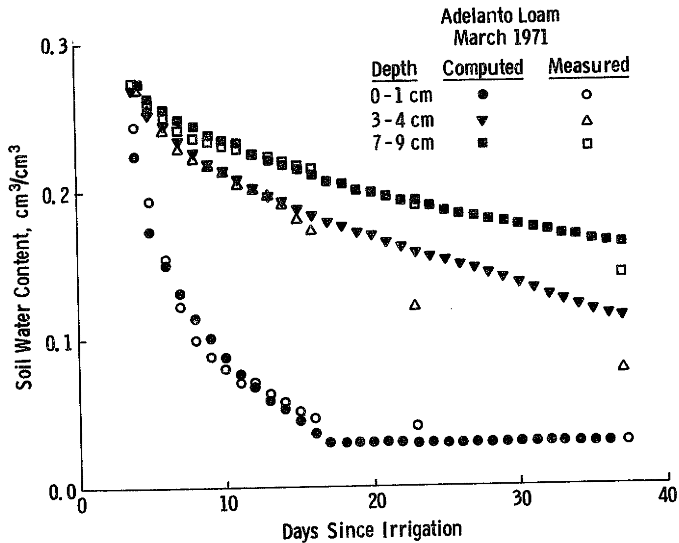
Figure 10. Comparison of computed and measured soil water contents for three depths as a function of time.
