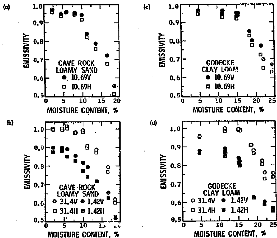
Figure 58. Moisture effects for loamy sand and clay loam. From Blinn and Quade (1973).
