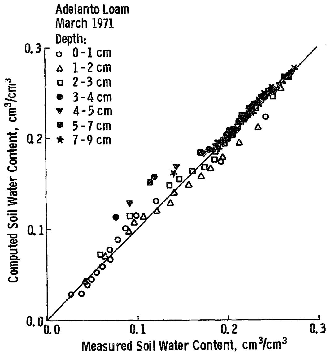
Figure 11. Comparison of computed and measured soil water contents. Data Set T51.
