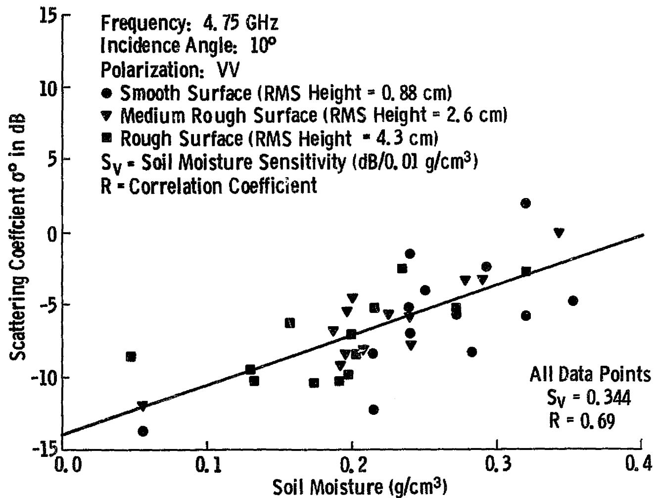
Figure 54. Scattering coefficient response as a function of soil moisture for three surface roughness profiles combined. From Ulaby, et al. (1975).
