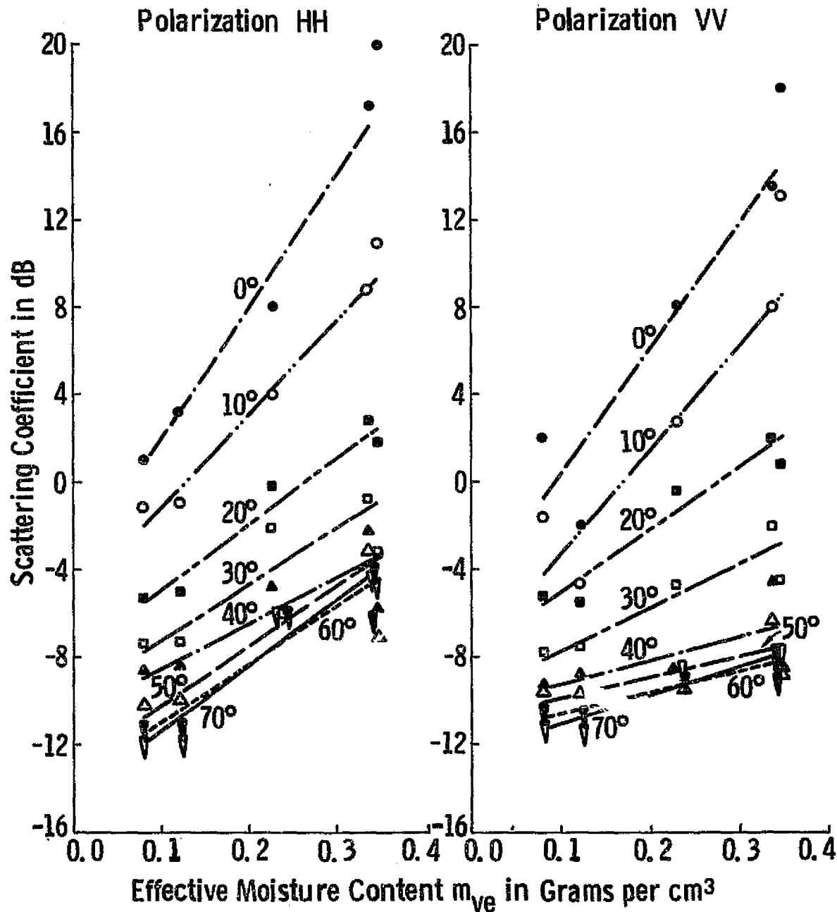
Figure 50. Scattering coefficient as a function of effective moisture content. Frequency is 4.7 GHz.
