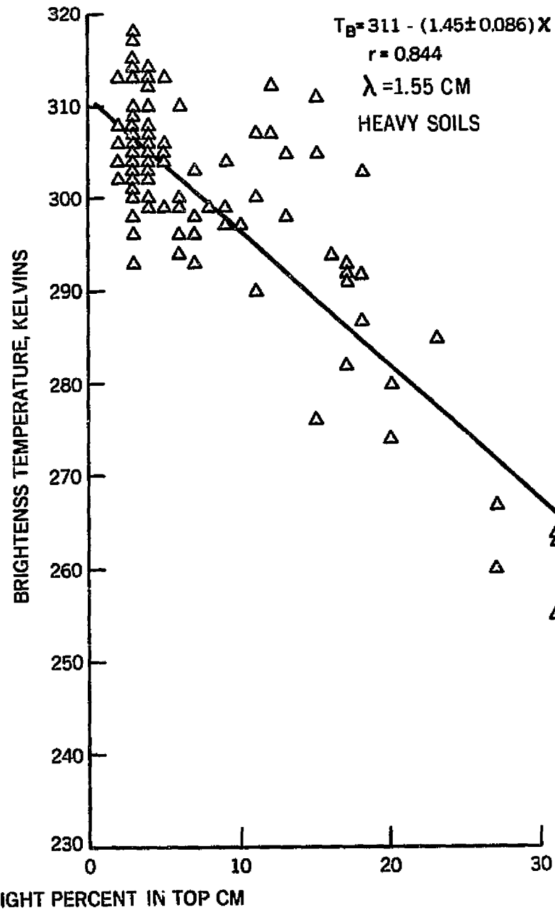
Figure 65. Plot of 1.55 cm brightness temperatures versus soil moisture for light soils (sandy loam and loam) and heavy soils (clay loam). From Ulaby, et al. (1975).
