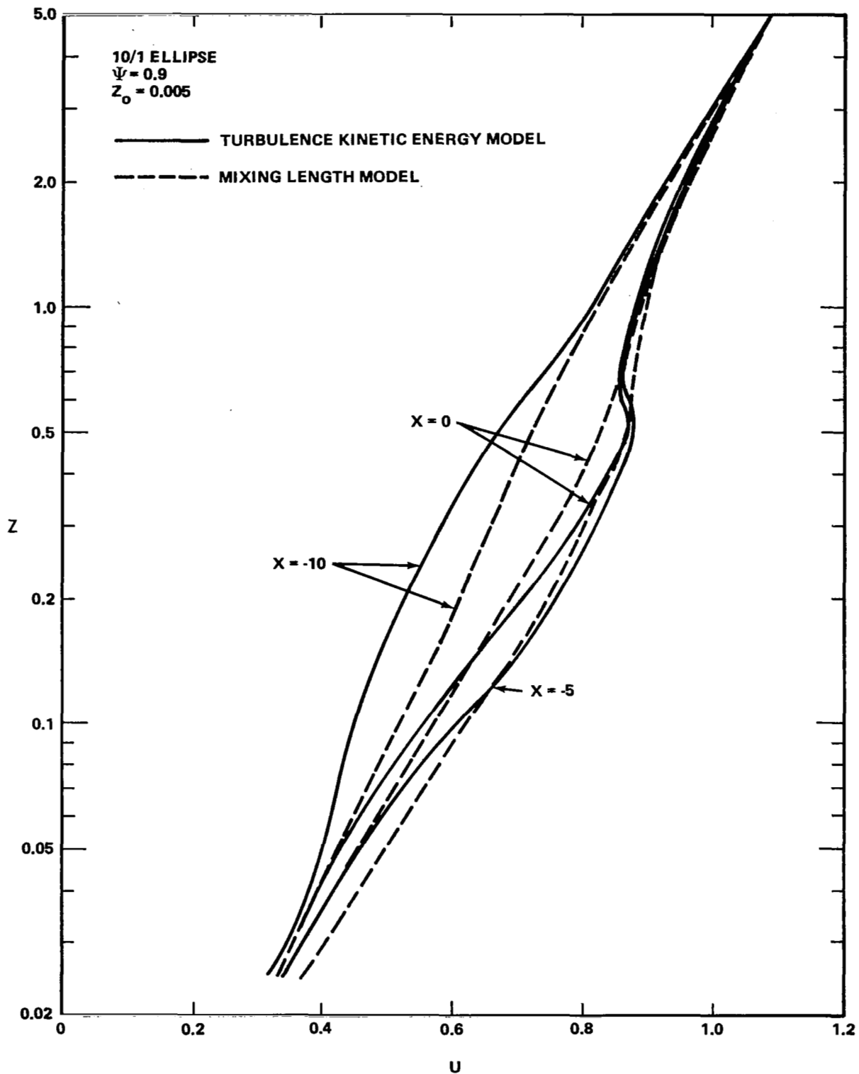
Figure 4. Velocity Distribution Over a 10/1 Ellipse for Turbulence Kinetic Energy and Mixing Length Models.
