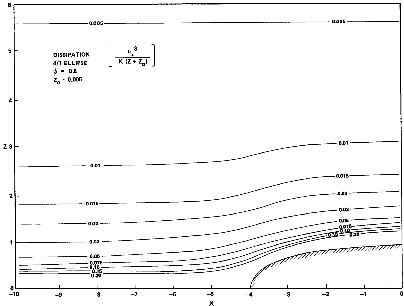
Figure 18. Distribution of Turbulence Kinetic Energy Dissipation Over
