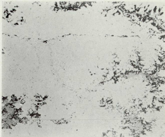
Figure C.6. Intrusive and extrusive igneous rocks (dark tones).
