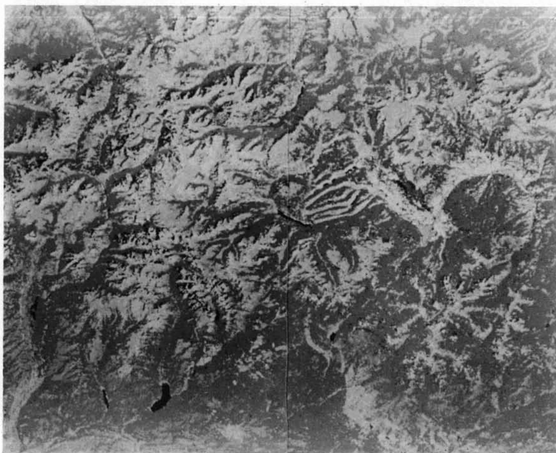
Figure A.17. Image from the digital display of the San Juan Mountain test site computer classification of level I. Black is water and terrain shadow, dark gray is coniferous forest, medium gray is deciduous forest, light gray is grass and cropland and white is barren.
