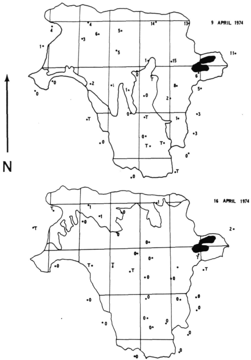
Figure 3. Snowcover maps for the Red River of the North above Emerson, Manitoba. The features in black are the Upper and Lower Red Lakes.
