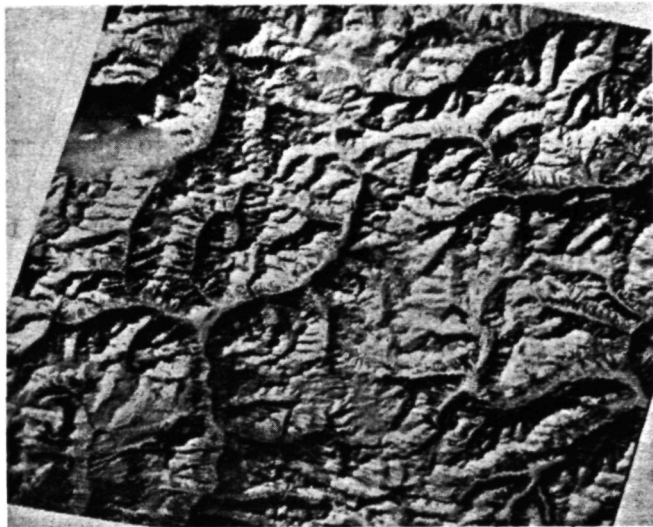
Figure 3. Digital Display Photograph of LANDSAT Frame 1119-17204, Band Five.
