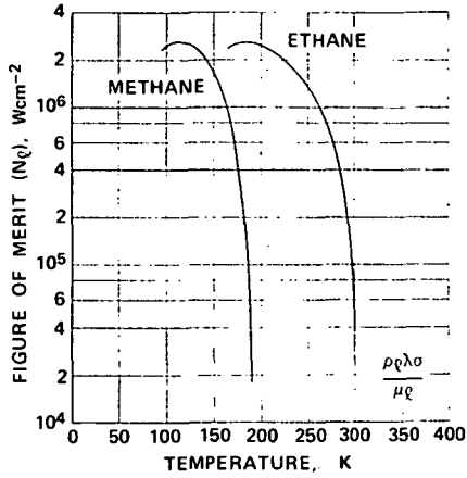
Fig. 1 Figure of merit of methane and ethane.
