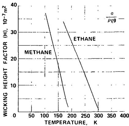
Fig. 2 Wicking height factor of methane and ethane.
