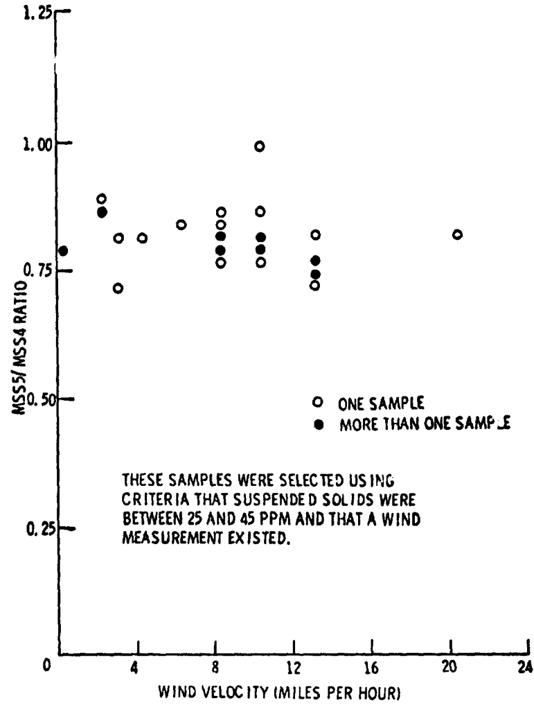
FIGURE 14. MSS 5/MSS 4 CCT RATIO VS. WIND VELOCITY FOR 35 SAMPLES TAKEN FROM 2 KANSAS RESERVOIRS OVER A 13 MONTH PERIOD.
